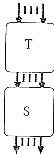
a product tangle
