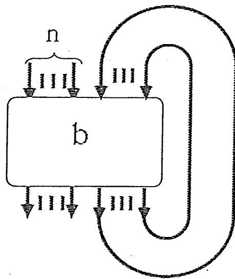
the n-closure of a braid b
