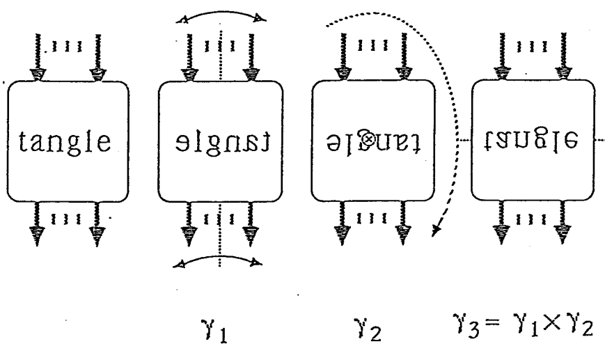
involutions of an n-tangle
