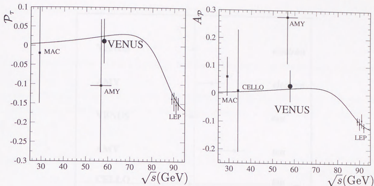
Figure 7.5: Measured values of P_\tau and A_P with those from other experiments. Solid line shows the Standard Model expectation.
