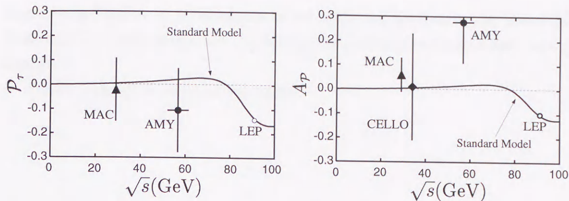
Figure 1.1: Results from other experiments on P_\tau (left) and A_P (right)[2, 3, 4, 5]. Solid line shows the Standard Model expectation. For the measurements at LEP, the values are averaged over four experiments and errors are close to the size of circles[5].
