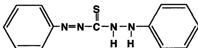
Dithizone
