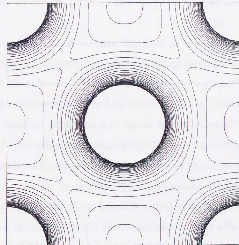
Figure 14: Electronic density maps on xy -plane of (a) BCT and (b) FCO. The contour values are given in 0.1 \text{ e}/\text{\AA}^3 and are drawn from 0.1 to 2.5 \text{ e}/\text{\AA}^3 .
