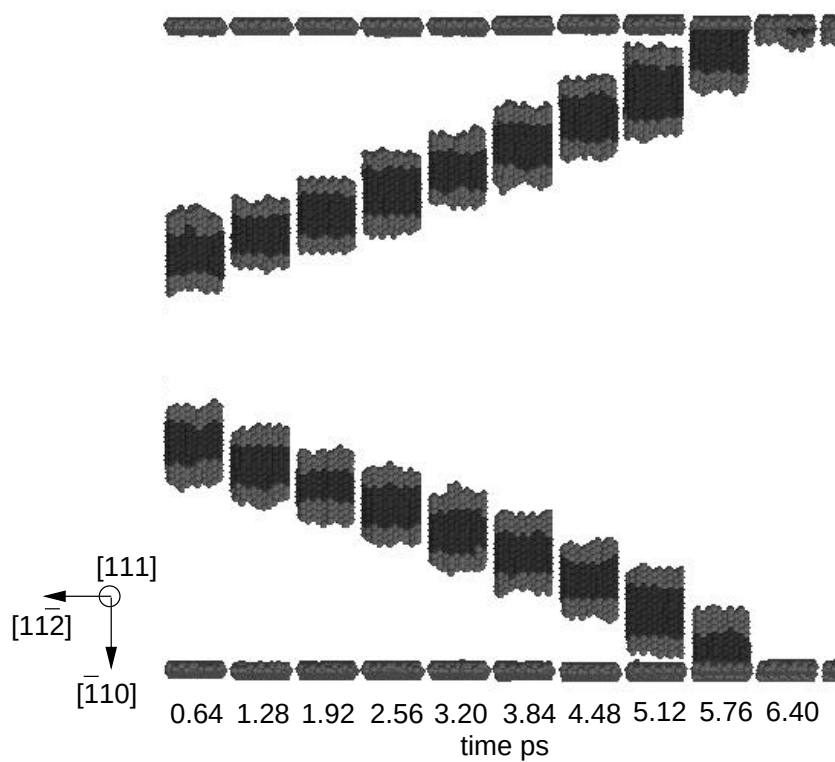
Fig. 3.4 Atomistic configuration of extended dislocations moving toward surface
