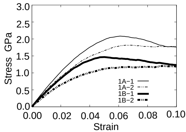
(b) x-tensile deformation
