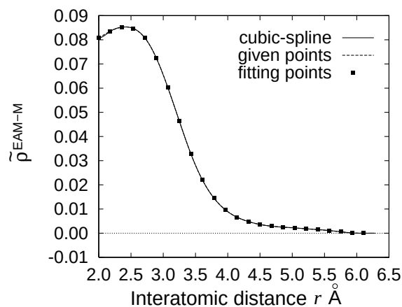
Fig. 2.4 Shape of the \tilde{\rho}^{\text{EAM-M}}(r)
