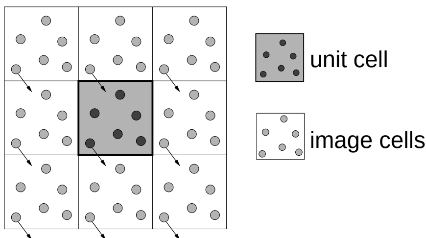
Fig. 2.1 Periodic boundary condition
