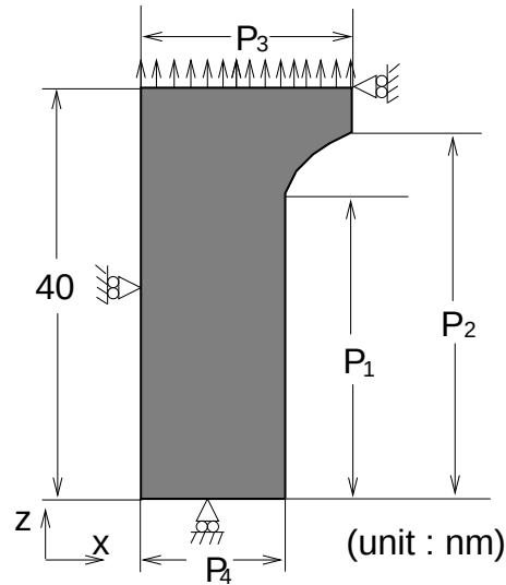
Fig. 5.1 Shape of a specimen
