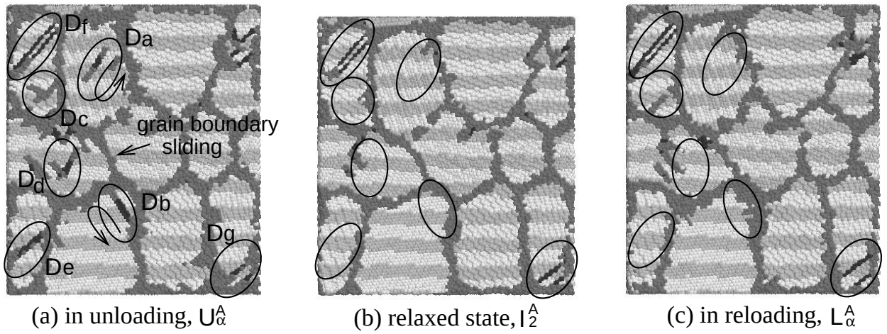
Fig. 4.36 Atomic configuration in a cross section of specimen 1A in the mechanically same states, U_{\alpha}^A and L_{\alpha}^A .
