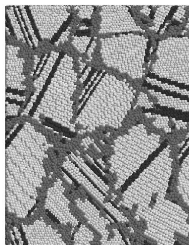
(f) Specimen 1B, \varepsilon=0.18
