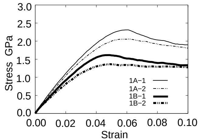
(a) z-tensile deformation
