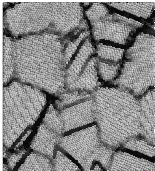
(a) Specimen 1A, \bar{\epsilon} : 0.00 \sim 0.08
