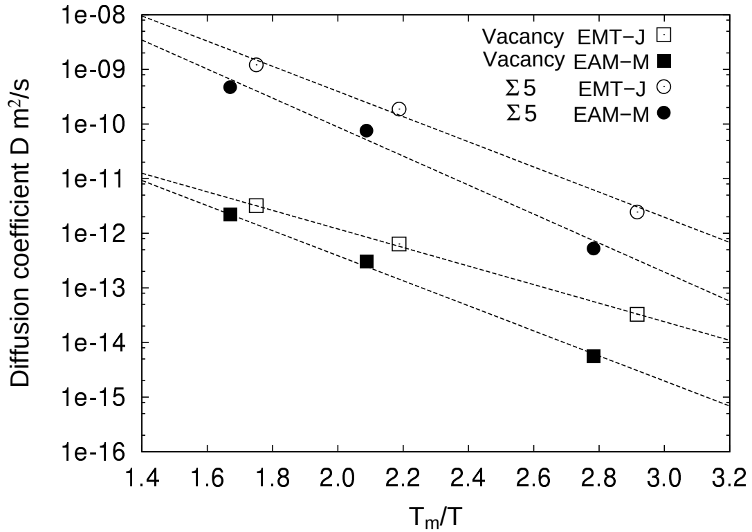
Fig. 3.14 Diffusion coefficient as a function of T_m/T
