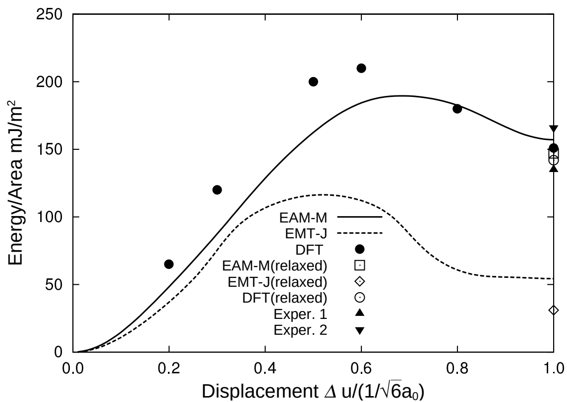
Fig. 3.1 GSF (Generalized Stacking Fault) energy curve
