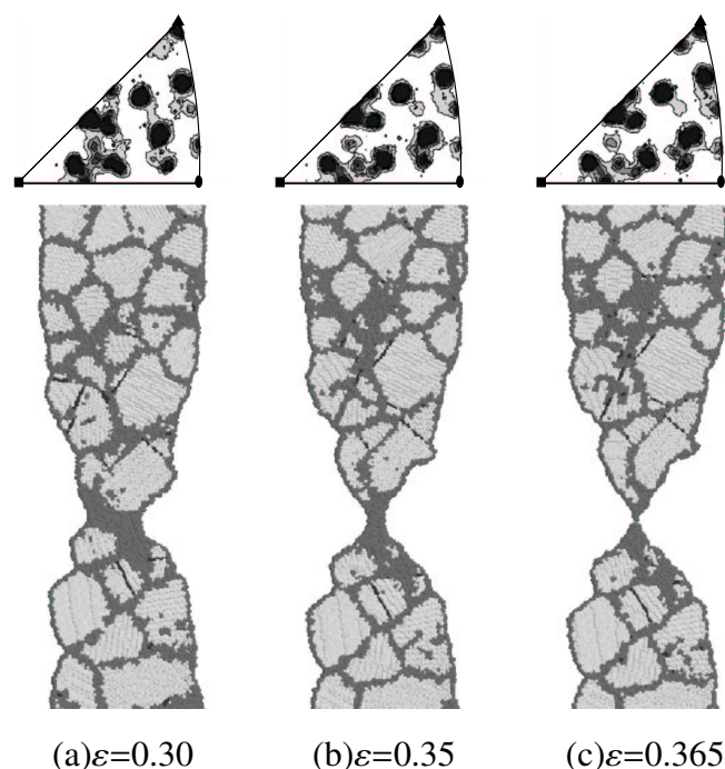
Fig. 5.15 Fracture of Specimen 4A at v=50\text{m/s}
