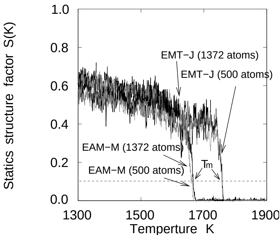
Fig. 3.11 Static structure factor as a function of temperature
