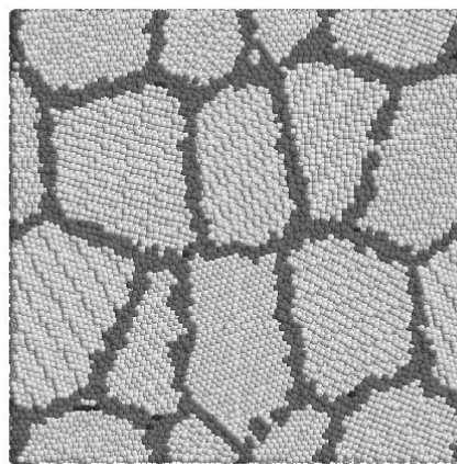
(b) Specimen 1B, \varepsilon=0.00
