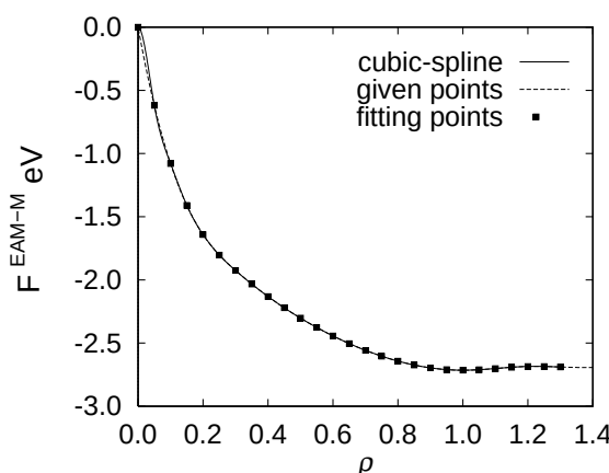
Fig. 2.5 Shape of the F^{\text{EAM-M}}(\rho)
