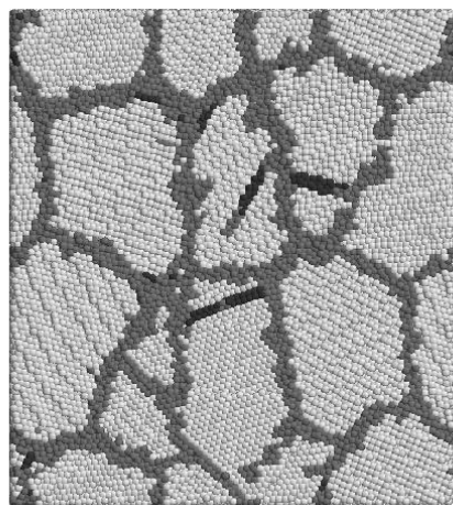
(c) Specimen 1A, \varepsilon=0.08
