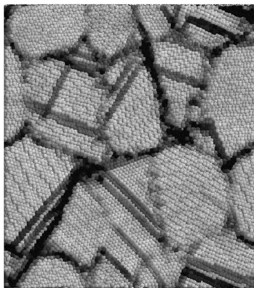
(b) Specimen 1B, \bar{\epsilon} : 0.00 \sim 0.08
