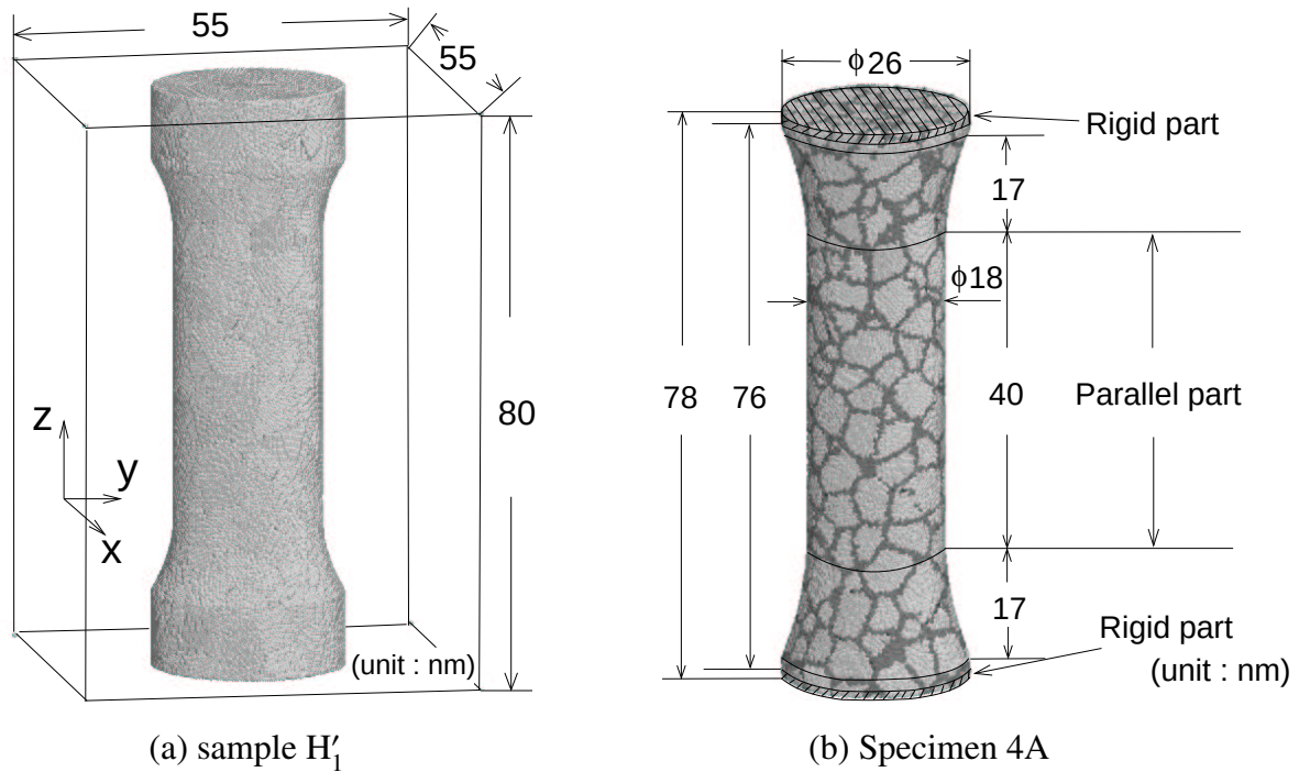
Fig. 5.3 Shape and dimensions of specimens
