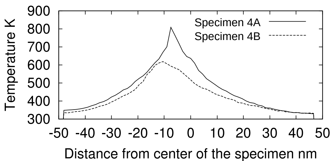
Fig. 5.19 Distribution of temperature of Specimen 4A and 4B in \varepsilon=0.35 , v=50\text{m/s}
