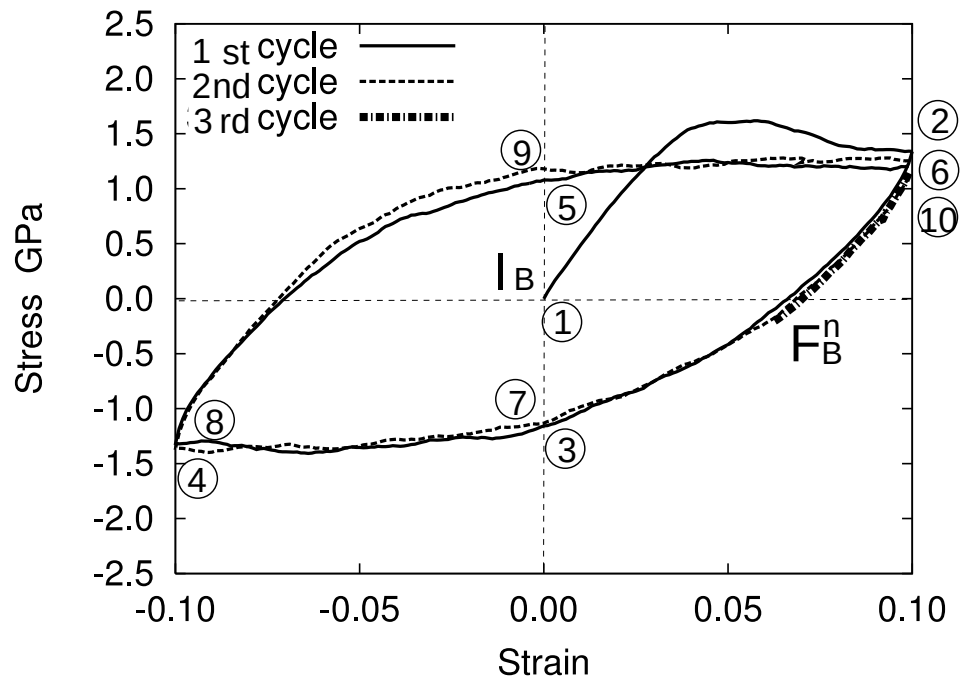
Fig. 4.60 Hysteresis loop of Specimen 1B
