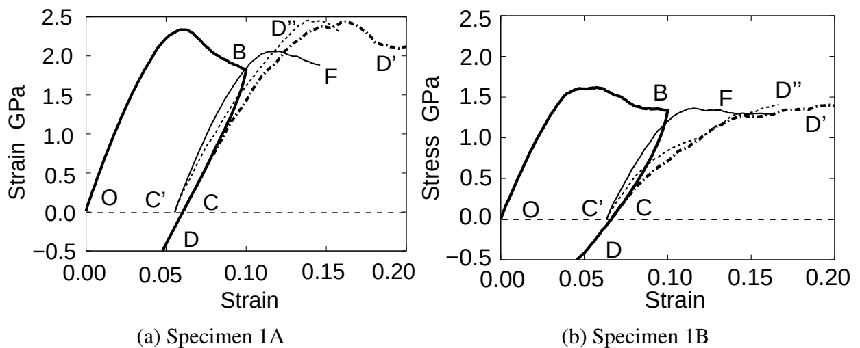
Fig. 4.64 Stress-strain curve
