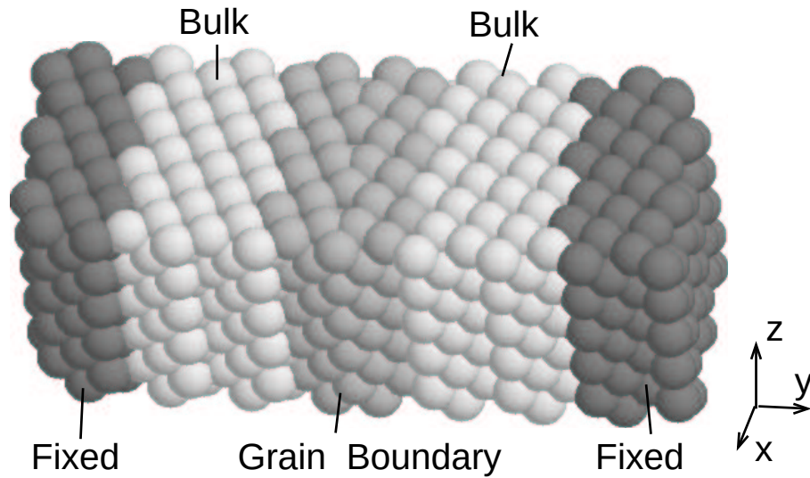
Fig. 3.10 Atomic arrangement of a model with \Sigma 5 tilt grain boundary
