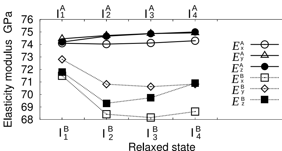
Fig. 4.39 Change of elasticity modulus E_x, E_y, E_z in each relaxed state.
