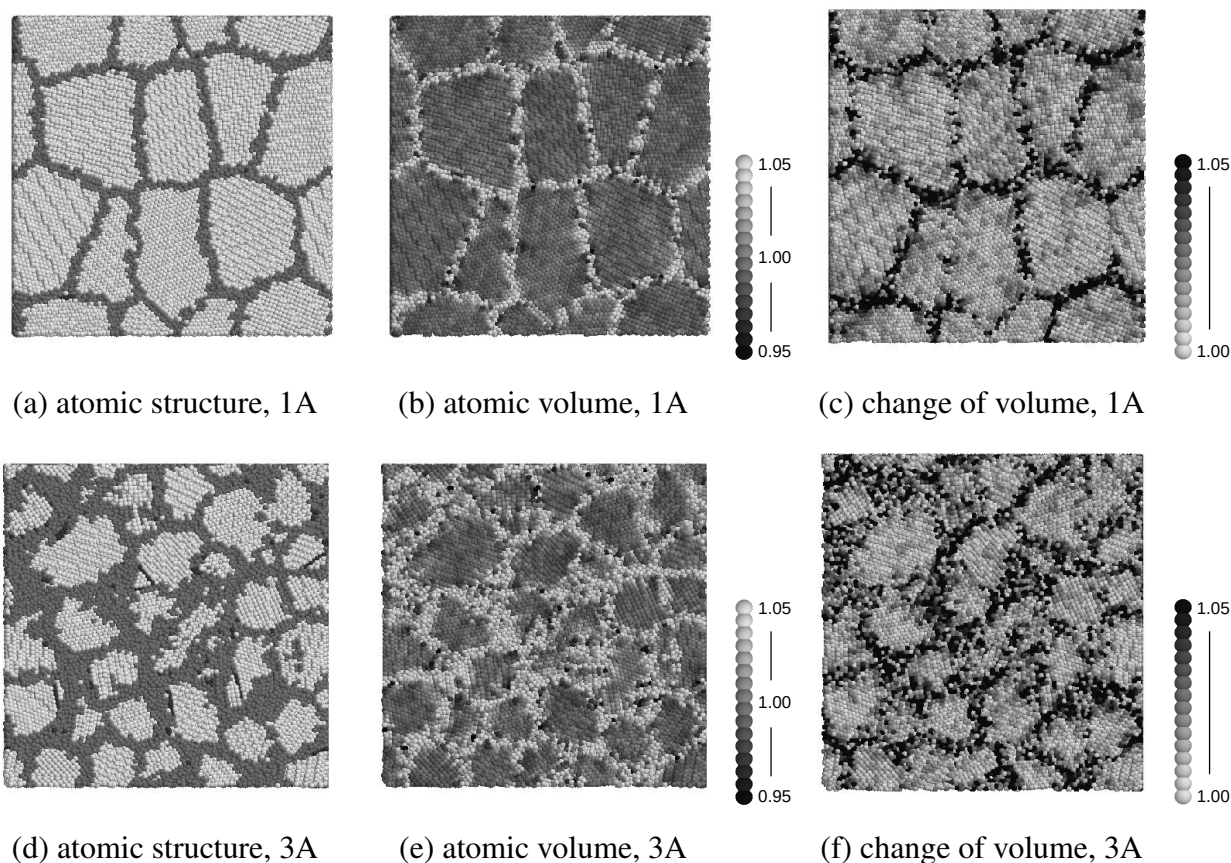
Fig. 4.17 Atomic arrangement on a cross section of specimen 1A and 3A on condition III, colored by (a), (d) atomic structure, (b), (e) atomic volume and (c), (f) absolute value of density change in \varepsilon from 0.00 to 0.04
