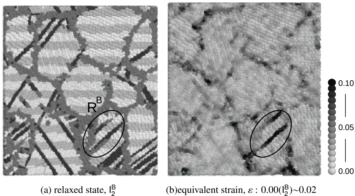
Fig. 4.41 Atomic arrangement of specimen 1B in the relaxed state l_2^B and opening of crystal slip in the early reloading process.
