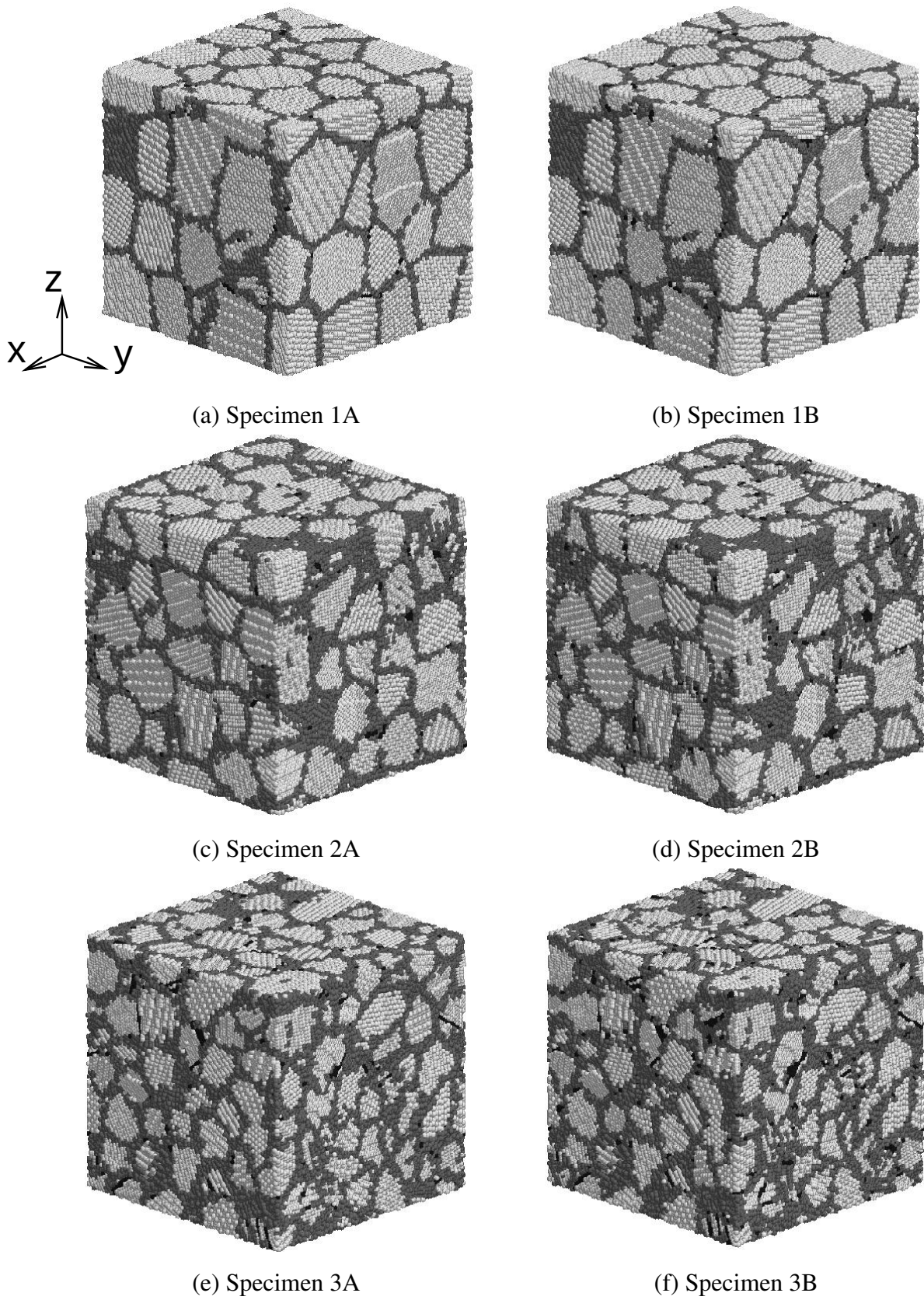
Fig. 4.3 Atomic configuration obtained by relaxation computation
