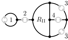
Fig. 5. A type \mathbf{D}_5 singular point: irreducible curves.
