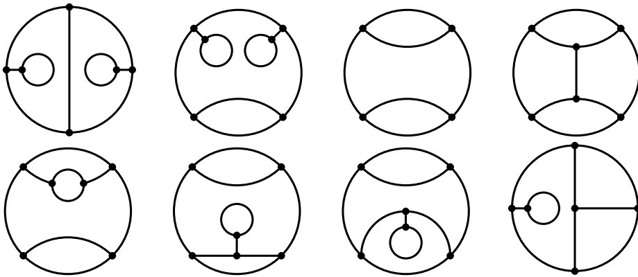
Fig. 6. A type \mathbf{D}_5 singular point: all curves.
