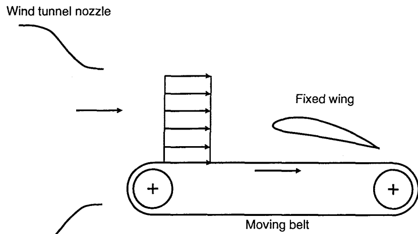
(a) Moving belt method.
