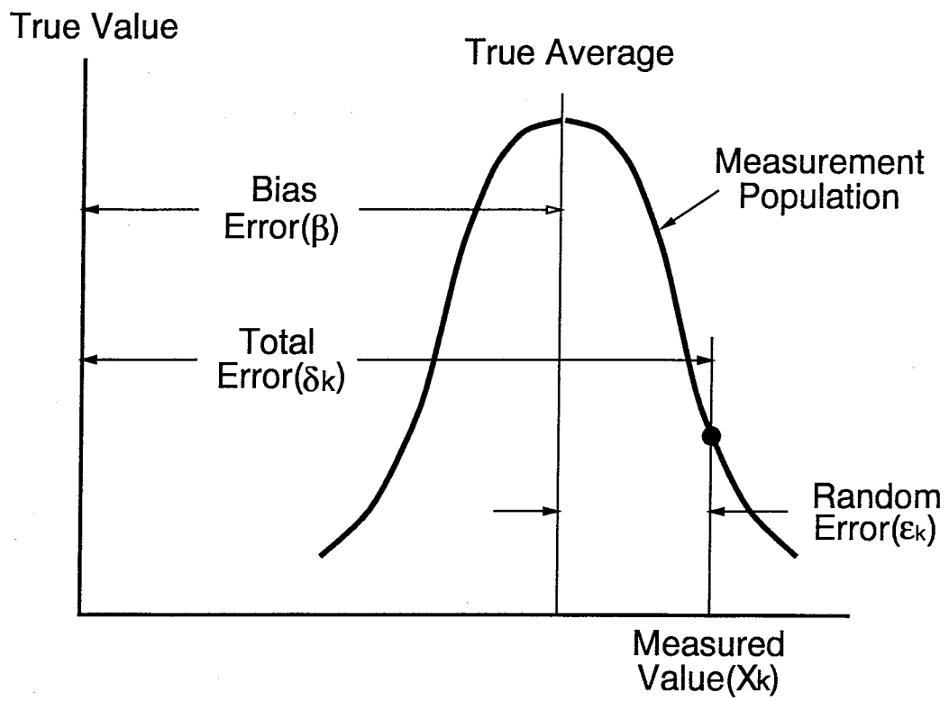
Fig. 3.22: Measurement errors.
