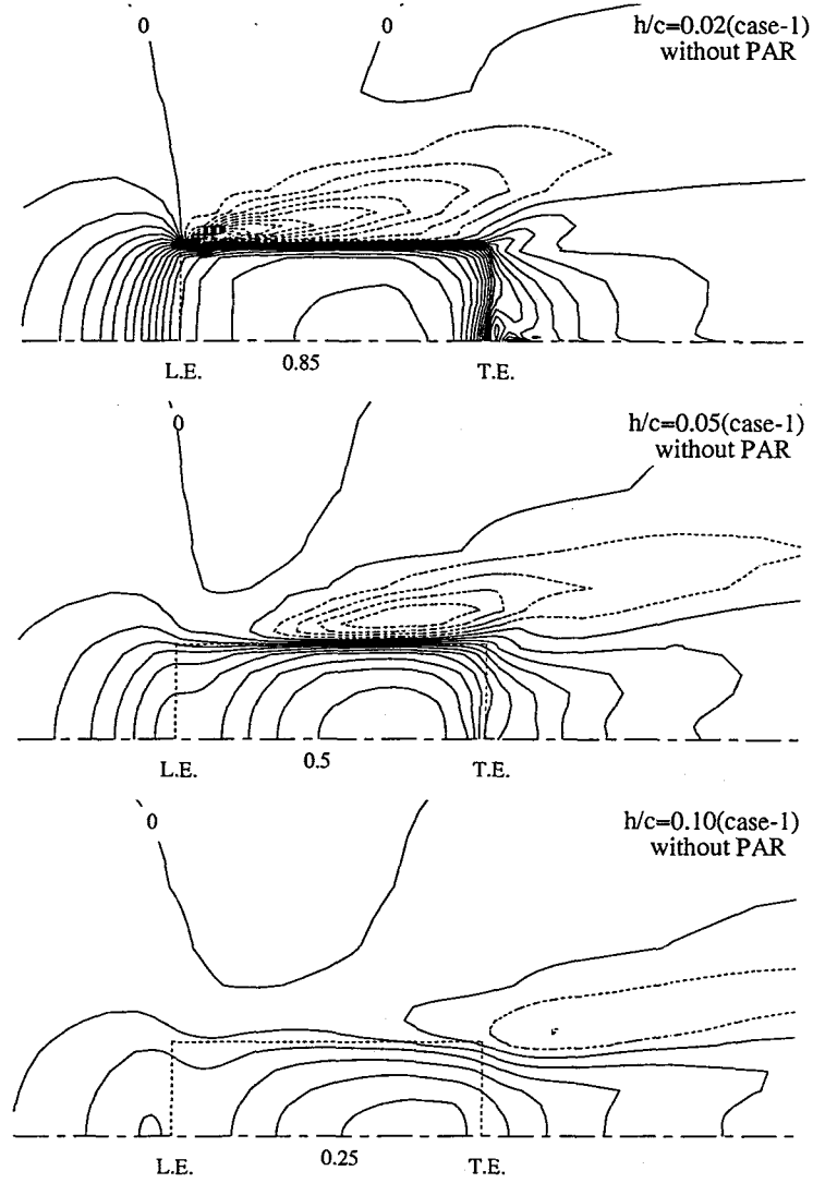
Fig. 5.23: Computed pressure distribution on ground without PAR thrust(Contour interval is 0.05q_\infty . Dotted lines show negative values).
