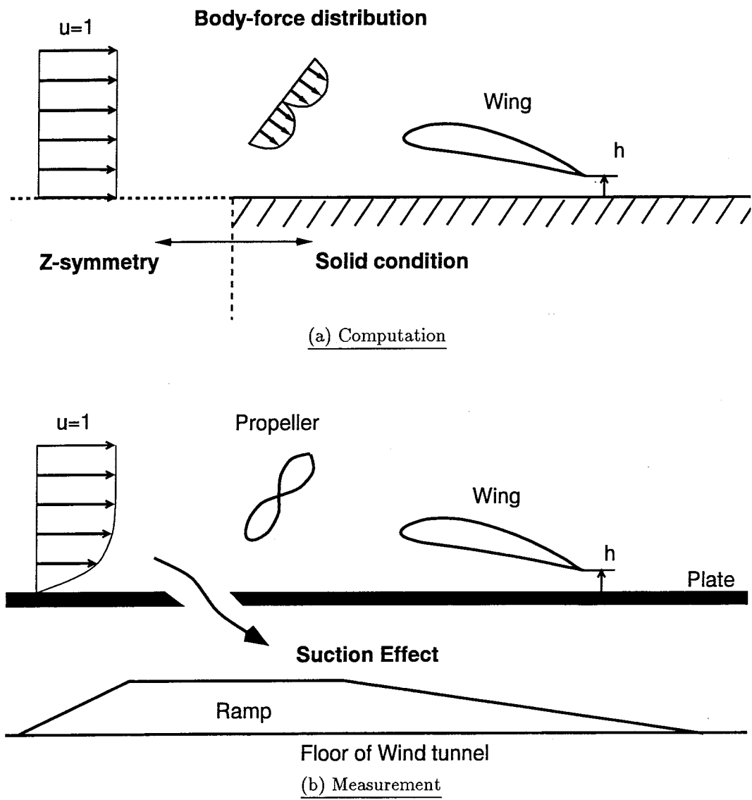
Fig. 4.3: Ground condition for a ground board method.
