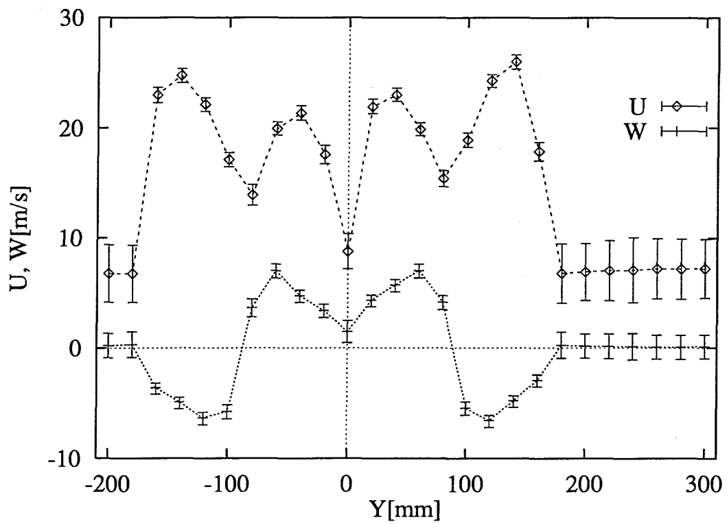
Fig. 3.8: Measured wake distributions behind a pair of propellers.
