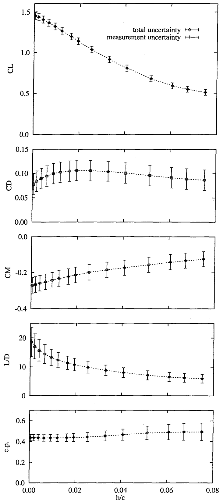
Fig. 3.9: Measured aerodynamic characteristics of a WIG at \alpha = 6^\circ by an image wing method.
