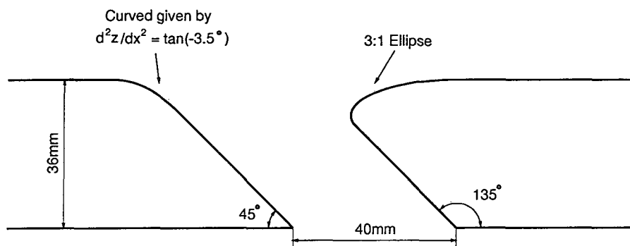
Fig. 3.4: Slot shapes.
