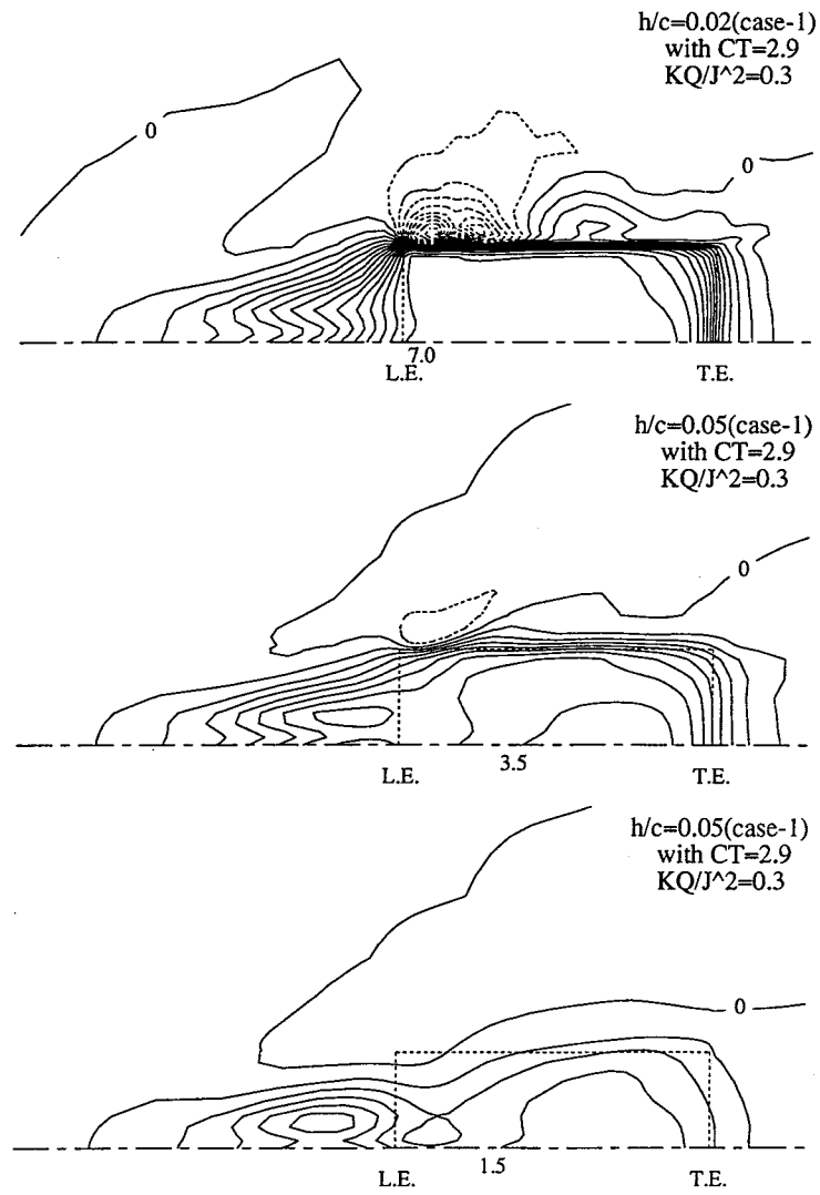
Fig. 5.30: Computed pressure distributions on ground with C_T = 2.9 and K_Q/J^2 = 0.3 (Contour interval is 0.5q_\infty . Dotted lines show negative values).
