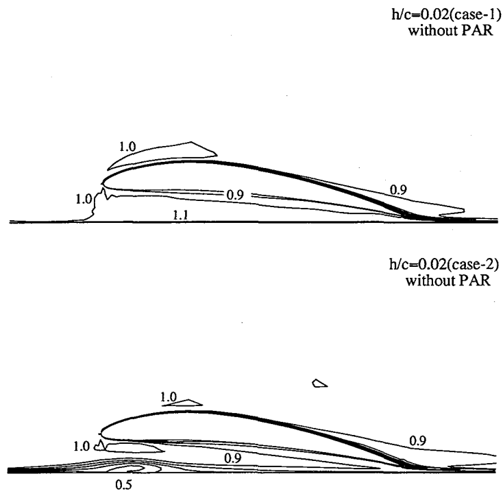
Fig. 5.3: Computed total pressure distributions at y/c = 0.188 without PAR thrust (Contour interval is 0.1q_\infty )
