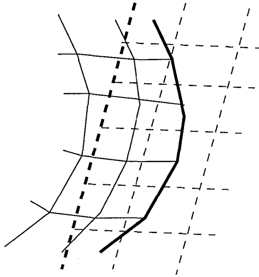
(a) Chimera grid
