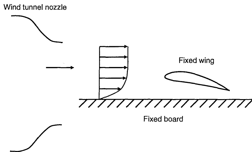
(c) Fixed ground board method.
