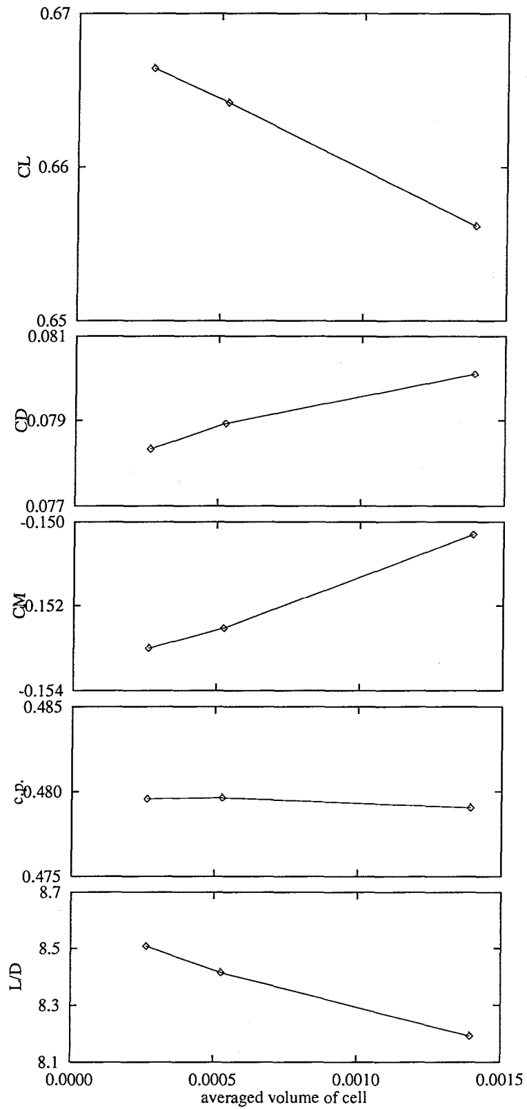
Fig. 4.4: Effect on aerodynamic characteristics of varing grid spacing
