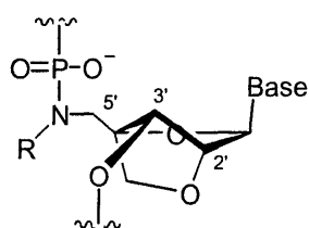
5'-amino-2',4'-BNA (R = H or Me) (N-type)
