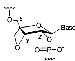
3',4'-BNA (S-type)
