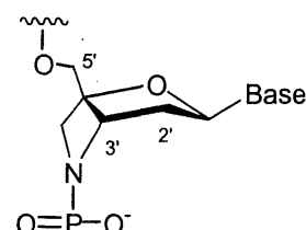
3'-amino-2'-deoxy-3',4'-BNA (S-type)
