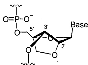
2',4'-BNA (N-type)
