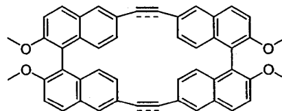
[2.2]binaphthylophane 2
