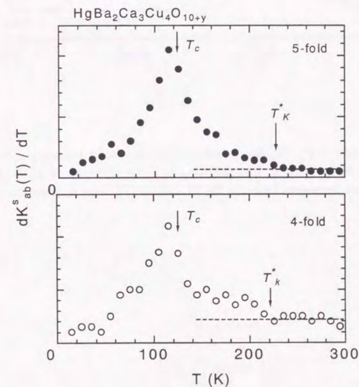
Figure 4.9: T -derivative change in K_{ab}^s(T) , dK_{ab}^s(T)/dT for 4-and 5-fold are plotted as a function of temperature.
