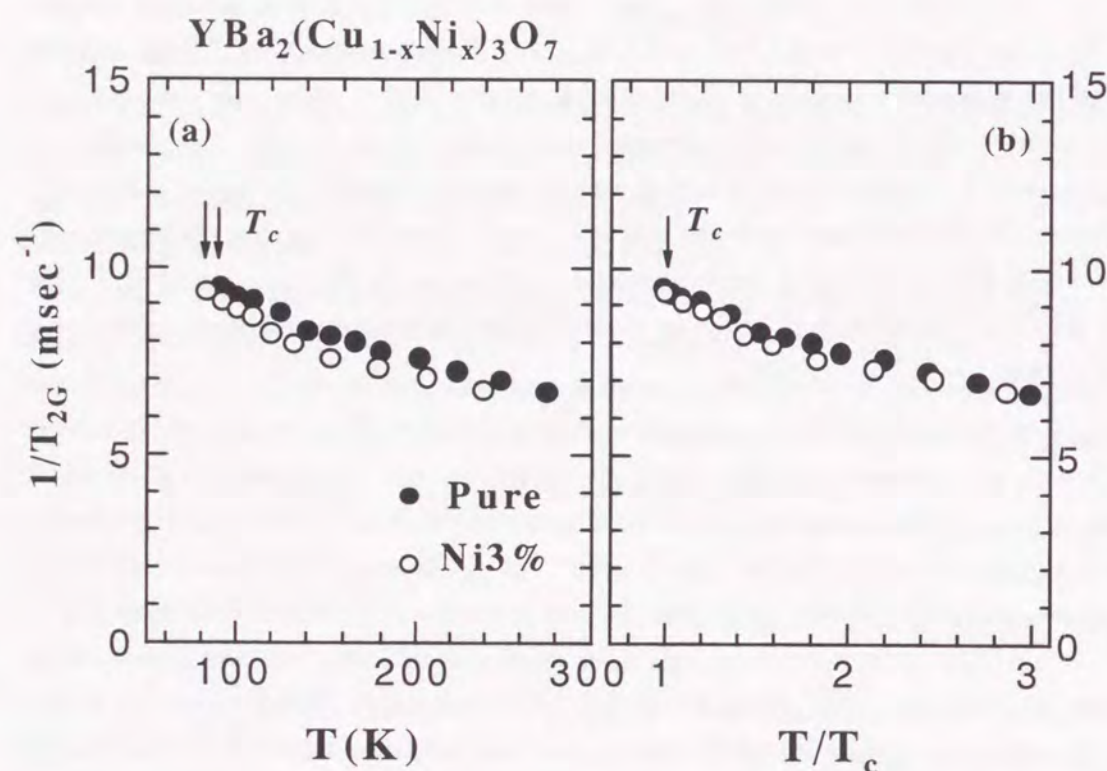
Figure 2.11: 1/T_{2G} in \text{YBa}_2(\text{Cu}_{1-x}\text{Ni}_x)_3\text{O}_7 are plotted against (a) T and (b) T/T_c(x) .
