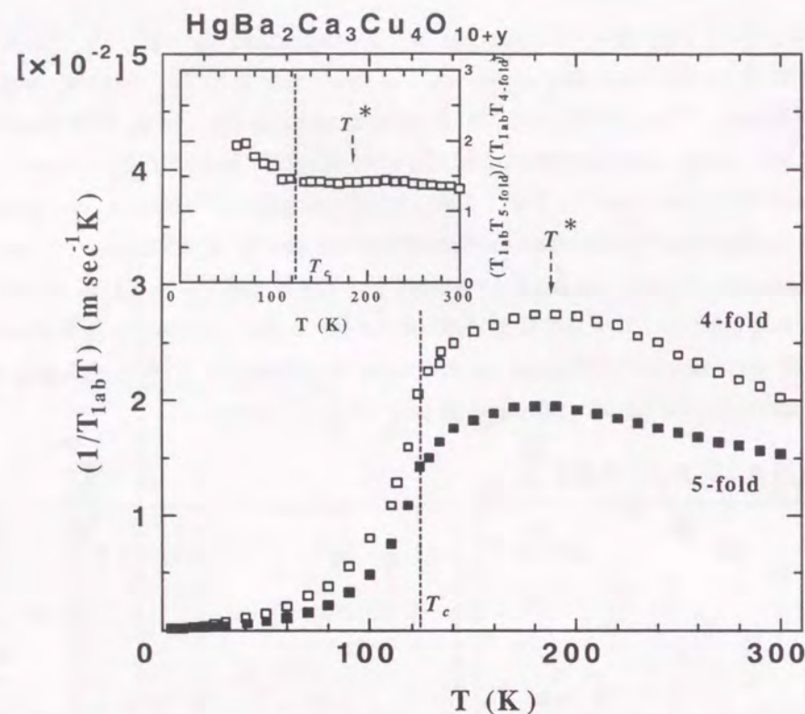
Figure 4.7: T dependence of ^{63}(1/T_1T)_{ab} for 4-fold and 5-fold. Inset shows the T dependence of the ratio of (T_1T_{5-fold})/(T_1T_{4-fold}) .
