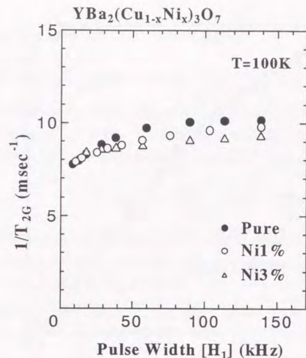
Figure 2.10: H_1 dependence of 1/T_{2G} in \text{YBa}_2(\text{Cu}_{1-x}\text{Ni}_x)_3\text{O}_7 at T = 100\text{K}
