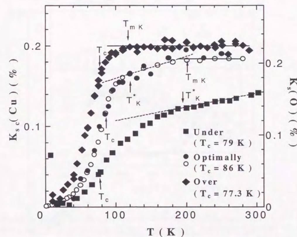
Figure 3.2: T -dependent spin part K_{sc}(\text{Cu}) in K_c in under-, optimally- and over-doped Bi2212. The T -dependent spin part K_s(\text{O}) in the ^{17}\text{O} Knight shift in optimally-doped Bi2212 reported by Takigawa et al. is also plotted by open circles ([25]). The anomalies at T_c , T_K^* and T_{mk} are indicated by arrows. (see text.)
