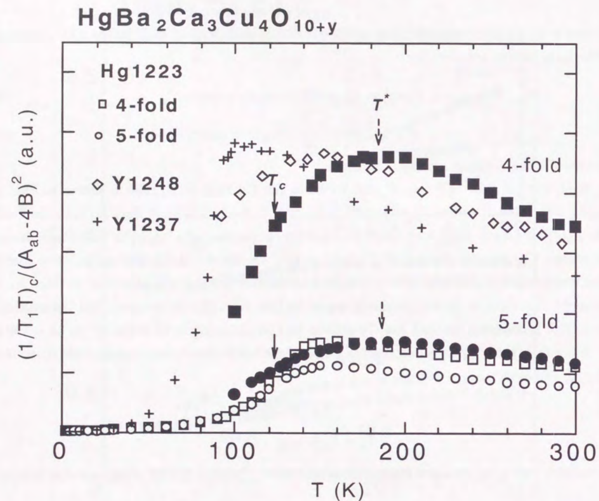
Figure 4.4: T dependence of ^{63}(1/T_1 T)_c / (A_{ab} - 4B)^2 ( \propto \alpha / \Gamma_Q ) along with the results of various high- T_c cuprates.
