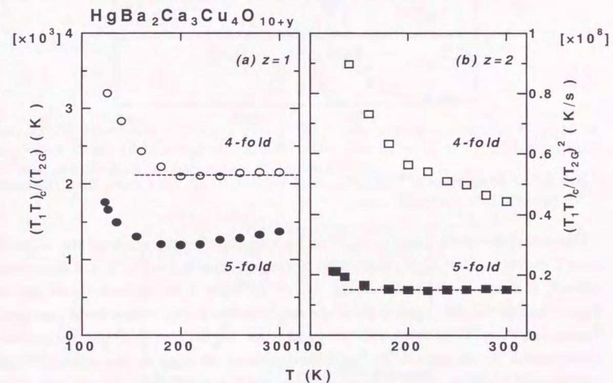
Figure 4.6: T dependence of (T_1T)_c/T_{2G} and (T_1T)_c/(T_{2G})^2 for both 4- and 5-fold.
