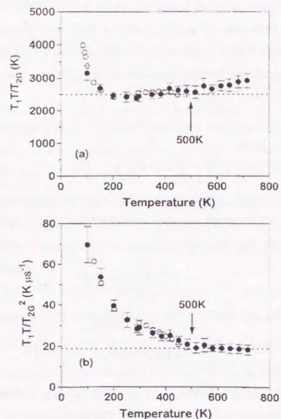
Figure 1.5: T_1T/T_{2G} and T_1T/T_{2G}^2 are plotted against T for \text{YBa}_2\text{Cu}_4\text{O}_8 ().
