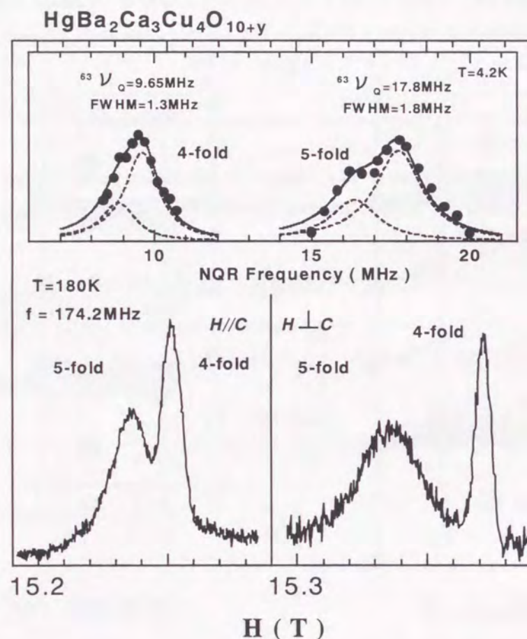
Figure 4.2: The ^{63}\text{Cu} NMR spectra for the central transition ( 1/2 \leftrightarrow -1/2 ) at f=174.2 MHz and T=180 K in the aligned powder with the c -axis parallel and perpendicular to the external magnetic field, H . The full-width at the half-maximum (FWHM) of the NMR spectra for c \parallel H are about \sim 85 Oe and \sim 155 Oe for 4- and 5-fold, respectively. Inset shows the Cu NQR spectra at T=4.2 K. \nu_Q 's and FWHM's are estimated to be 9.65 MHz and 1.3 MHz for 4-fold, and 17.8 MHz and 1.8 MHz for 5-fold, respectively.
