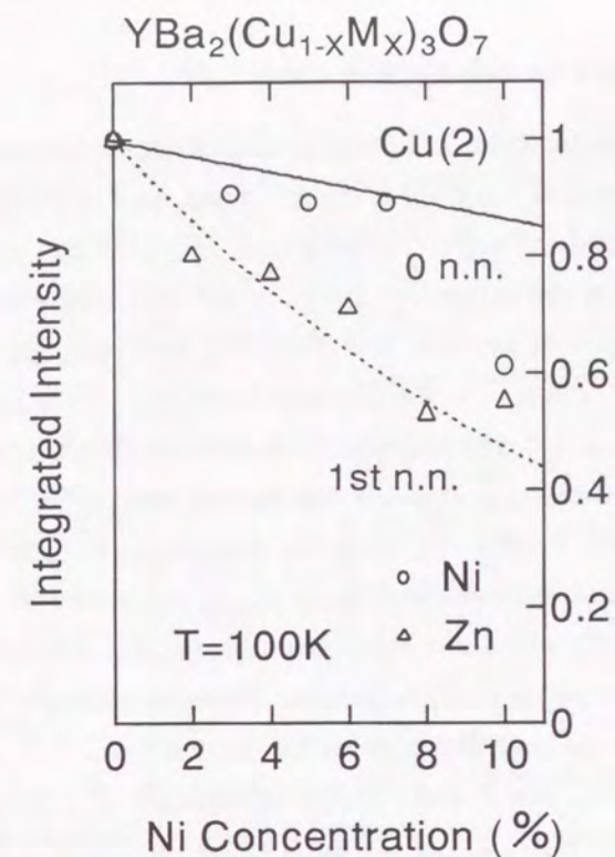
Figure 2.5: The Ni content dependence of the integrated intensity, I_{Ni}(x) for the Cu(2) NQR spectrum together with that for Zn-doped YBCO 7
