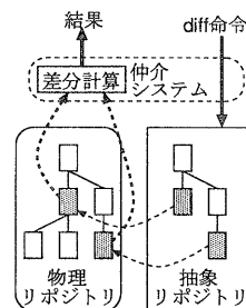
図 9: Diff の流れ
