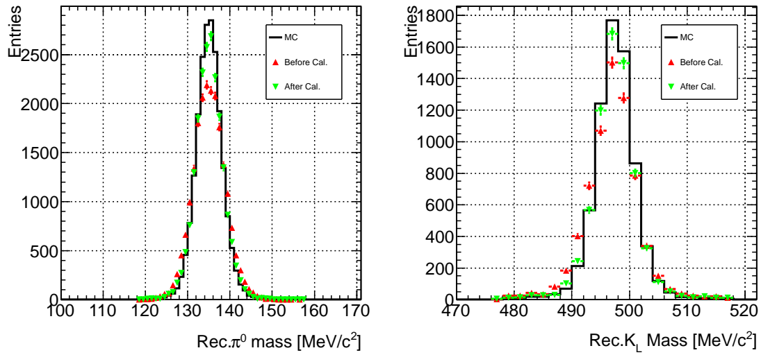
Figure 8.9: Reconstructed mass distribution of \pi^0 (left) and K_L (right). The distribution from the MC (black solid line), and beam data before (red triangle) and after (green triangle) applying calibration results are shown.
