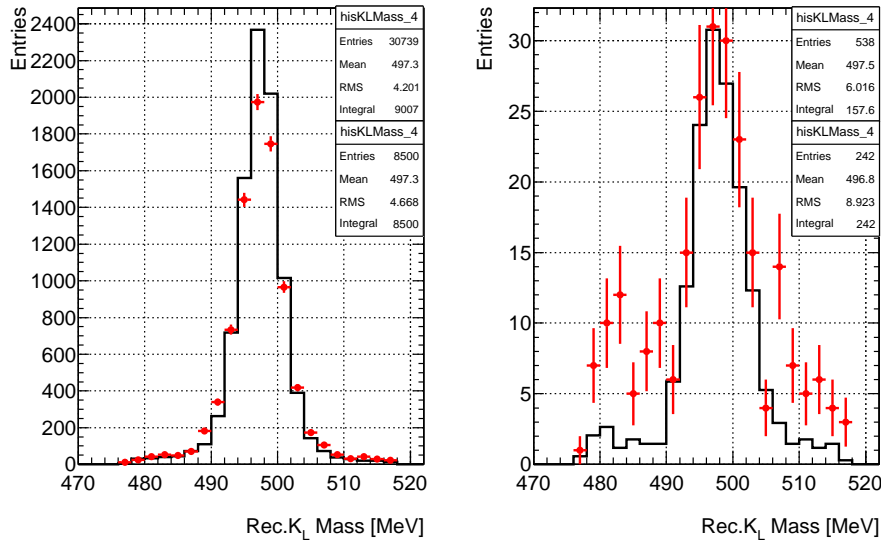
Figure 8.7: K_L mass distributions after cut. [Left]Reconstructed K_L s from 6\gamma events for MC data (black) and beam data (red). [Right]Reconstructed K_L s from 7 gamma events for Mc data (black) and beam data (red). The distributions from MC data is scaled by 0.293 in integral.
