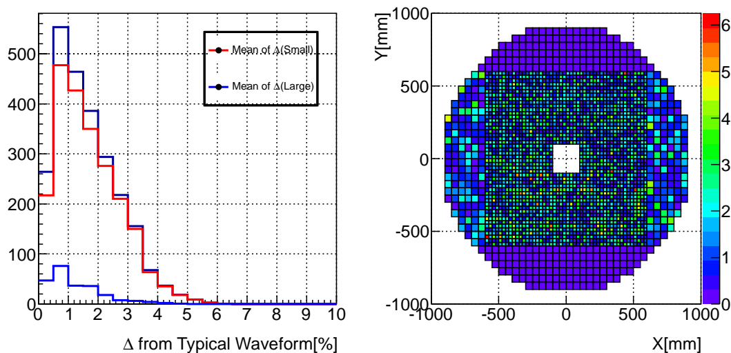
Figure 3.3: [Left]The distributions of \Delta . Red line shows the \Delta distribution of small modules, and blue line shows that of larger modules. [Right]XY distribution of \Delta . Two channels which had apparently different waveform are not included.
