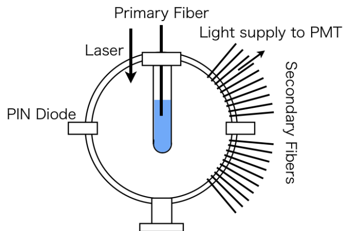
Figure 2.11: Schematic view of light distribution device of Laser gain monitoring system. The light is injected into scintillator placed at the center of light distribution device. The light from scintillator is distributed to PMTs through thin fibers pointing the center.
