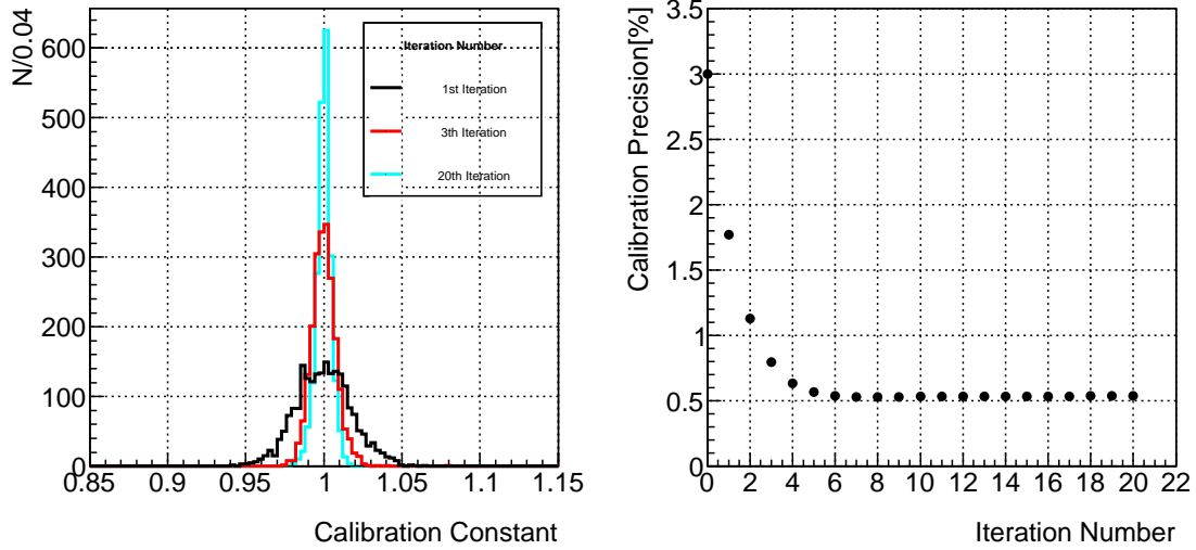
Figure 5.6: Effect of iteration on the final calibration accuracy. [Left]Distributions of the ratio between the calibration result and the ideal calibration constant is shown for different numbers of iterations (black: 1, red: 3, and blue 20). [Right]The relation of the calibration accuracy vs and number of iteration. After the 10th iteration, the RMS became stable at 0.54%. 2 \times 10^9 K_L \rightarrow 3\pi^0 events are used for calibration. The initial calibration constant variation was 3% in RMS.
