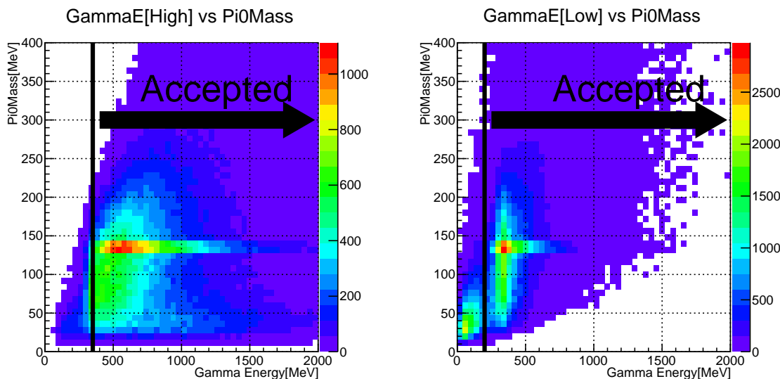
Figure 6.2: The distribution of the reconstructed \pi^0 mass and the gamma with larger energy (left) and smaller energy (right)
