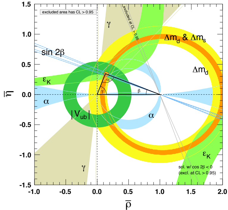
Figure 1.1: Current CKM unitarity triangle [5]
