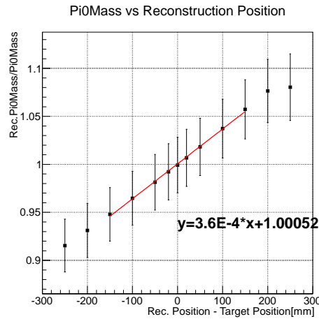
Figure 6.8: Effect of Al target position mis-measurement on \pi^0 mass peak value. The error var shows the width of the \pi^0 mass distribution.
