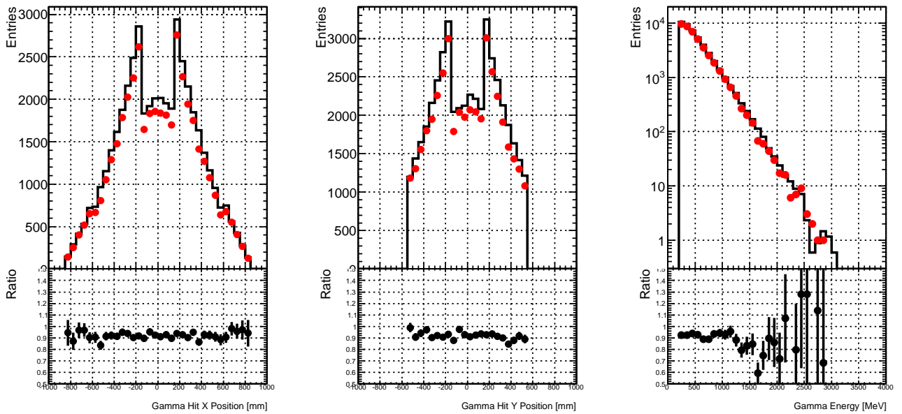
Figure 8.3: Gamma hit distributions in x (left) and y (center). The right plot shows the gamma energy. The black line and the red dots in the distributions shows the MC data and the beam data, respectively. The lower half shows the ratio between the two distributions (Beam/MC).
