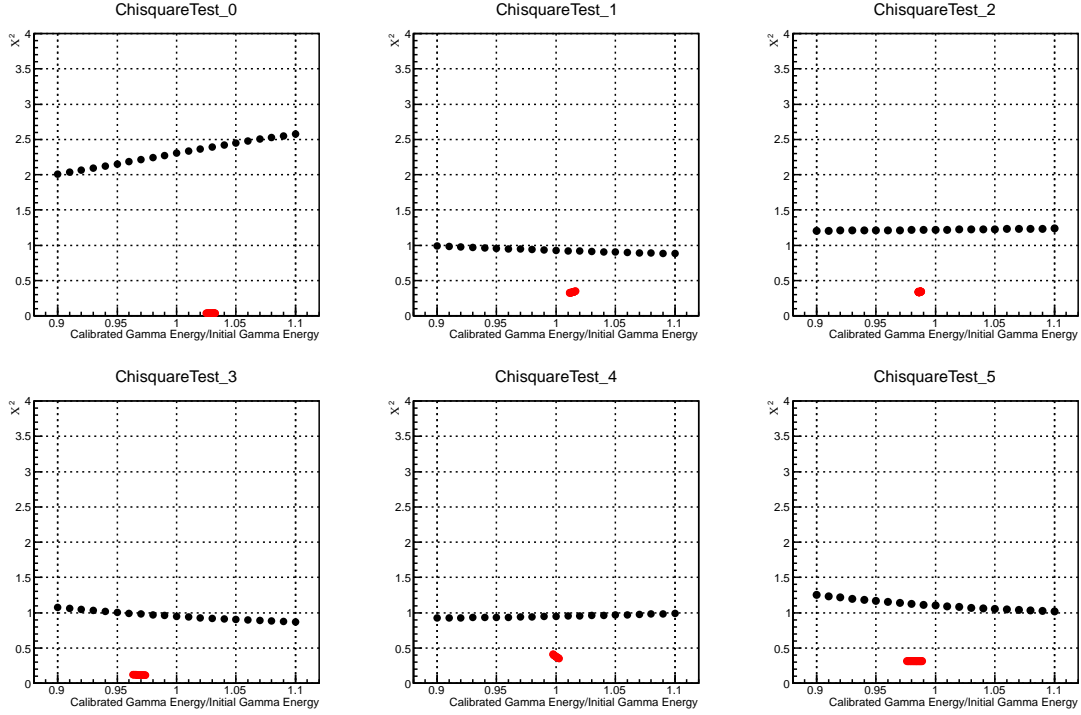
Figure 5.3: Calibration test result with a K_L \rightarrow 3\pi^0 event. Each plot corresponds to each gamma in the K_L \rightarrow 3\pi^0 decay. The black dots show the \chi^2 before fitting as a function of the ratio between a changed energy and an initial energy of the selected gamma. The red dots show the ratio between a fitted energy and correct energy of a selected gamma.
