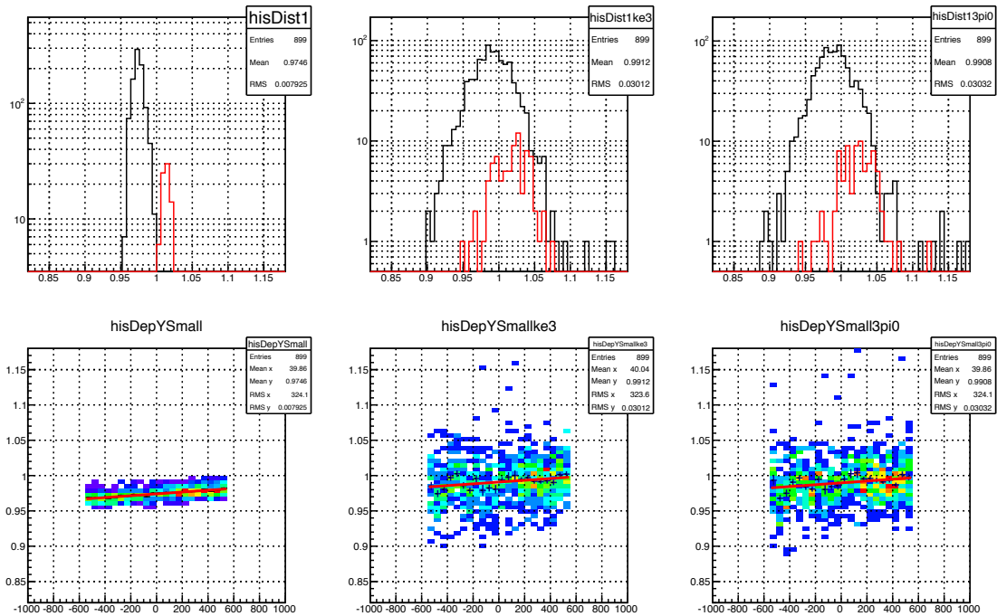
Figure 5.10: Comparison the calibration constant position distribution of small modules with other result. [Top, Left]The peak of MIP energy deposit distribution for small modules (black) and large modules (red). [Top, Middle]The distribution of the calibration constant from the Ke3 calibration method. All calibration constants are normalized by the initial calibration result. [Top, Right]The distribution of calibration constant from the relative calibration method. [Bottom, Left]The peak of MIP energy deposit distribution of modules vs module y position. [Bottom, Middle] The calibration constant from Ke3 calibration method vs module y position. [Bottom, Right]The calibration constant from relative calibration method vs module y position.
