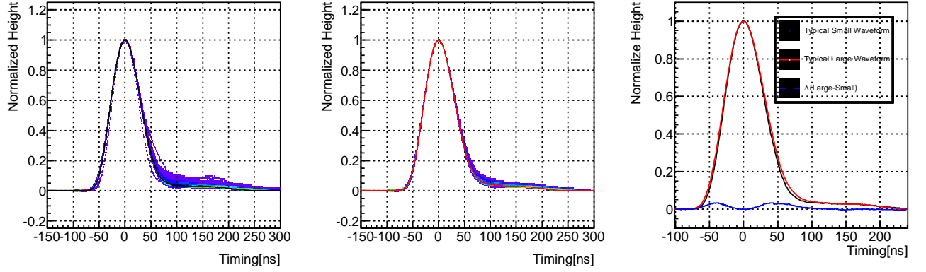
Figure 3.2: The templates of small modules (left) and large modules (middle) are shown. In the right figure, the typical waveform of small modules (left, black line) and large modules (center, red line) and their difference (right, blue line) are shown. The difference of templates widens at the tail region (50 ns in the figure). The waveform of large module is slightly wider than small module.
