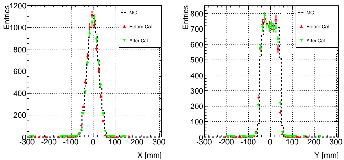
Figure 8.10: Distributions of x_{c.o.e.} (left) and y_{c.o.e.} (right). The distribution from the MC (black dashed line), and beam data before (red triangle) and after (green triangle) applying calibration result are shown.
