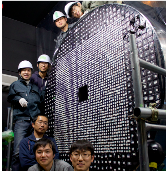
Figure 1.7: Front view of the calorimeter. In the center of calorimeter, there are beam exist.
