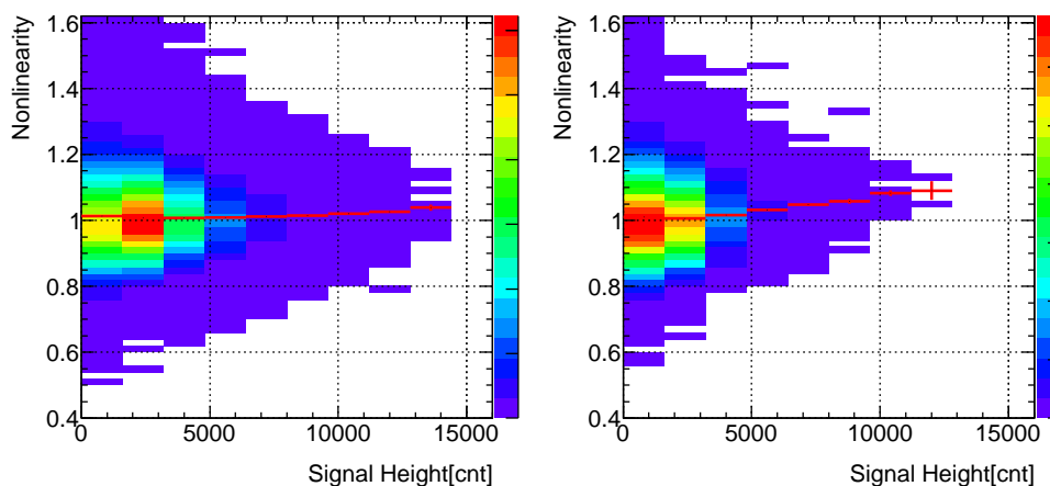
Figure 7.4: The relation of the \delta(h) and the max pulse height with 2% nonlinearity (left) and 5% nonlinearity (right) assumed for all modules. Red line shows the average nonlinearity by pulse height.
