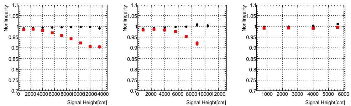
Figure 7.7: Derived nonlinearity from 3\pi^0 calibration method for common small modules (left), specific small modules (middle), and large modules (right). Red dots represent nonlinearity from the beam data, and black dots represent nonlinearity from the MC.
