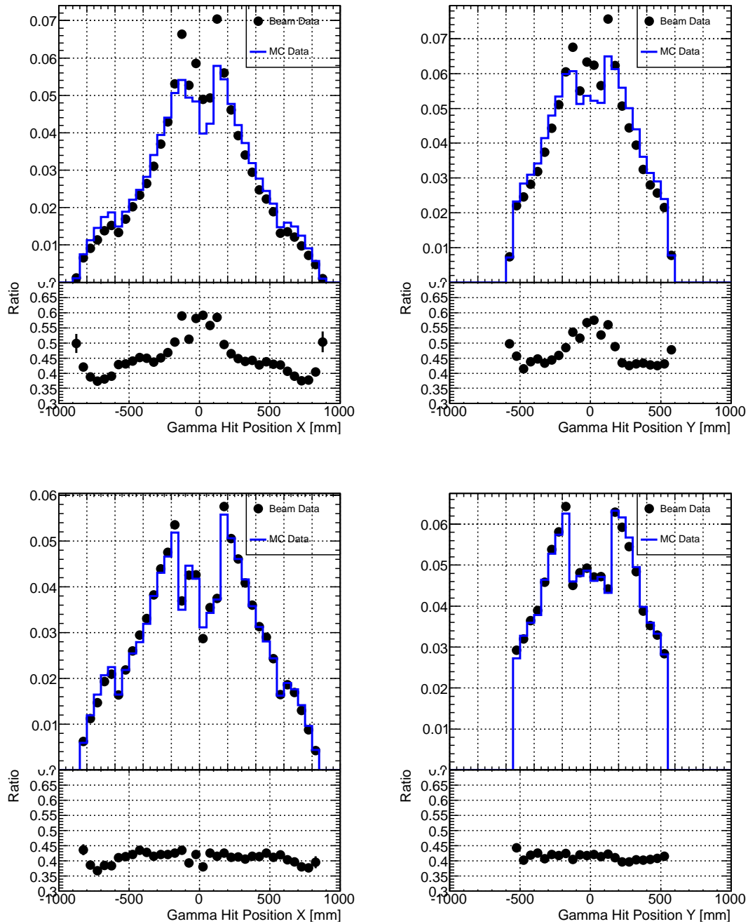
Figure 6.4: Gamma hit position of Al target run data. [Top] x (left) and y (right) distributions before applying cuts. [Bottom] x (left) and y (right) distributions after applying cuts. Black dots show beam event data, and blue lines shows MC data. The dots shown in the lower half shows the ratio between beam event data and MC data.
