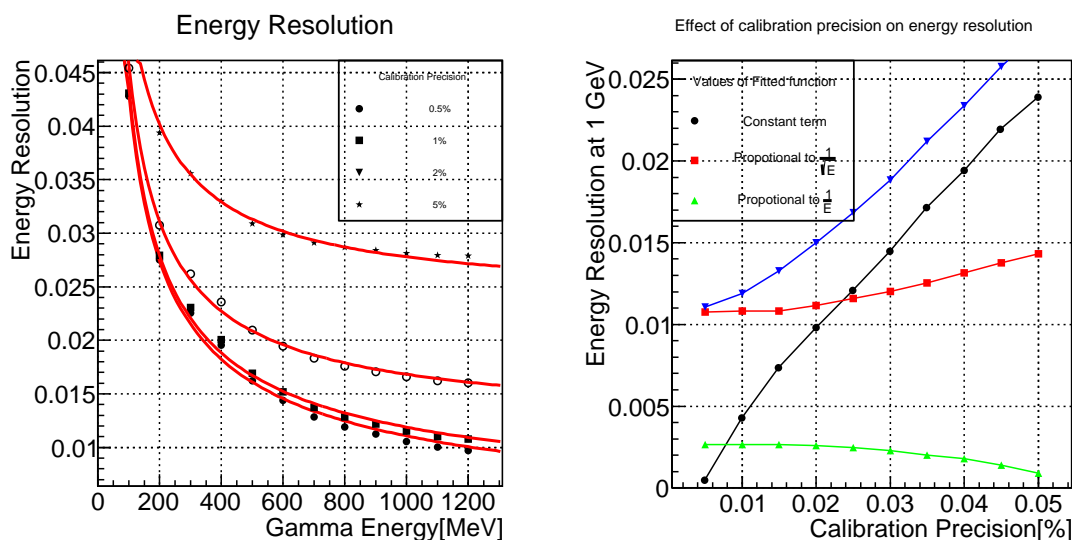
Figure 8.8: Effect of the calibration precision on the gamma energy resolution in the MC. The energy resolutions for 0.5%, 1%, 2%, and 5% of calibration precision for various gamma energies are shown on the left. The energy dependence of the energy resolution was fitted by a function, f(E) = p_0 \oplus \frac{p_1}{\sqrt{E}} \oplus \frac{p_2}{E} . The energy resolution at 1GeV for various calibration precision and the contributions of the fitting parameters, p_0 (black line), p_1 (red line), p_2 (green line), on the energy resolution are shown on the right. The constant term ( p_0 ) was linear with the calibration precision.
