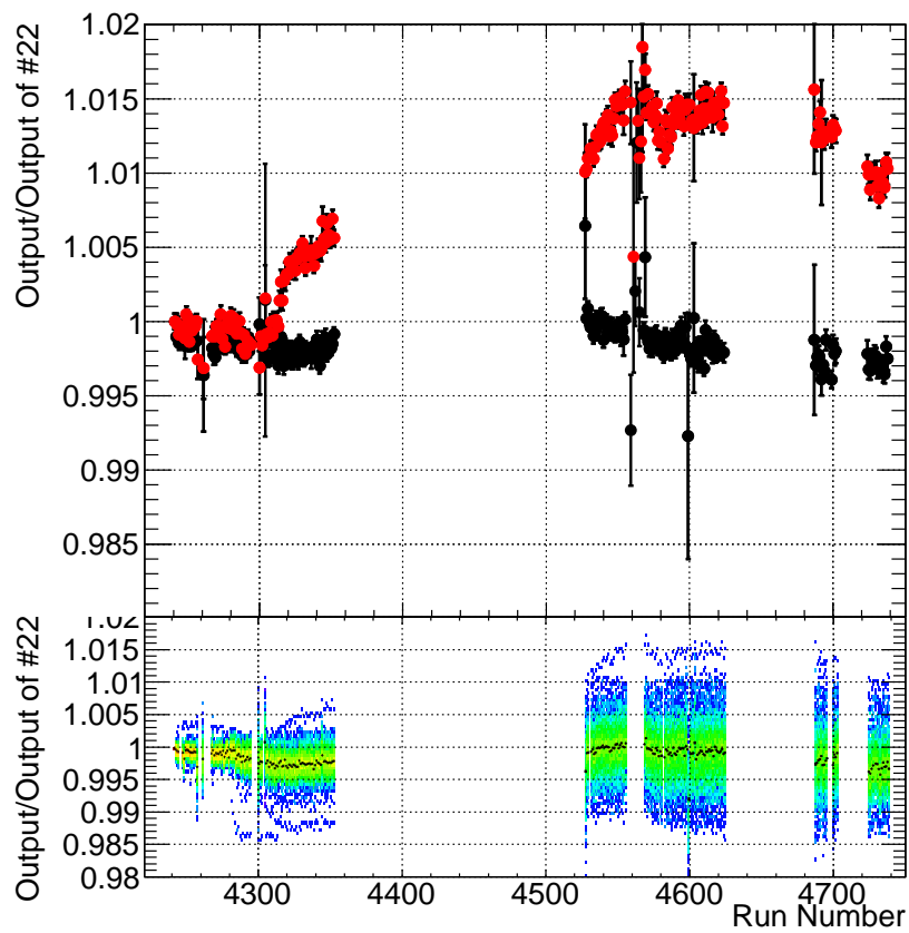
Figure 3.10: Temporal variations of pulse height ratio of the Laser event output. [TOP] Temporal variations of typical stable channel (black dots), and unstable channel (red dots). [Bottom] Temporal variations of multiple channels. Black dots represents mean value of the pulse height ratios.
