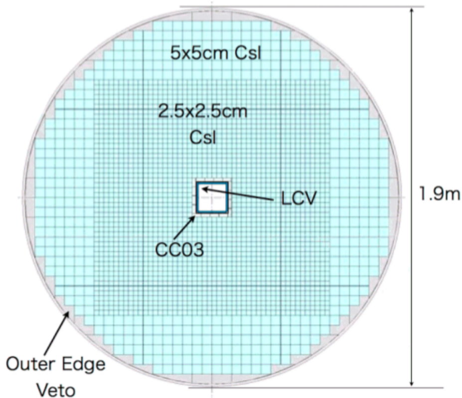
Figure 2.4: Geometry of CsI calorimeter and neighbouring VETO detectors. The CC03 is placed around the beam hole. The LCV is attached on the inner beam hole surface of CC03. Outer edge veto is placed between the CsI crystals and cylindrical support structure.
