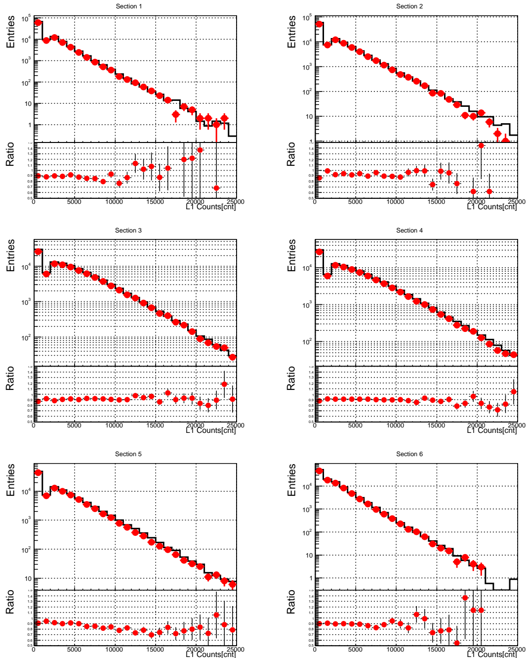
Figure 8.1: Distributions of L1 section count sum for section 1-6. The black line shows MC data, and red dots shows beam event data. The lower half shows the ratio between the two distributions (Beam/MC).
