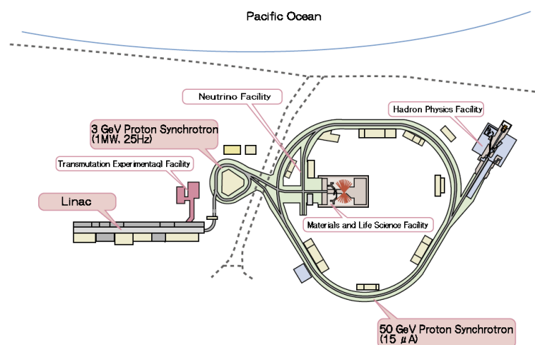
Figure 2.1: An overview of the J-PARC Facility [12].
