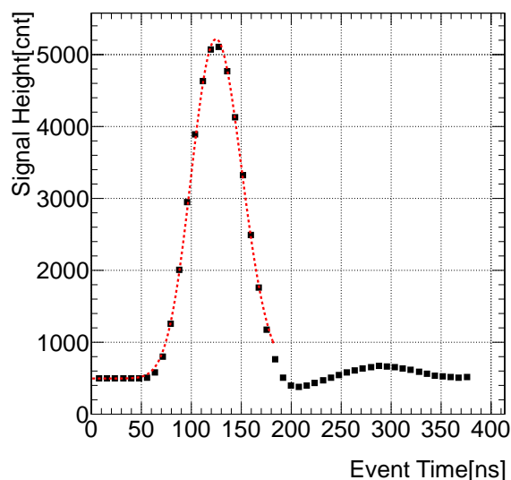
Figure 3.1: The raw data recorded by FADC. Points are recorded every 8 ns.
