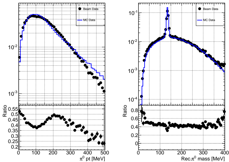
Figure 6.6: Distribution of reconstructed transverse momentum (left) and \pi^0 mass (right). Black dots show beam event data, and blue lines show MC data, and their ratio (Data/MC) are shown in the lower half.
