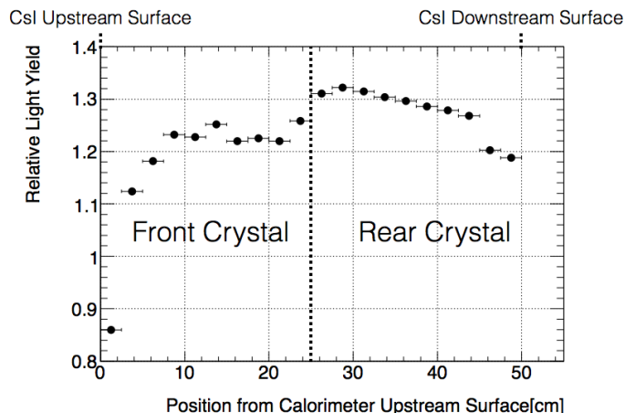
Figure 4.1: A Sample light yield distribution in the crystal ID 2511. Many crystals are made of two 25-cm-long crystals. It causes a large light yield change at the 25 cm from the CsI upstream surface. This was measured using RI source.
