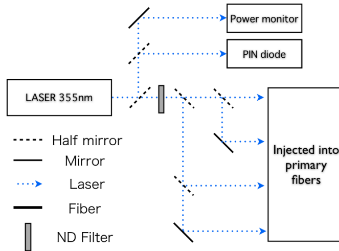
Figure 2.10: Schematic view of upstream part of Laser gain monitoring system. The Laser beam is divided with mirrors and injected into four primary fibers. The light intensity can be adjusted with a neutral density (ND) filter.
