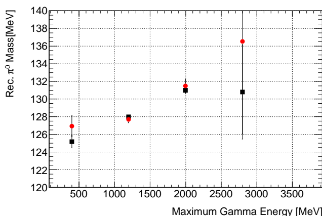
Figure 7.3: The mass of the \pi^0 with the largest gamma energy calculated with the averaged decay vertexes of other two \pi^0 s, is shown as a function of the maximum gamma energy. Black dots show the MC data with no nonlinearity, and red dots show the beam event data.
