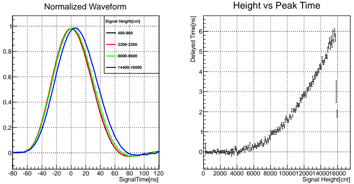
Figure 3.6: Changes of waveforms for various pulse heights. The changes of waveform of Laser event for different pulse height regions (left) and the correlation between timing delay and the pulse height (right) are shown.
