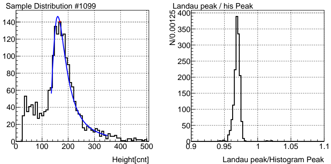
Figure 4.4: Sample of energy deposit distribution (left) and the ratio between fitted Landau peaks and peak of energy deposit distribution (right).
