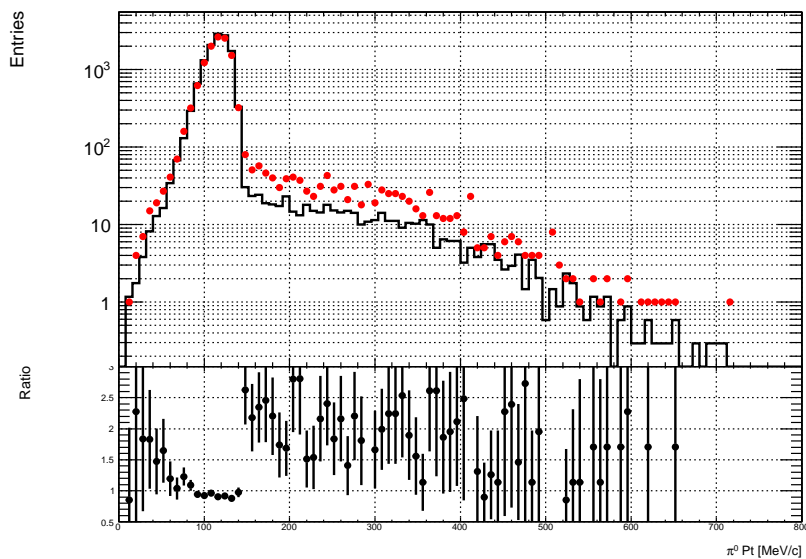
Figure 8.4: Transverse momentum distributions of \pi^0 after applying all gamma cuts on beam data (red dots) and MC (black solid line). The lower half shows the ratio between two distributions (Beam/MC).
