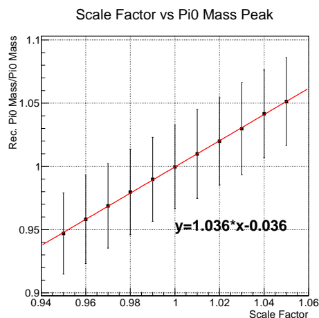
Figure 6.7: Relation between the fitted \pi^0 mass and the energy scale, (1/\Delta_E) . The error bar shows the sigma of the \pi^0 mass distribution.
