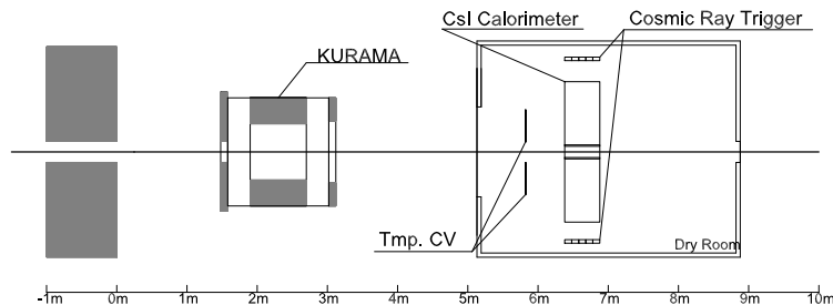
Figure 2.6: Schematic view of the experiment setup.
