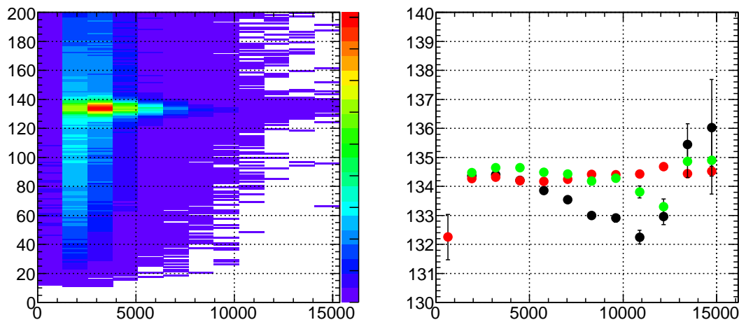
Figure 7.8: Correlation between the reconstructed \pi^0 mass and the maximum pulse height in the cluster. [Left] 2D distribution of \pi^0 mass and the maximum pulse height. [Right] \pi^0 peak value vs the max pulse heights, using the ordinary nonlinearity correction function (black), the correction function derived with 3\pi^0 calibration method (green), and MC with no nonlinearity (red).
