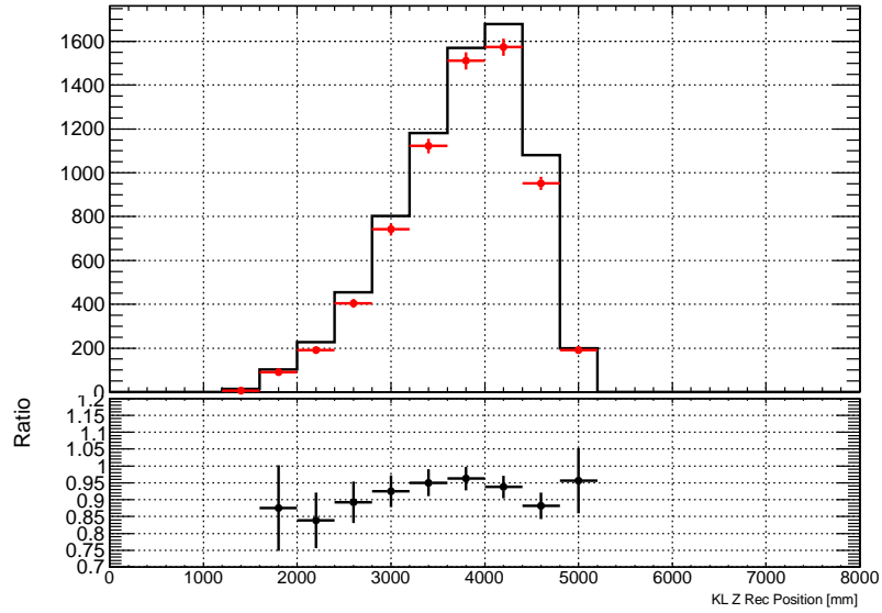
Figure 8.5: Distribution of z_{K_L} after applying all cuts. Red dots represent beam data, and black solid line represents MC. The lower half shows the ratio between two distributions (Beam/MC).
