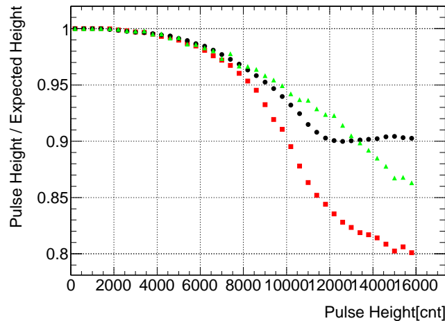
Figure 7.1: Signal height nonlinearity surveyed with the Laser Monitoring System for various modules: small modules (black), small modules where FADC are inserted in a specific VME crate (red), and large modules (green).
