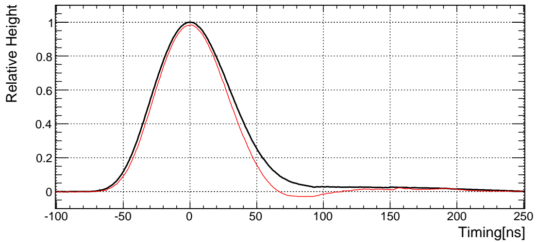
Figure 3.4: The template pulse shapes are shown for Laser events (red) and gamma shower events (black).
