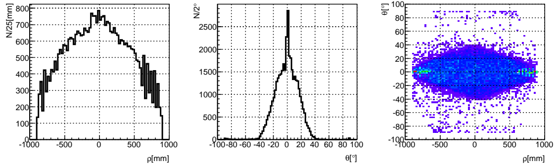
Figure 4.5: \rho – \theta distributions of cosmic ray events. [Left]:Distribution of \rho from \chi^2 minimization. [Middle]: \theta distributions. [Right]:2D-distribution of \rho and \theta .
