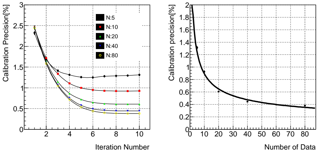
Figure 5.7: Statistical Effect on calibration accuracy. [Left]The changes of accuracy by iteration for various numbers of K_L events. Each color of point means different number of events used for the calibration (Yellow: 1 \times 10^{11} K_L , Blue: 5 \times 10^{10} K_L , Green: 2.5 \times 10^9 K_L , Red: 1.3 \times 10^9 K_L , Black: 6 \times 10^8 K_L ). [Right]The relation between the final calibration result at the 10th iteration and number of K_L events. The fitted function shows that the calibration accuracy is dominated by the statistics of K_L events.
