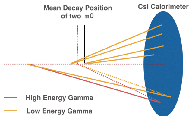
Figure 7.2: Concept of the nonlinearity survey using K_L \rightarrow 3\pi^0 decay.
