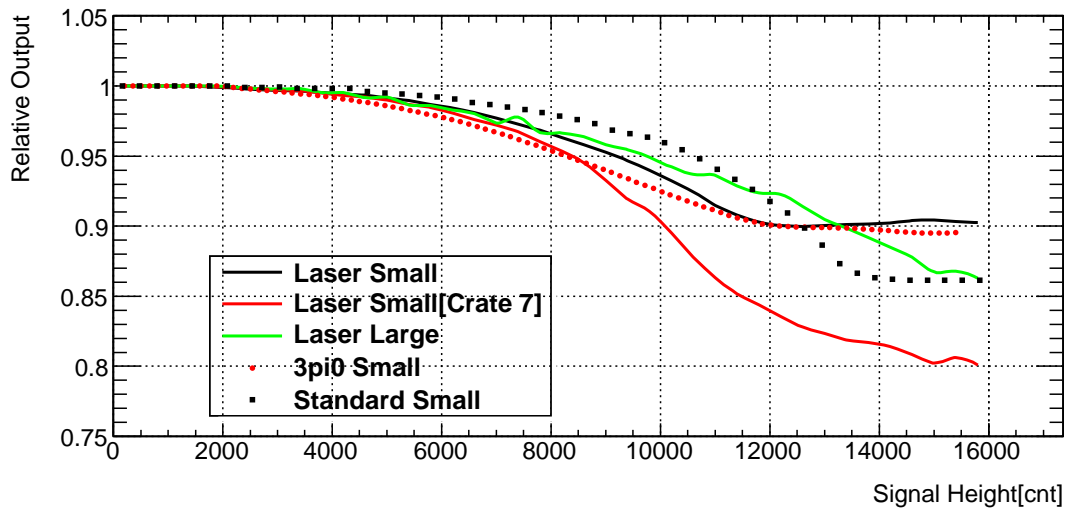
Figure 3.5: Output nonlinearities measured with various measurements. The nonlinearity which was measured in the previous test [16] is shown by dotted black line "Standard Small". The nonlinearities which was measured using the Laser system are shown by solid lines. In the previous test the nonlinearities did not depend on the crystal size. The nonlinearities using the laser system, however, shows a crystal size dependence.
