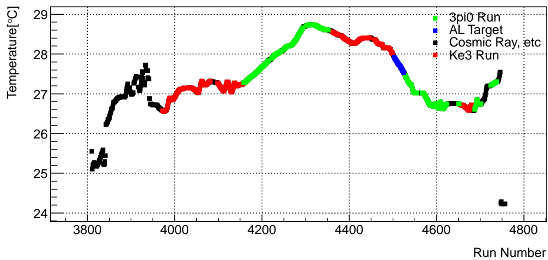
Figure 3.9: Temperature at the surface of the calorimeter during the data taking. Each color represents each type of run, 3pi0 (green), Ke3 (red), Special run with Al target (blue), and cosmic ray (black). The change in temperature was less than \pm 1.2^{\circ}\text{C} during 3pi0 Runs.
