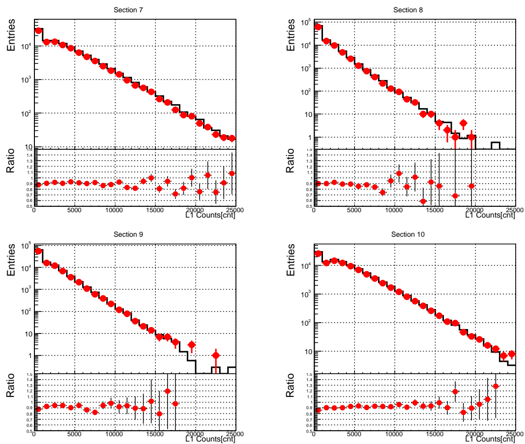
Figure 8.2: Distributions of L1 section count sum for section 7-10. The black line shows MC data, and red dots shows beam event data. The lower half shows the ratio between the two distributions (Beam/MC).
