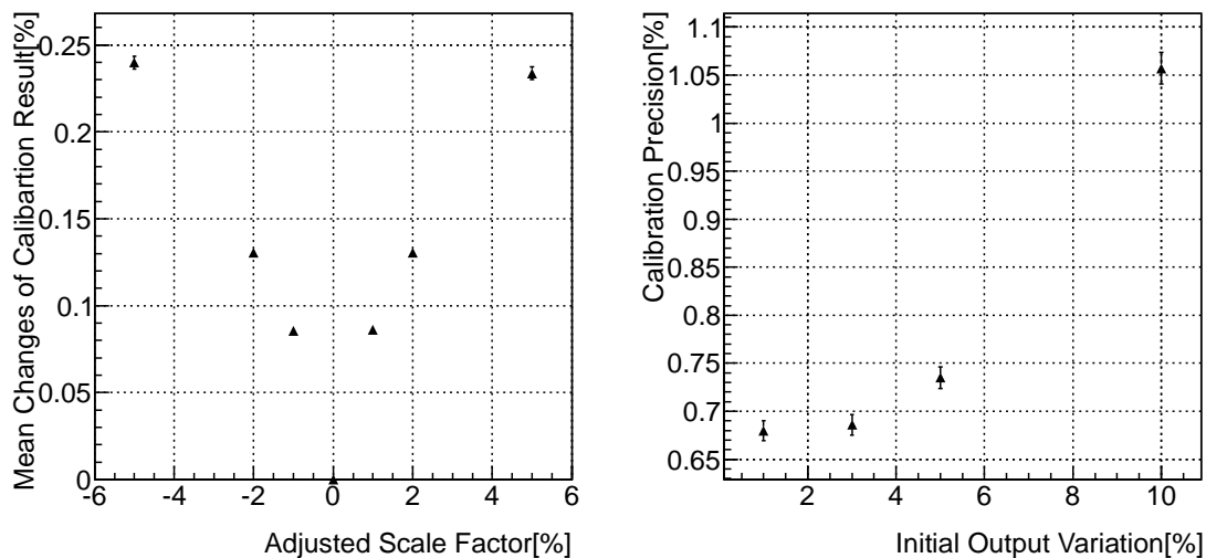
Figure 5.8: Effect of initial condition on the calibration result. [Left]Effect of overall scale factor on the calibration result. [Right]Effect of initial output variation on the calibration result. The x axis shows the RMS of initial output variation, and the y axis shows the final calibration accuracy.
