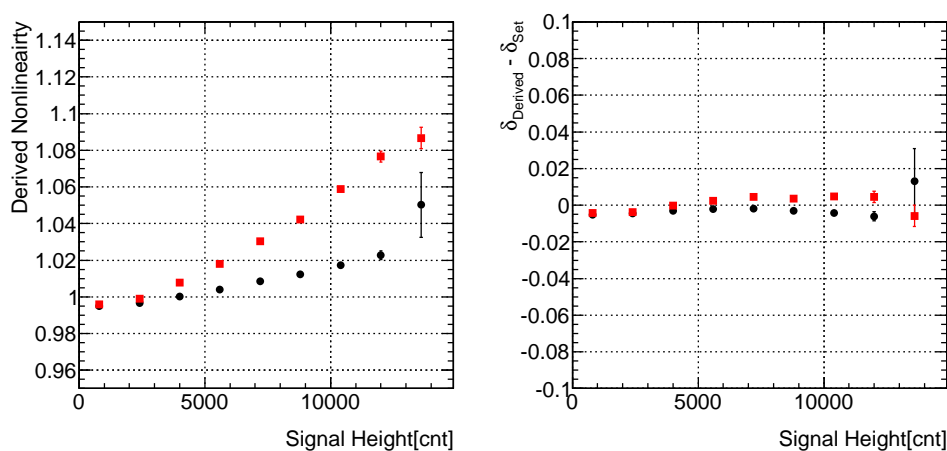
Figure 7.5: The nonlinearity derived from the MC test data for 2% (black dots) and 5% (red) nonlinearities. The left plot shows the derived nonlinearity. The right plot shows the difference between the derived nonlinearity and the applied nonlinearity.
