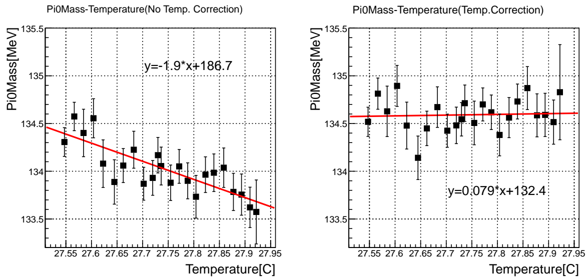
Figure 3.8: Correlation between reconstructed \pi^0 mass peak value and the calorimeter surface temperature for before (left), and after (right) applying temperature correction of (-1.48 \pm 0.03)\%/^{\circ}\text{C} . The red lines show fitted linear function.
