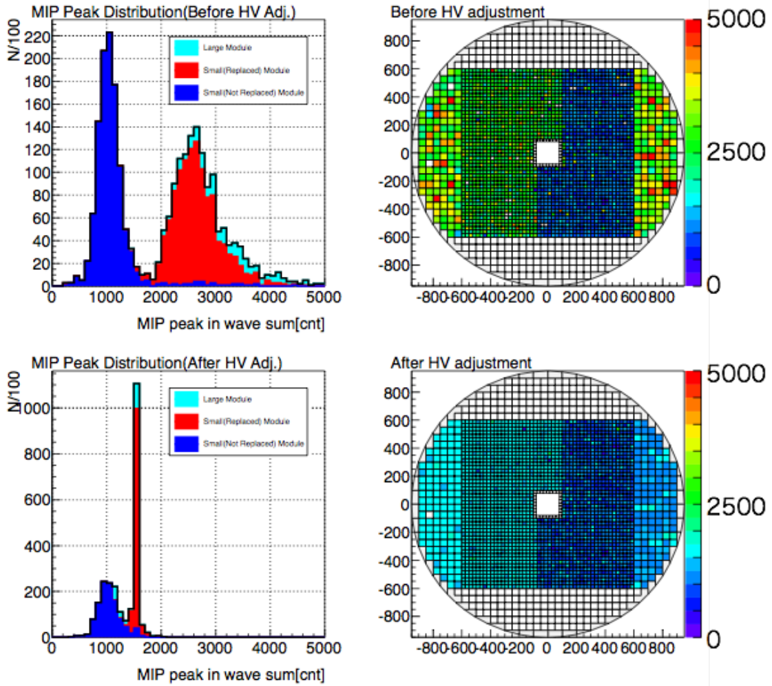
Figure 4.6: The result of cosmic ray calibration and HV adjustment. [Top left]The distribution of the peaks of fitted functions before HV adjustment. HV of all channels were set to 1750 V. The x-axis value was converted from the FADC count sum of the waveform. [Top right]The xy-distribution of peaks of MIP’s energy deposit. The outputs of the modules with damaged silicone cookies are half of others. [Bottom left]The distribution of the peaks of fitted functions after HV adjustment. [Bottom right]The xy-distribution of peaks of MIP’s energy deposit after HV adjustment.
