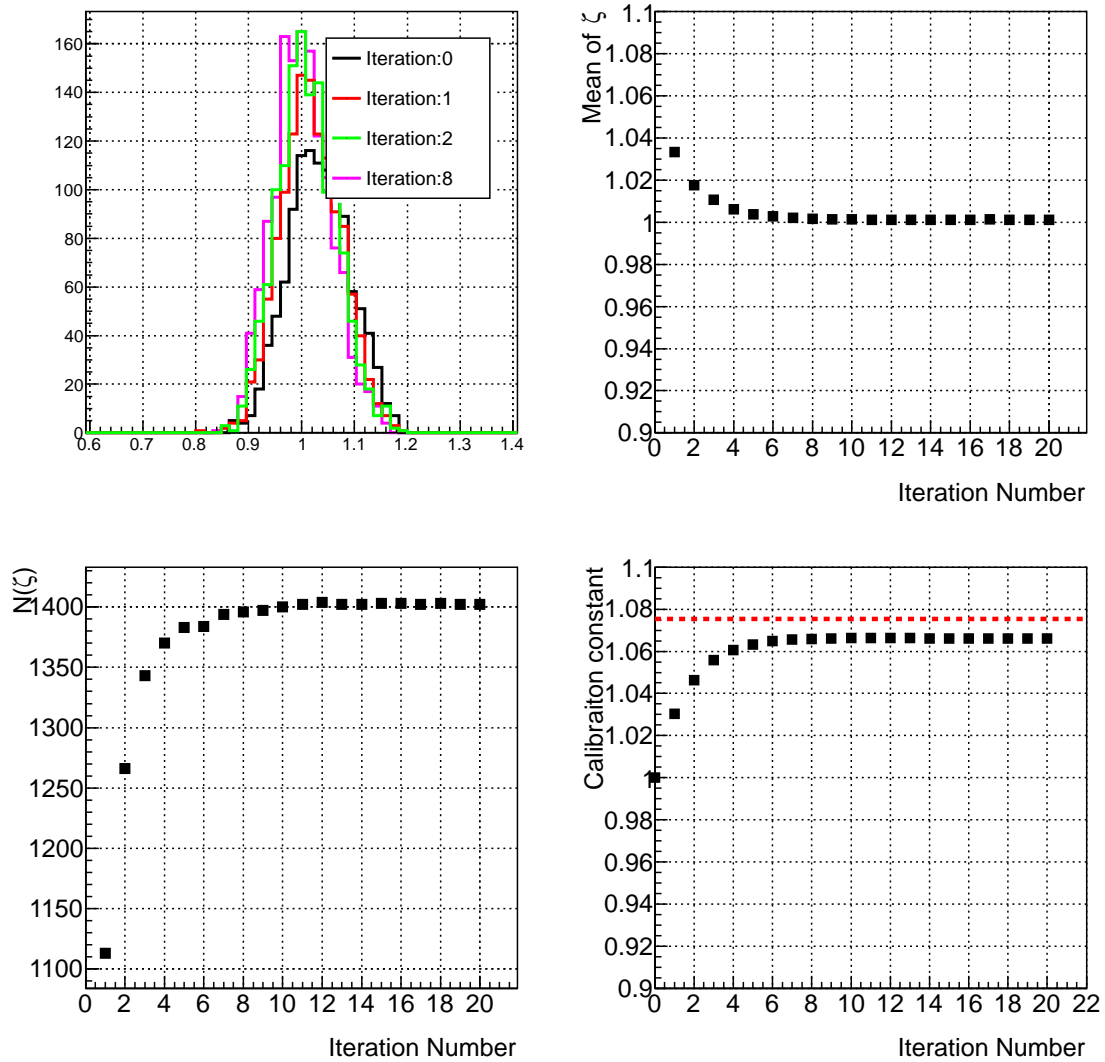
Figure 5.5: The convergence of calibration factor in a specific channel. [Top, Left]Raw distribution of \zeta after different numbers of iteration. [Top, Right]The average of \zeta vs the number of iterations. [Bottom, Left]The number of collected \zeta in a module vs the number of iterations. [Bottom, Right]The number of iterations vs the derived calibration constant for the module. The calibration constant in the figure is normalized by the initial calibration constant.
