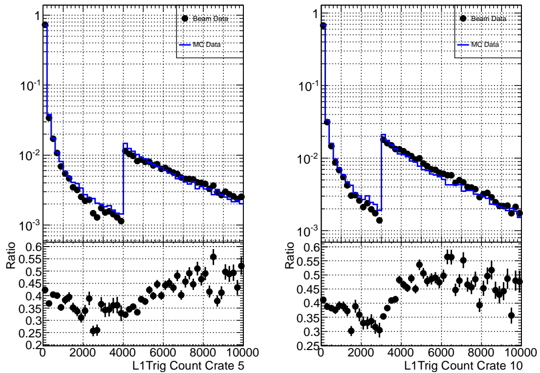
Figure 6.3: The distributions of L1 section energy sum in the energy scale calibration data. The L1 section energy sum was expressed in ADC counts, and the ratios, energy/ADC counts, were different for all sections. Therefore the thresholds for L1 sections were set by different value in ADC counts. The distribution of L1 section energy sum of section #5 (left) and section #10 (right) are shown. Black dots show beam event data, and blue lines show MC data. The section #5 was assigned for nominal small modules, and the section #10 was assigned for cookie-damaged modules.
