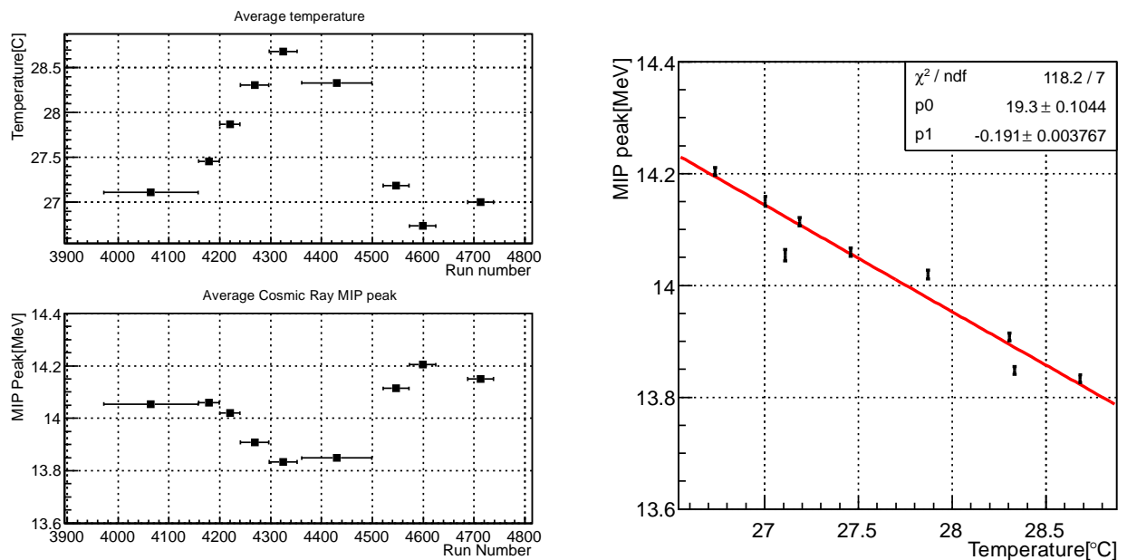
Figure 3.7: The temperature dependence of the representative cosmic ray outputs during data taking. [Left, Top]The surface temperature of the calorimeter vs run numbers. [Left, Bottom]The average MIP vs run numbers. [Right] The correlation of the representative cosmic ray outputs and temperature. The slope of fitted line was (-0.191 \pm 0.004) \text{ MeV}/^\circ\text{C} .
