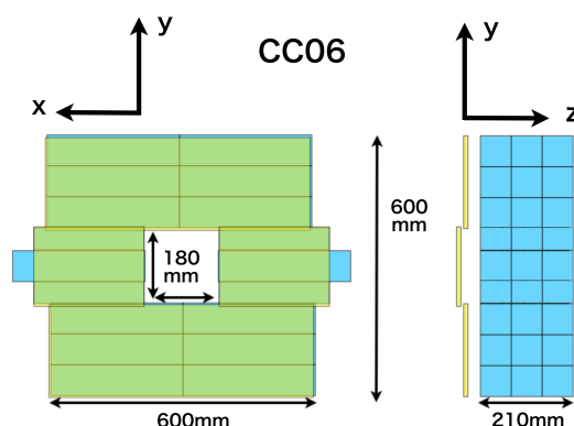
Figure 2.5: Structure of CC06. The CsI crystals (sky blue in the figure) are used to detect gammas. The plastic scintillators (green and yellow in the figure) are located upstream of the CsI crystals to identify charged particles.
