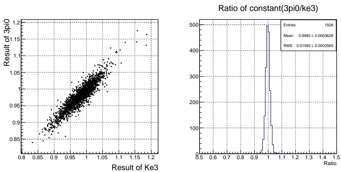
Figure 8.11: Correlation between my calibration result and the Ke3 calibration result [17]. The scatter plot of the results of two calibration methods (left) and their ratio distribution (right) are shown.
