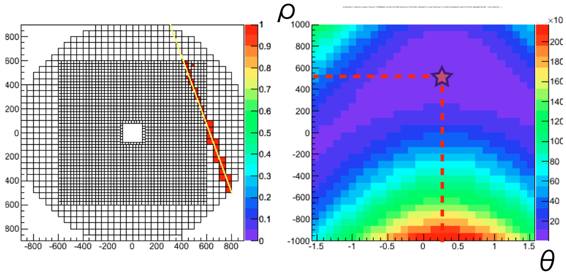
Figure 4.3: Sample of cosmic ray event (left) and the distributions of \chi^2 defined in Eq. 4.1(right). The star mark in the right figure shows where \chi^2 is minimum, and derived line is shown in the left figure as yellow line.
