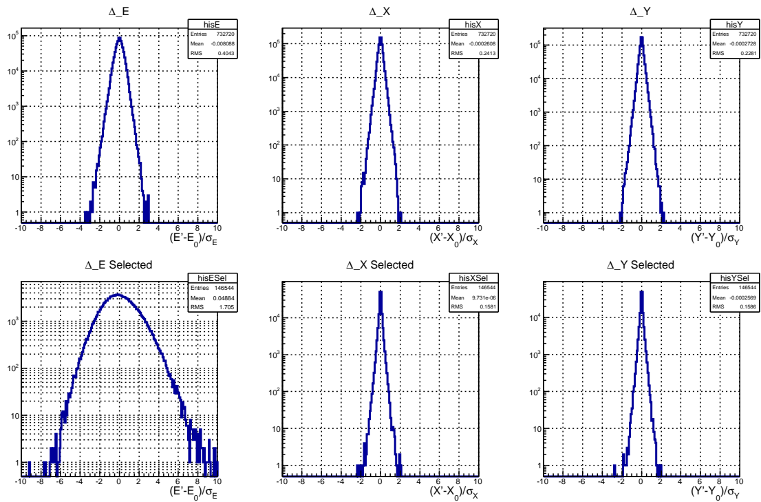
Figure 5.2: Changes of the measured parameters in the fitting. [Top, Left] \Delta distributions for gamma energies. [Top, Middle] \Delta distributions for gamma x position. [Top, Right] \Delta distributions for gamma y position. [Bottom, Left] \Delta distributions for the selected gamma energy. [Bottom, Middle] \Delta distributions for x position of the selected gamma. [Bottom, Right] \Delta distributions for y position of the selected gamma. The RMSs of \Delta distributions were less than 1 for measured parameters, but RMS of the \Delta distribution for the selected gamma energy ( v(4) ) was larger than other parameters.
