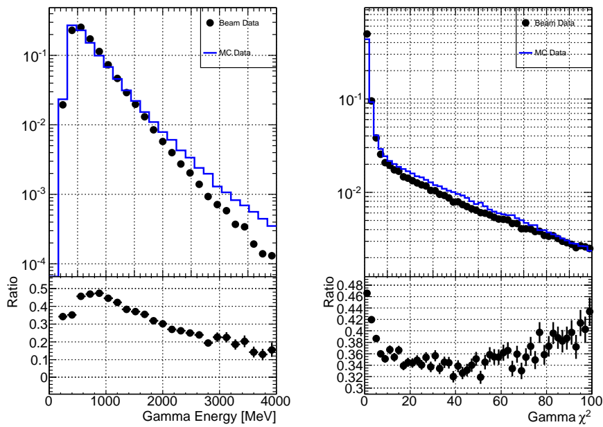
Figure 6.5: Distribution of gamma energy (left) and gamma \chi^2 (right; before applying gamma \chi^2 cut). Black dots show beam event data, and blue lines shows MC data. Their ratio (Data/MC) are shown in the lower half.
