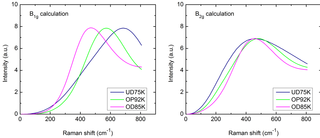
Figure 5.29: Doping dependence of calculated spectra in two geometries B_{1g} and B_{2g} . Peak position in B_{1g} increases clearly with underdoping while it changes lightly with a dome shape in B_{2g} .
