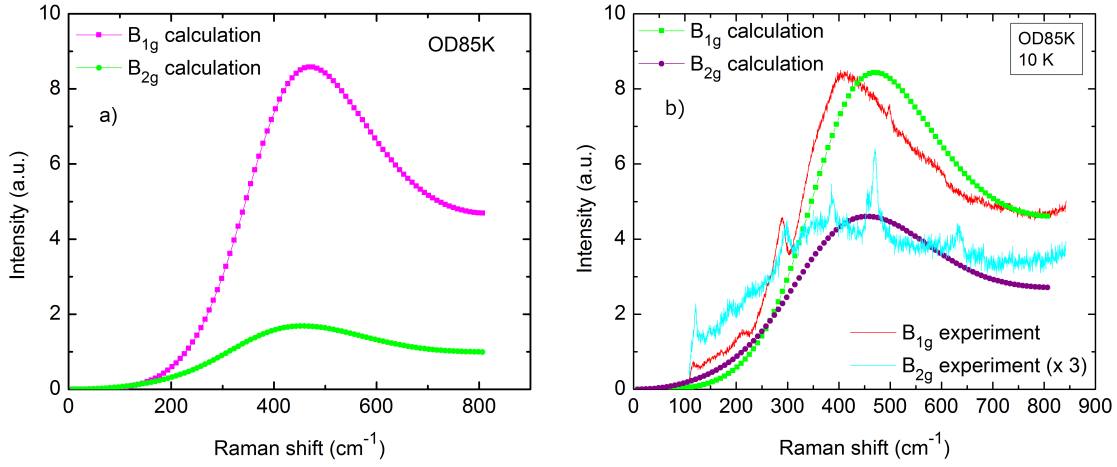
Figure 5.28: a) The original calculated B_{1g} and B_{2g} Raman spectra in superconducting state of the sample OD85K using ARPES data on whole Brillouin zone and subtracted Shirley backgrounds b) Comparison between the calculation results and experimental data, the experimental B_{2g} is multiplied by a factor of three to see more clear and the calculated spectra were normalized their intensity to the experimental ones.
