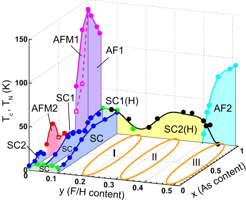
Figure 4.7: The phase diagram of \text{LaFeP}_{1-x}\text{As}_x\text{O}_{1-y}(\text{F}/\text{H})_y [56, 59, 71, 72, 73, 82].
