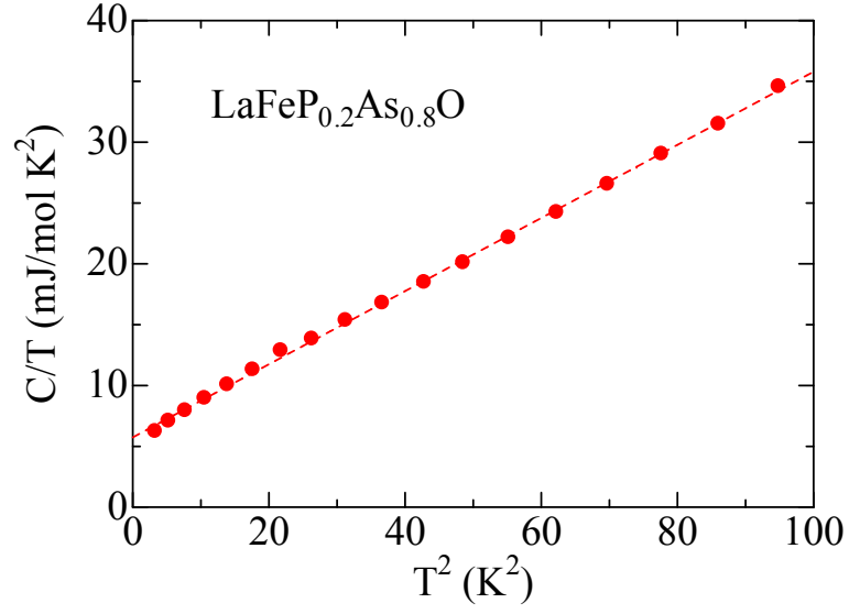
Figure 3.39: The T^2 dependence of specific heat C/T of \text{LaFeP}_{0.2}\text{As}_{0.8}\text{O} .
