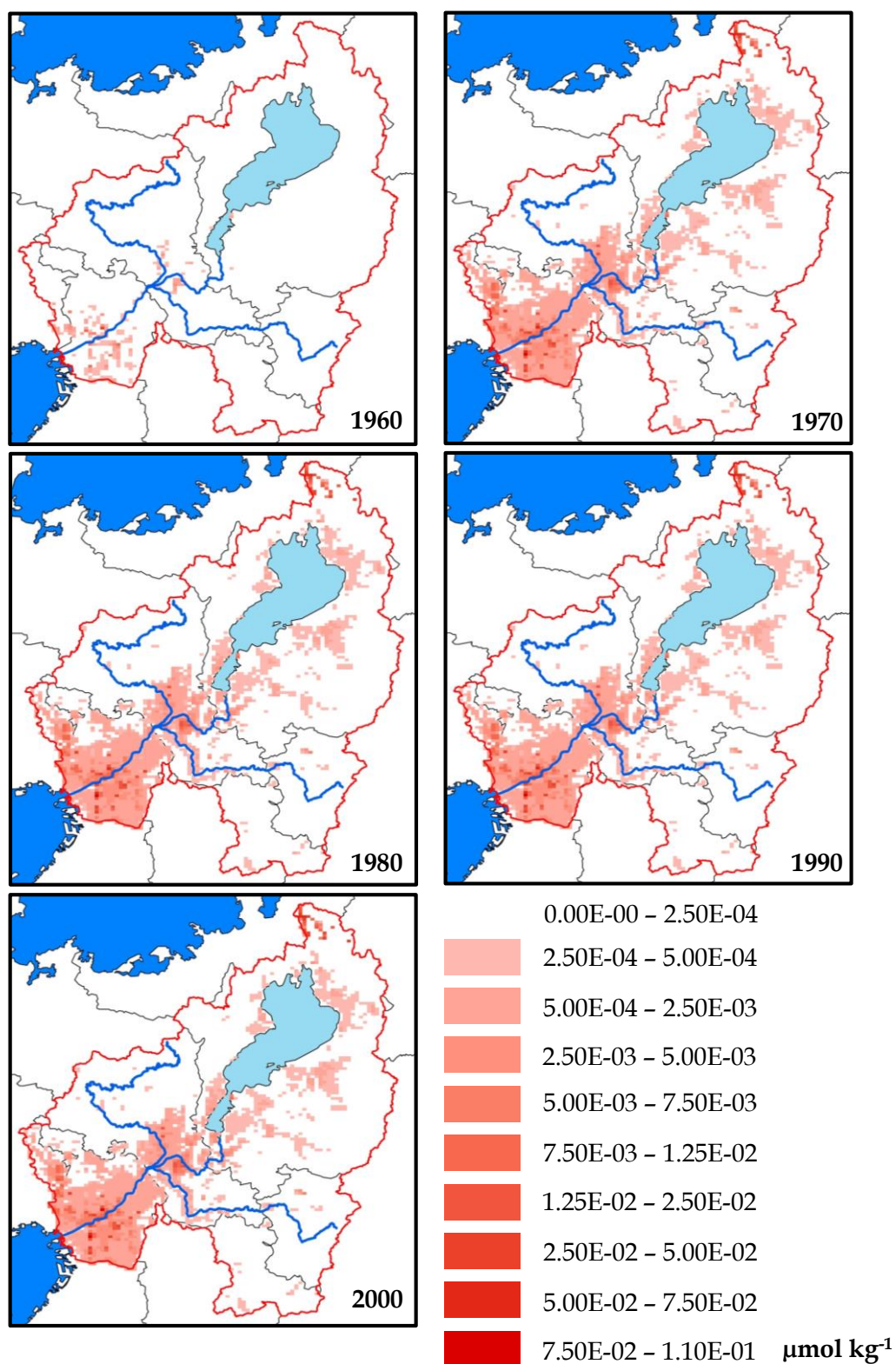
Fig. 5.5 Spatial distribution of the Hg concentration in the soil of LBVRB from 1960 to 2000.
