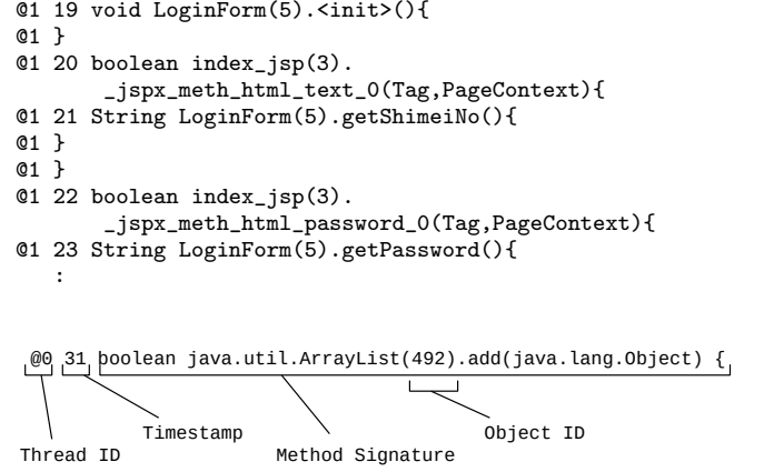
Figure 2: An example trace
