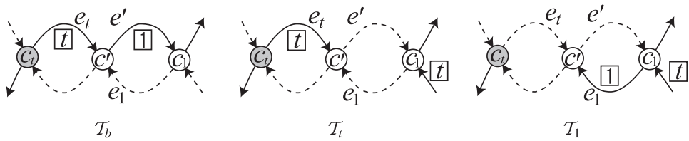
Fig. 11. The edges drawn by broken line are not contained.
