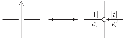
Fig. 1. The alternating orientation and the weights of edges.
