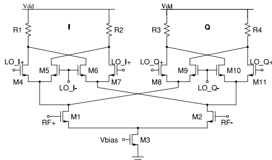
Fig. 6 Quadrature mixer with shared transconductor.
