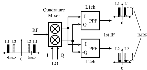
Fig. 5 Block diagram of image-reject mixer.
