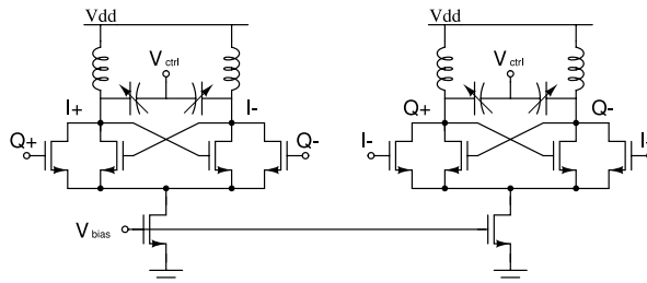
Fig. 7 Quadrature-coupled LC-VCO.
