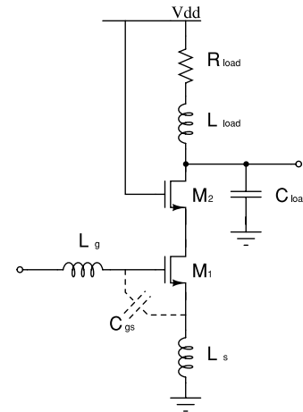
Fig. 2 Circuit of LNA.
