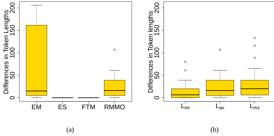
Figure 4.7: Box plots of L_{av} for EM, ES, FTM, and RMMO patterns (a), and of L_{mi} , L_{av} , and L_{mx} for RMMO pattern (b)
