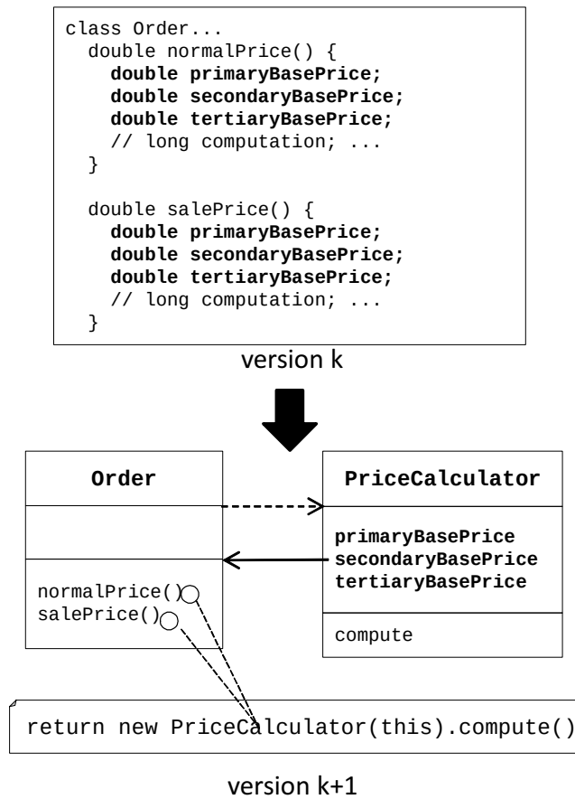
Figure 4.3: An example of clone refactoring using RMMO pattern]
