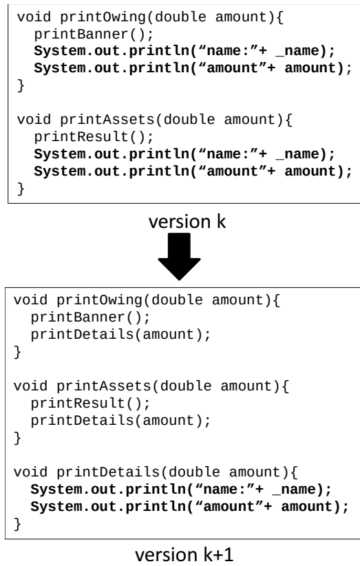
Figure 4.2: An example of clone refactoring using EM pattern
