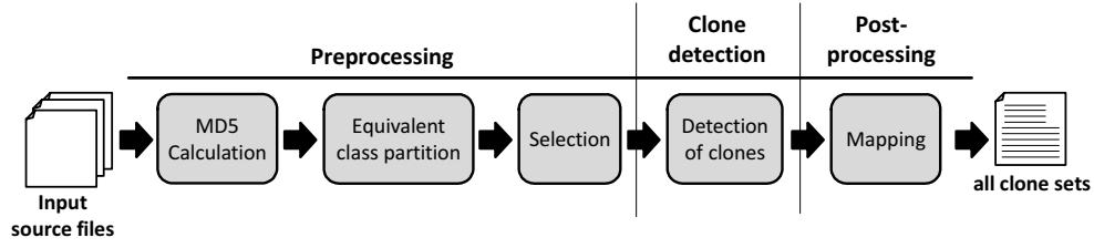
Figure 3.2: Overview of approach with non-normalization
