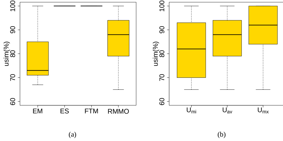
Figure 4.6: Box plots of U_{av} for EM, ES, FTM, and RMMO patterns (a), and of U_{mi} , U_{av} , and U_{mx} for RMMO pattern (b)
