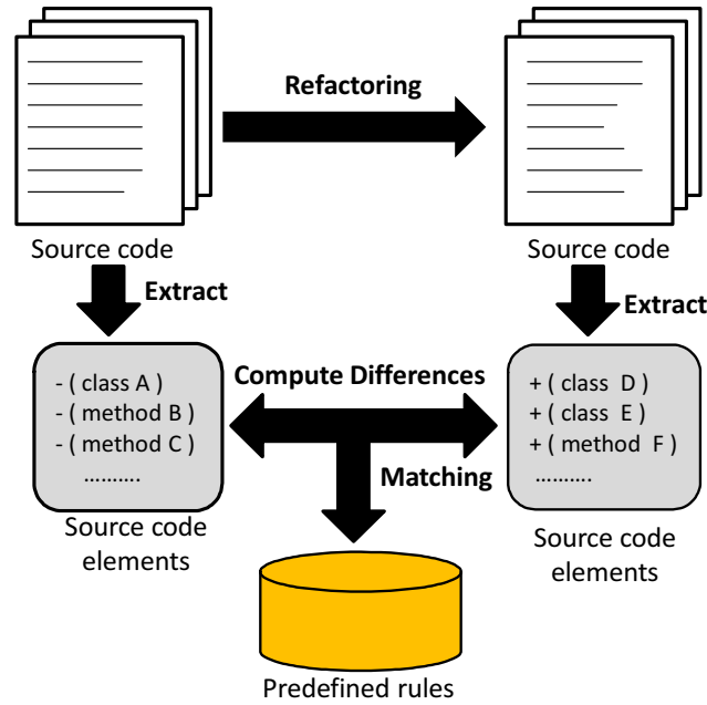
Figure 2.1: Overview of a rule-based refactoring detection approach
