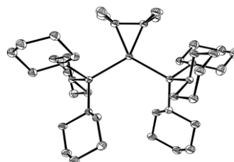
Figure 2.1. ORTEP structure of 3 .
