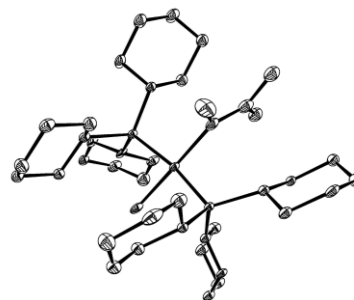
Figure 2.2. ORTEP structure of 4 .
