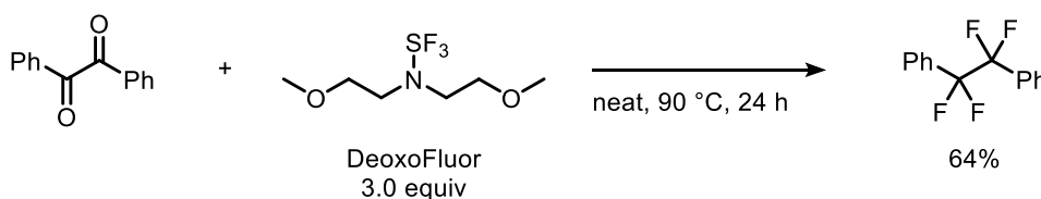
Scheme 1.6. Deoxofluorination of 1,2-diketones with DeoxoFluor. 15
