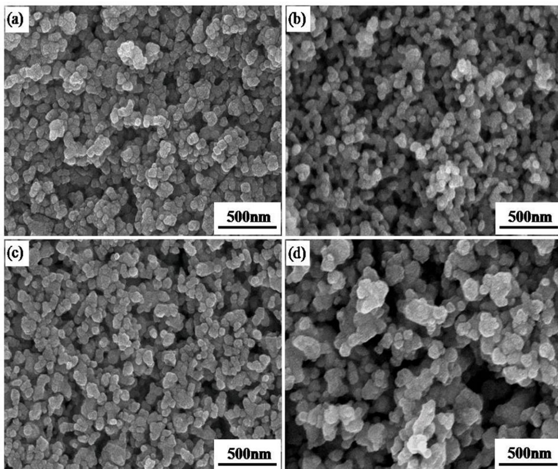
Fig. 5.2 SEM images of as-synthesized NiO-YSZ powders containing (a) 30, (b) 40, (c) 50 and (d) 70 vol% Ni.
