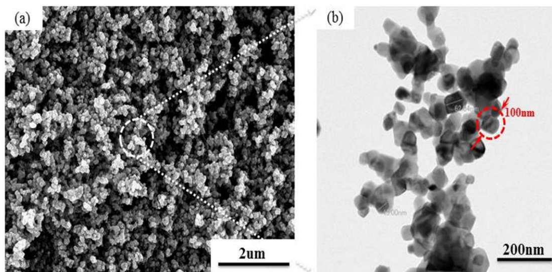
Fig. 4.4 SEM and TEM images of the synthesized NiO-YSZ composite powder (sample-2) calcined at 1000^{\circ}\text{C} . (a) SEM image; (b) TEM image.
