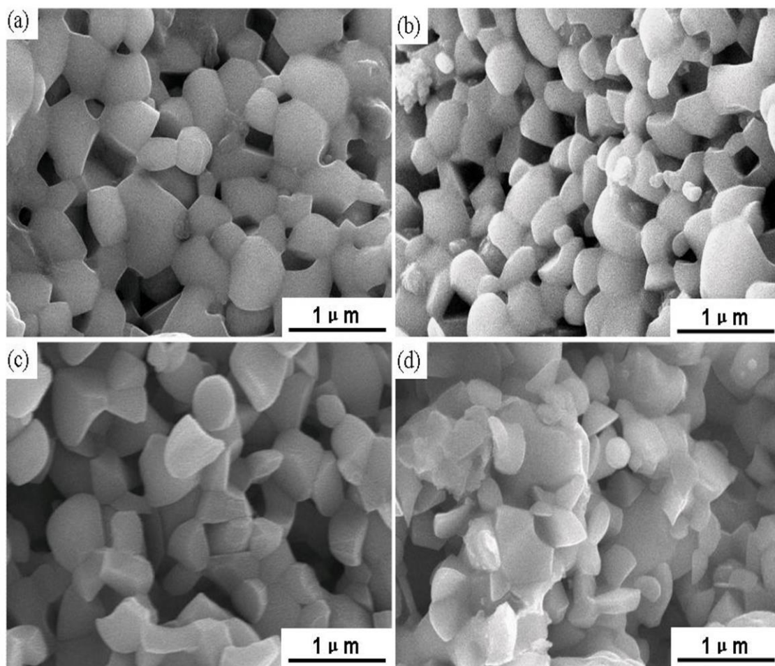
Fig. 5.6 SEM images of Ni/YSZ cermet containing (a) 30, (b) 40, (c) 50, and (d) 70 vol% Ni.
