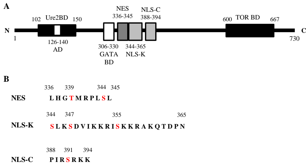
Fig. 11 Schematic representation of Gln3. (A) The structural domains of Gln3; this model is based on previous reports (Carvalho and Zheng 2003; Kulkarni et al. 2001). AD, activation domain; BD, binding domain. (B) Amino acids sequences of the NES, NLS-K and NLS-C regions (Saccharomyces Genome database; http://www.yeastgenome.org/ ). The residues substituted to alanine or aspartic acids are shown in red font.
