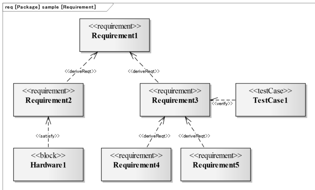
Fig. 3.4 Requirement diagram example.
