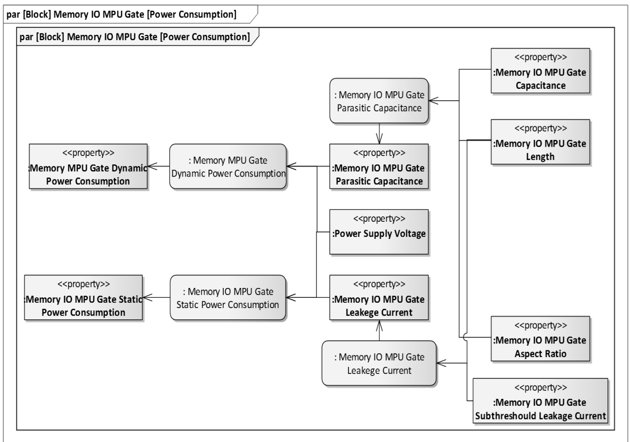
Fig. A.59 Memory IO MPU gate internal block diagram.
