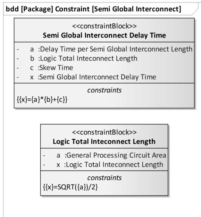
Fig. A.22 Detail of semi global interconnect constraint block.
