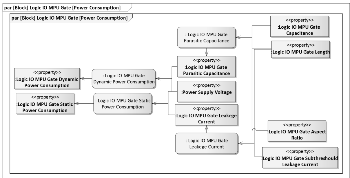
(a) Power consumption. Fig. A.33 Logic IO MPU gate parametric diagram.
