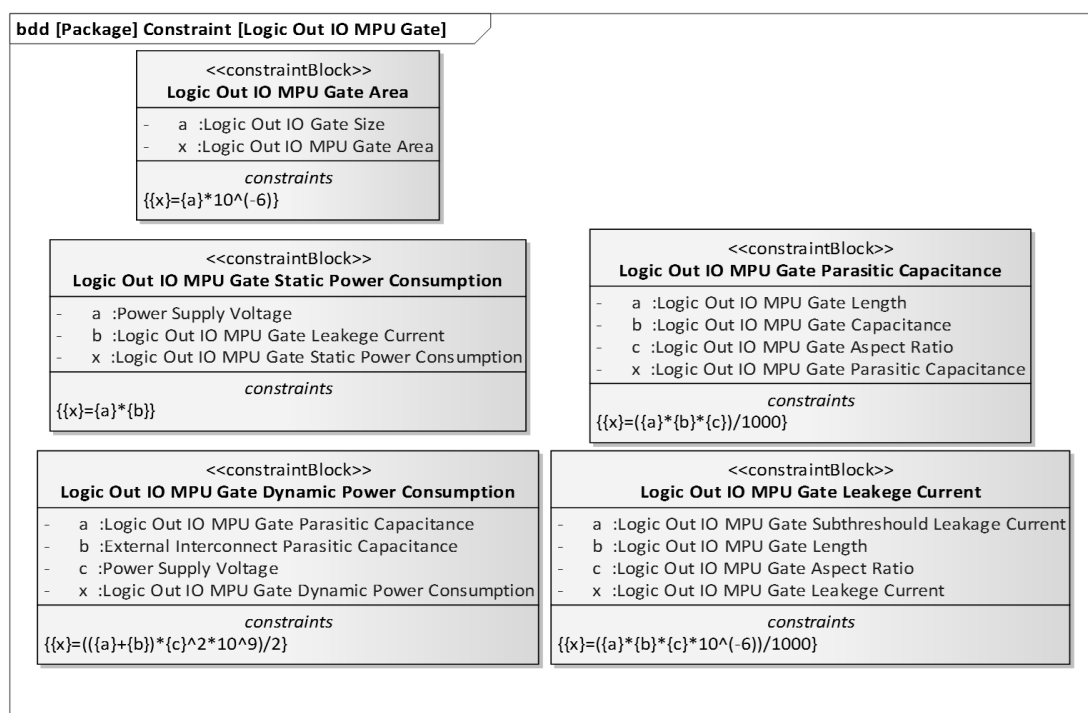
Fig. A.40 Detail of logic out IO MPU gate constraint block.
