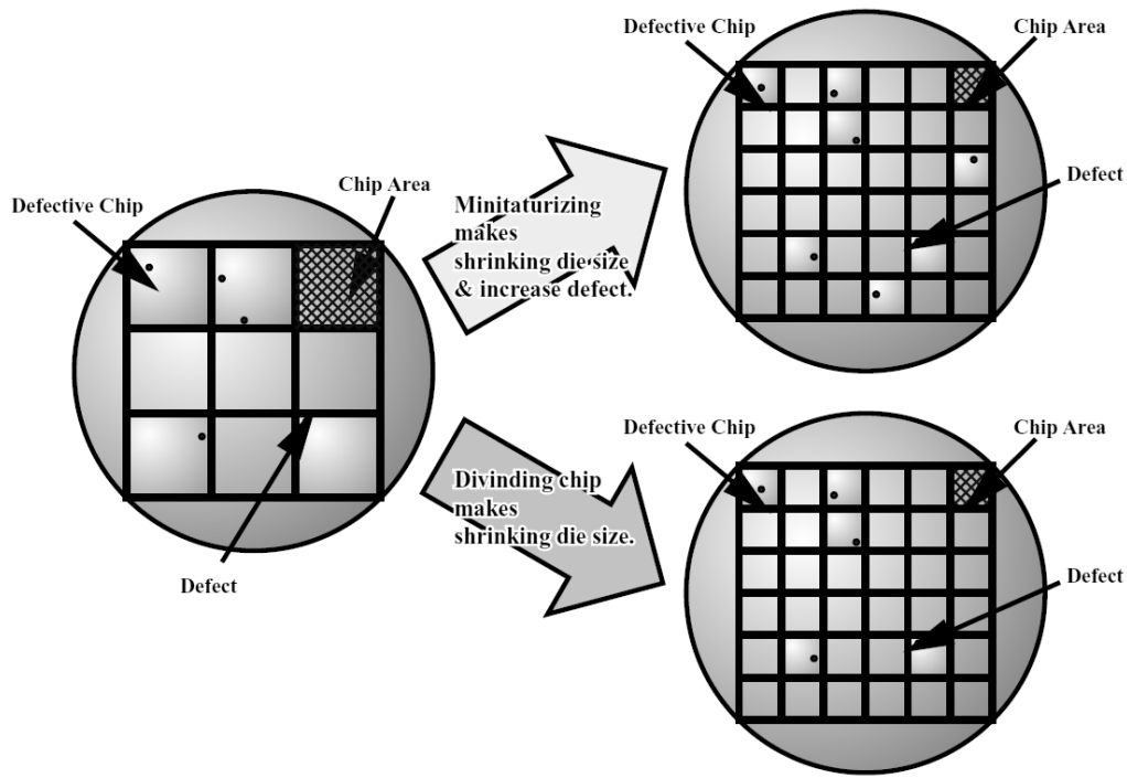
Fig. 4.11 The effect on cost of miniaturization and dividing chips.
