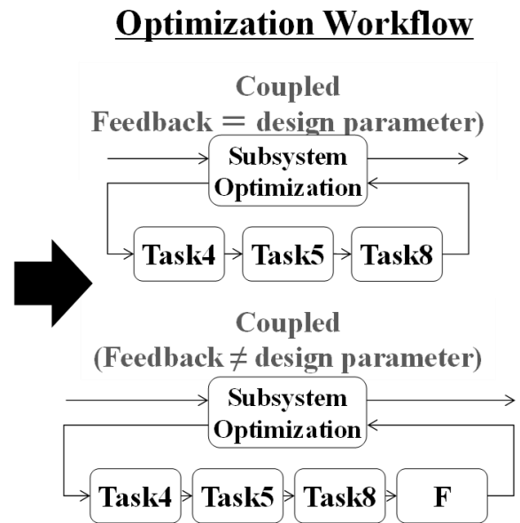
Fig. 3.30 Proposal method of constructing optimization execution workflow from partitioned DSM.
