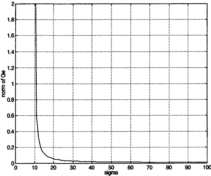
Figure 4.26: \|G_e(s)\|_\infty for specified poles
