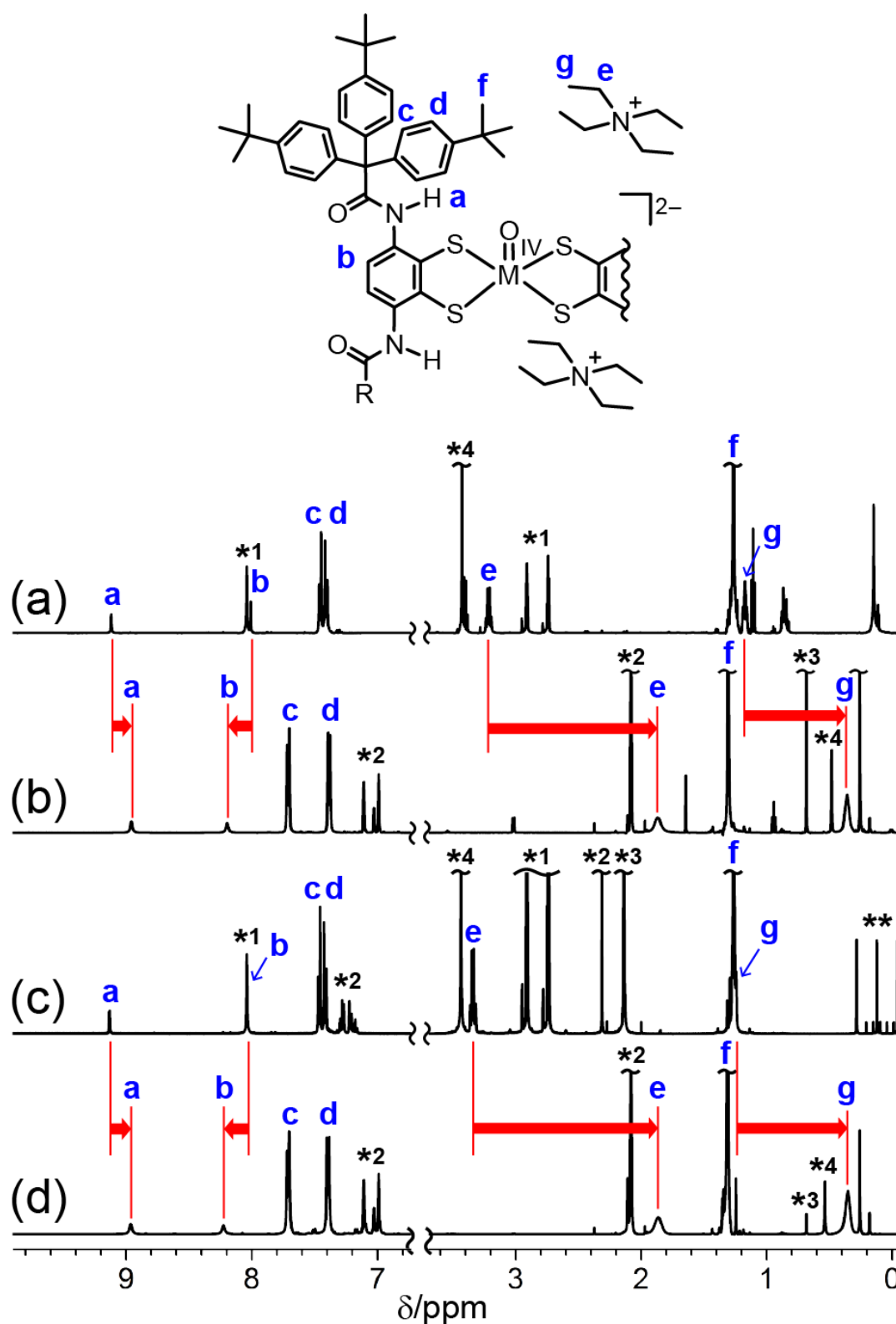
Figure 7. ^1\text{H} NMR spectra of (a) 1-Mo in \text{DMF-}d_7 , (b) 1-Mo in \text{toluene-}d_8 , (c) 1-W in \text{DMF-}d_7 , and (d) 1-W in \text{toluene-}d_8 at 30 ^\circ\text{C} . The asterisks denote solvents as a contaminant (*1: DMF; *2: toluene; *3: acetonitrile; *4: water). The double asterisk (**) denotes \text{BH}_4^- used for clear spectrum by reducing a trace amount of \text{W}^{\text{VO}} species.
