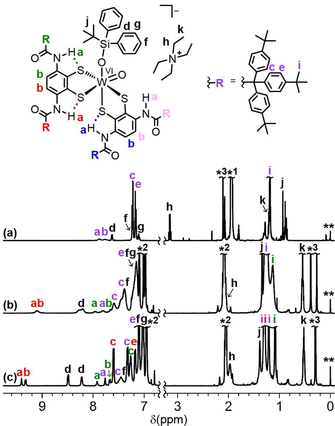
Figure 4. ^1\text{H} NMR spectra of 3 in (a) \text{CD}_3\text{CN} at 30^\circ\text{C} , (b) \text{toluene-}d_8 at 30^\circ\text{C} , and (c) \text{toluene-}d_8 at -45^\circ\text{C} . The two set of assignable signals and unassignable signals are colored in red, green, and purple, respectively. The asterisks denote solvents as a contaminant (*1: acetonitrile; *2: toluene; *3: water). The double asterisk (**) denotes TMS.
