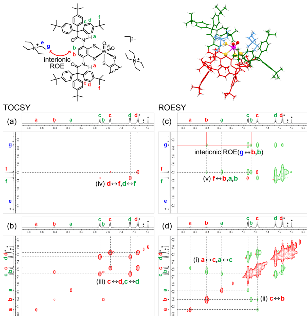
Figure 10. (a,b) TOCSY and (c,d) ROESY spectra of 2-W in toluene- d_8 at -45\text{ }^{\circ}\text{C} . The asterisks denote the residual signals of toluene- d_8 . Assignment of red and green protons is represented in (i) to (v).
