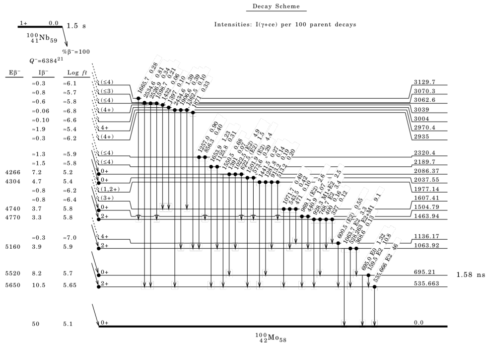
FIGURE C.1: Level diagram of 100 Mo[50]
