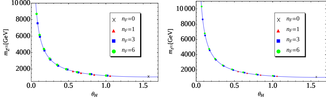
Figure 10: \theta_H vs m_{Z^{(1)}} and \theta_H vs m_{t^{(1)}} for m_H = 126 GeV with n_F degenerate dark fermions in the left and right panels, respectively. Blue line in the left panel is fitting function m_{Z^{(1)}} \sim 1044 \text{ GeV}/(\sin \theta_H)^{0.808} . Blue line in the right panel is fitting function m_{t^{(1)}} \sim 1033 \text{ GeV}/(\sin \theta_H)^{0.862} . In the n_F = 0 case Wilson line phase is \pi/2 . The left panel of this figure is originally shown in [13].
