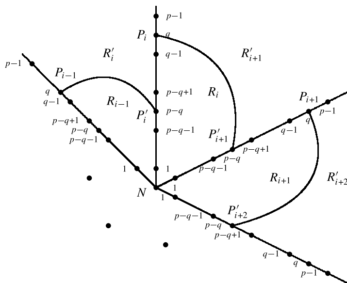
Fig. 4. The Minkus polyhedral scheme for M_n(p, q) .
