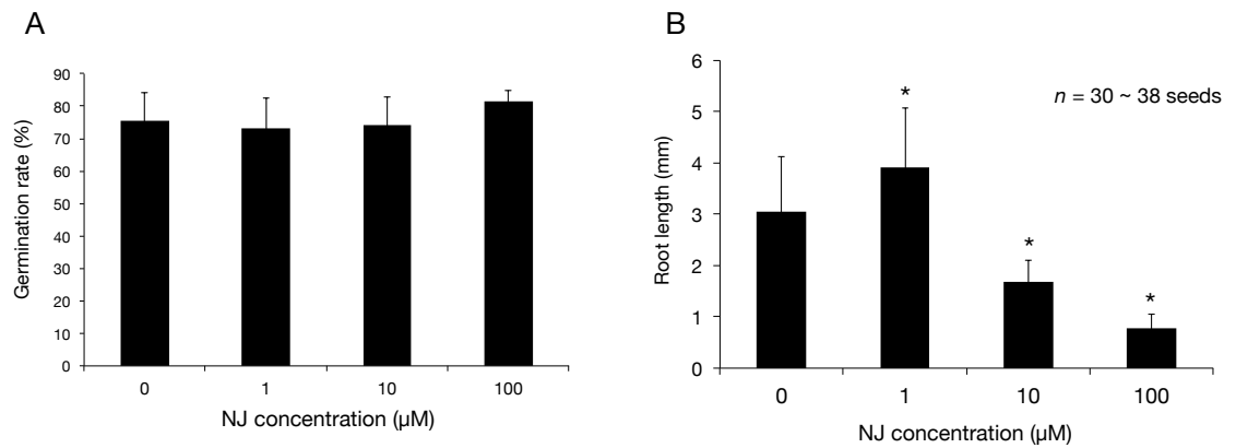
Figure 10. Effects of NJ on seed germination (A) and root elongation (B) of P. japonicum . (A) NJ, even at 100 μM, did not affect germination rate of P. japonicum . Number of germinated seeds (out of 20) was counted (mean \pm SD, n = 3 ). (B) Effects of NJ on root elongation became visible at 10 μM; root length of seedlings treated with 100 μM NJ was approximately one-quarter that of control. Radicle lengths of 30 to 38 germinated seeds were measured using ImageJ software. Asterisks indicate significant differences in the root lengths between control and NJ-treated seeds ( P < 0.05 , Student's t test).
