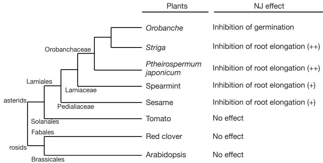
Figure 16. Relationship between plant evolution and NJ effect. The order and family were classified based on Angiosperm Phylogeny Group III system (Angiosperm Phylogeny Group, 2009), and parasitic plants in the Orobanchaceae were assigned by proposed evolutionary process (Westwood et al. , 2010). The plant species is closer to O. minor , the stronger the effect of NJ appeared. (++) indicates strong inhibitory effect; (+) indicates weak inhibitory effect.
