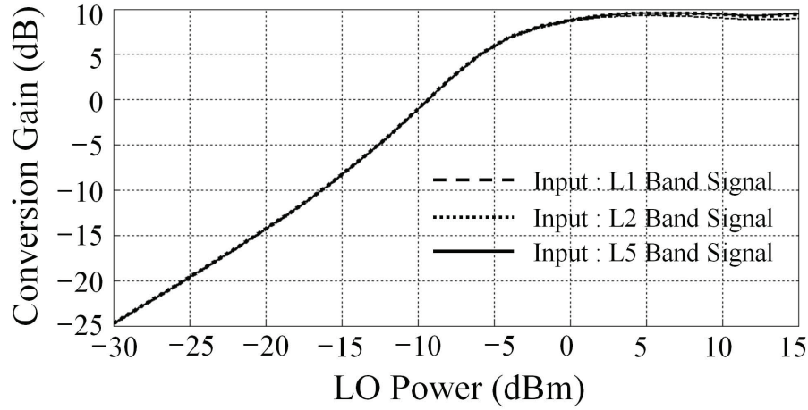
Figure 4.14: Mixer's conversion gain against LO power at triple-band signal.
