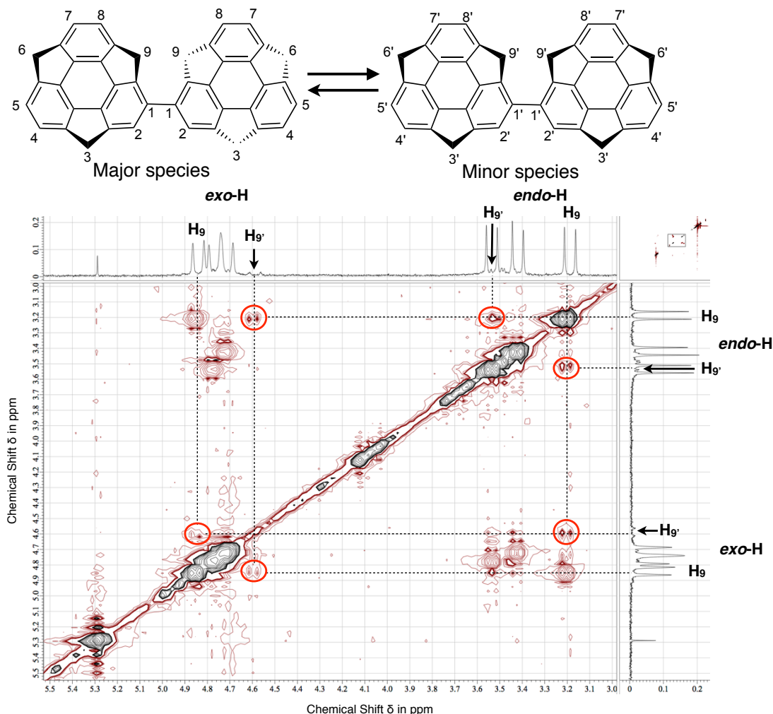
Figure 3.3 EXSY spectrum (600 MHz) of 39 in \text{CDCl}_3 at room temperature. The cross signals between the major signals (endo- and exo- H_9 ) and the minor signals (endo- and exo- H_9' ) are indicated by circle.
