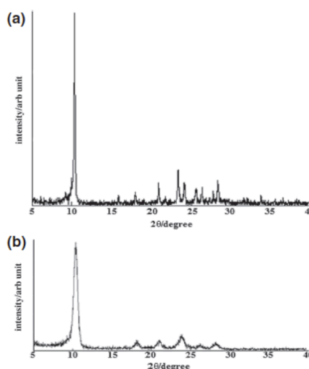
Figure 5.5 XRD pattern of 8 . a) single crystalline. b) nanocrystal.
