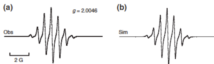
Figure 5.8 (a) EPR spectrum of 8^{\bullet-} generated by photoinduced electron-transfer reduction of 8 with (BNA) 2 in deaerated CH 3 CN at 298 K. (b) Simulated EPR spectrum obtained from a (H \times 6) = 0.70 G and \Delta H_{\text{msl}} = 0.12 G.
