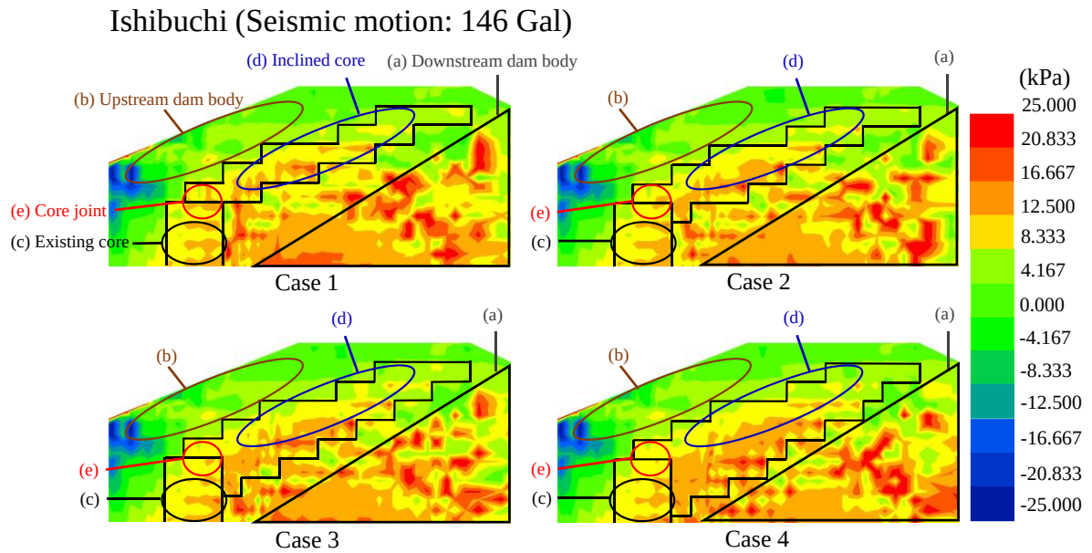
Figure 3.29 Shear stress distribution near the core joint (Ishibuchi seismic motion)
