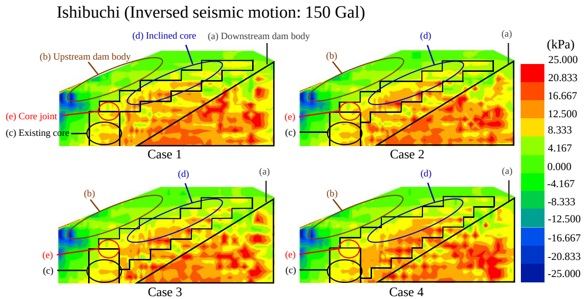
Figure 3.30 Shear stress distribution near the core joint (Ishibuchi inversed seismic motion)
