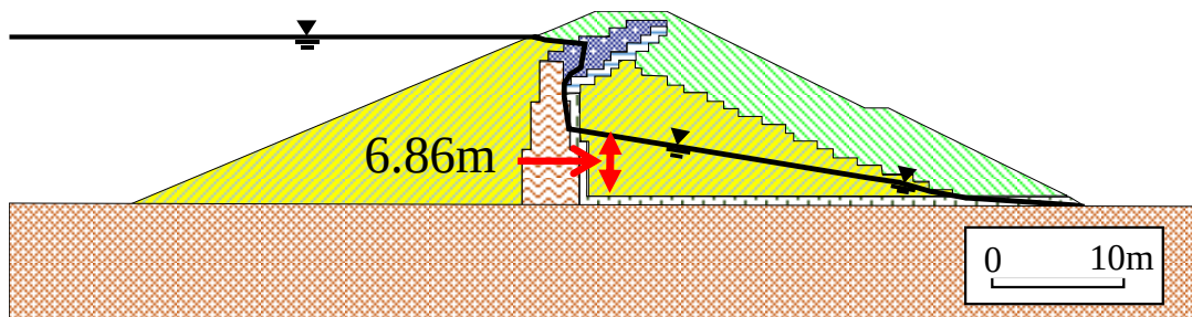
Figure 2.8 Change of seepage line in the model of Case 4
