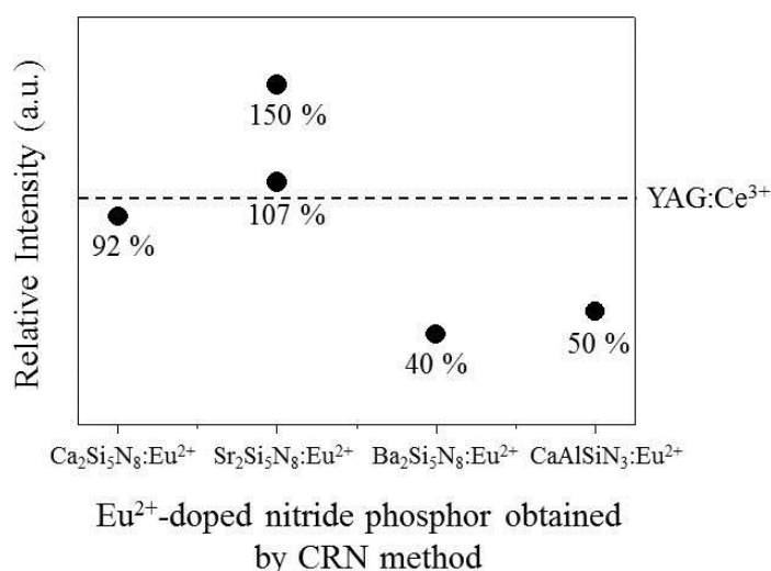
Fig. 2-1. Relative emission intensity of \text{Eu}^{2+} -doped nitride phosphors compared with \text{YAG:Ce}^{3+} phosphor.
