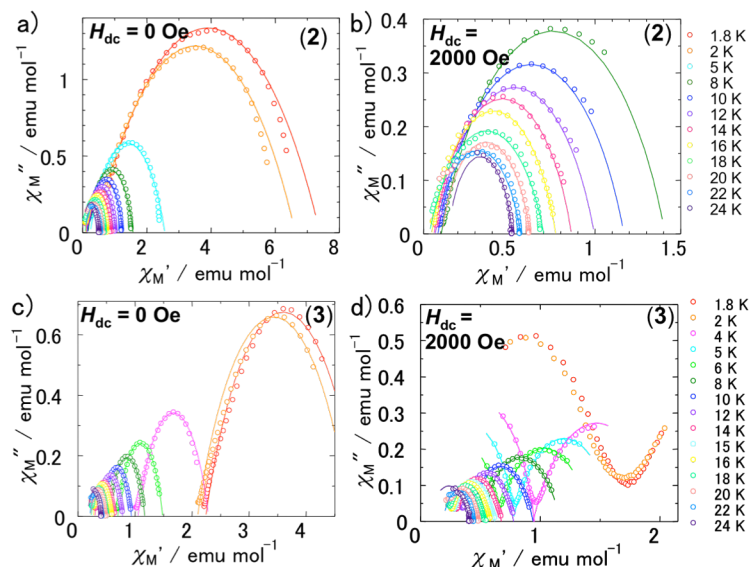
Figure 7. Argand plots for a crystalline powder sample of anionic form 2 in (a) zero dc magnetic field and (b) 2000 Oe magnetic field, and for a powder sample of radical form 3 in (c) zero dc magnetic field and (d) 2000 Oe magnetic field. The solid lines were fitted by a generalized Debye model. Reprinted with permission from ref. 60. Copyright 2014, Wiley.
