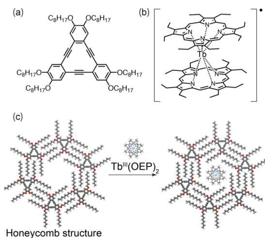
Scheme 1. Chemical structure of (a) DBA-OC8 and (b) radical form \text{Tb}^{\text{III}}(\text{oep})_2 . (c)
