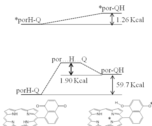
Figure 2. Energy level diagram before ( \text{porH-Q} ) and after ( \text{por-QH} ) ESIPT and the transition state ( \text{por}\cdots\text{H}\cdots\text{Q} ) of the porphyrin–quinone dyad. Reprinted with permission from ref. 26. Copyright 2012, The Japan Institute of Heterocyclic Chemistry.
