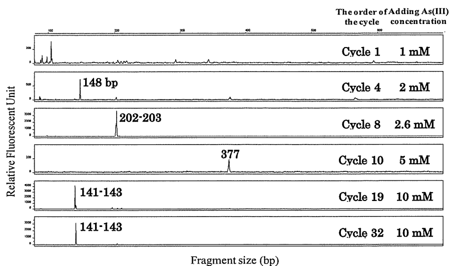
Fig. 2.5 Typical T-RFLP profiles of the enrichment culture during different enrichment cycles.
