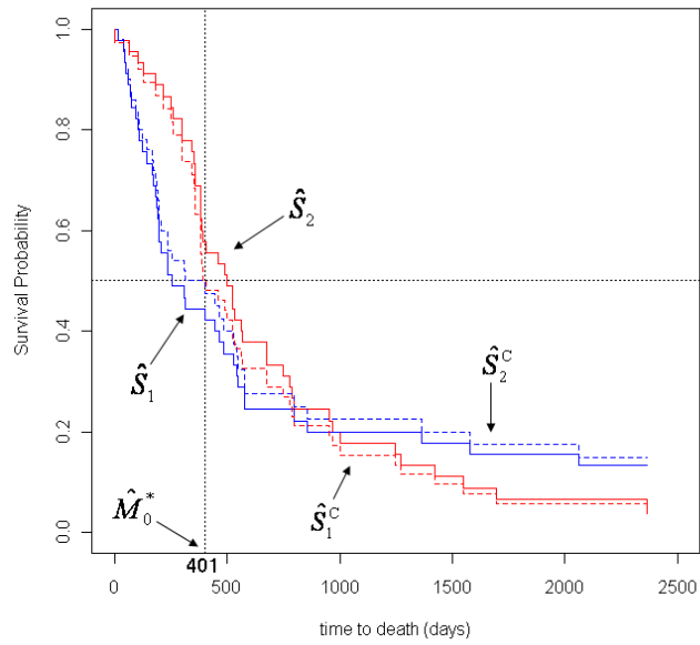
Figure 30: Kaplan-Meier estimates \widehat{S}_j(t) and the constraint Kaplan-Meier estimates \widehat{S}_j^c(t) , j = 1, 2 (dotted line) for gastric cancer data
