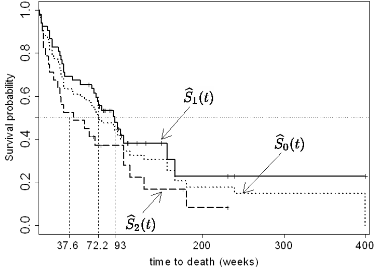
Figure 26: Kaplan-Meier estimates \hat{S}_1(t) (Aneuploid Tumors: solid line) and \hat{S}_2(t) (Diploid Tumors: dashed line), and weighted Kaplan-Meier estimate \hat{S}_0(t) (dotted line)
