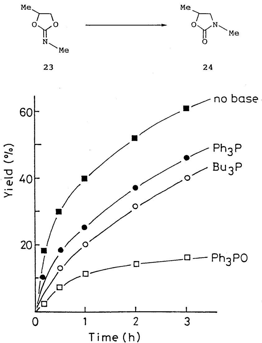
Figure 1. The Isomerization of 23 to 24.
