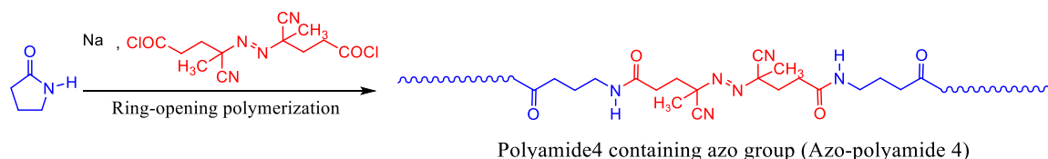
Scheme 6
