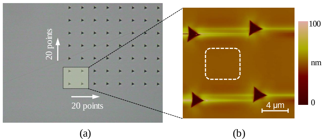
Figure 5.3 Fiducial indents on the SiC surface. (a) CCD image of the fiducial indents formed on the surface of 4H-SiC to be polished. b) AFM image of the lower-left corner of the indented area. The change in the step-terrace structure on the polished surface after each polishing experiment was observed in the same area indicated by the dashed square.
