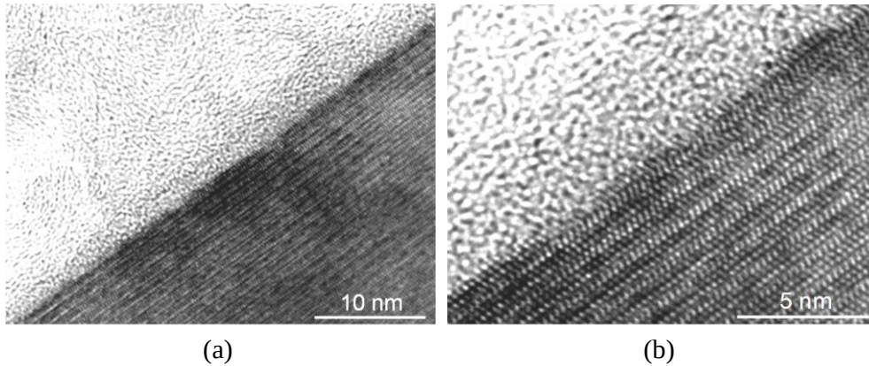
Figure 4.6 XTEM images of CMP-processed SiC.
