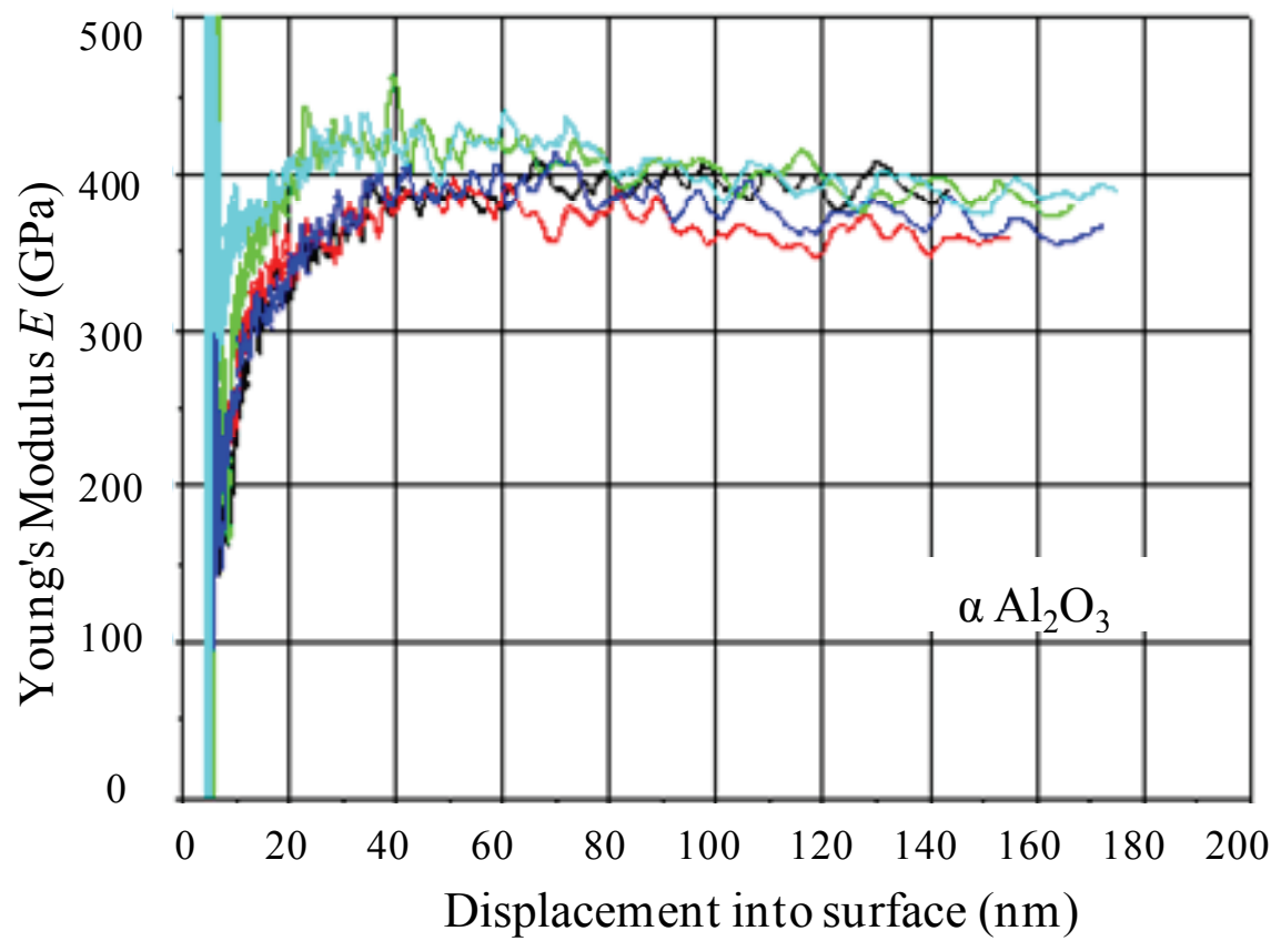
Fig.5-12 Relationship between displacement into surface and Young's modulus of Al 2 O 3 coating by atmospheric plasma spraying (APS) at \alpha -phase point.
