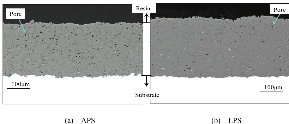
Fig.5-1 Typical macroscopic SEM image of \text{Al}_2\text{O}_3 coatings sprayed by atmospheric plasma spraying (a) APS and by low pressure plasma spraying (b) LPS.
