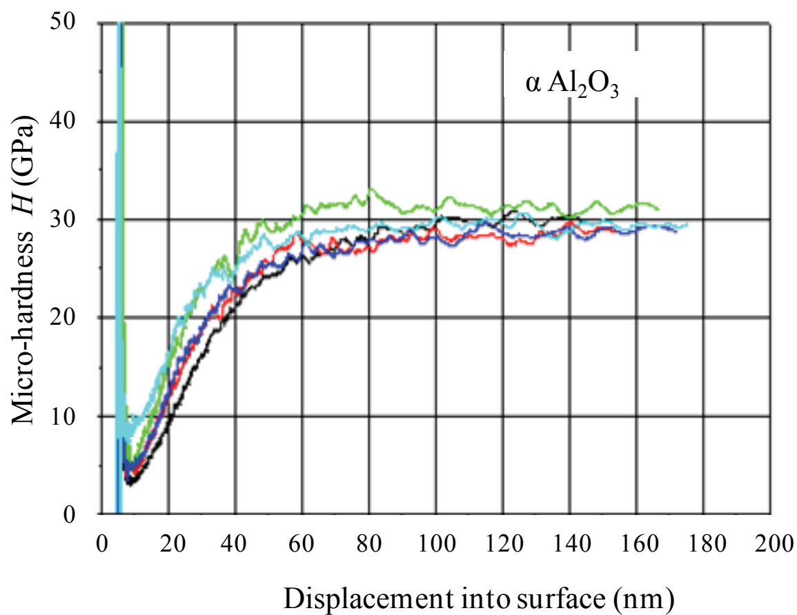
Fig.5-13 Relationship between displacement into surface and micro-hardness of \text{Al}_2\text{O}_3 coating by atmospheric plasma spraying (APS) at \alpha -phase point.
