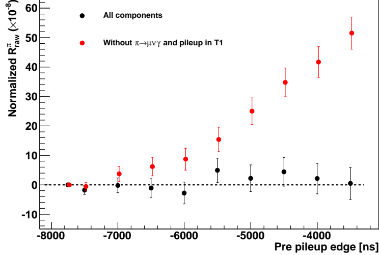
Figure 4.29: Stability plots of the pre pileup cut for the fit using all components (black) and the fit without the functions of \mathcal{G} and \mathcal{F}_2 . The values of R_{\text{raw}}^{\pi} and the statistical errors were normalized to the value at -7750 ns.
