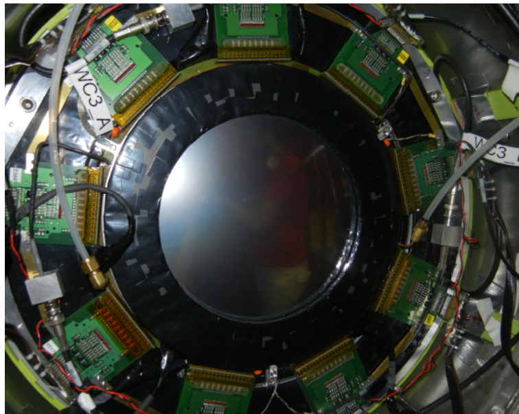
Figure 3.11: Picture of WC3 placed on the flange of the NaI(Tl) enclosure.
