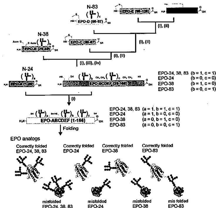
Figure 2. Synthetic strategy of EPO analogs.
