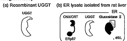
Figure 3. Biological assay with synthetic EPO
