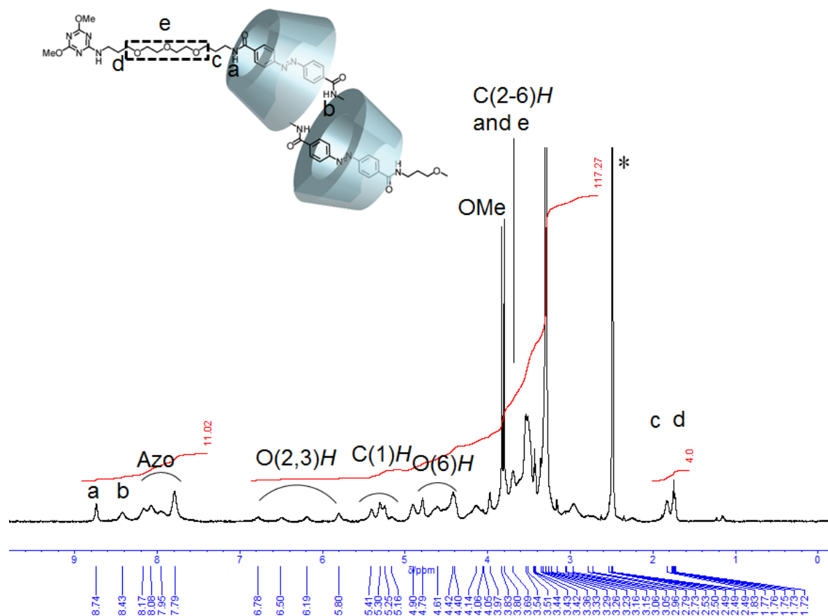
Figure 2-19. 500 MHz ^1\text{H} NMR spectrum of [c2]DMTAzoCD 2 in DMSO- d 6 . "*" denotes the signals due to the solvent used.
