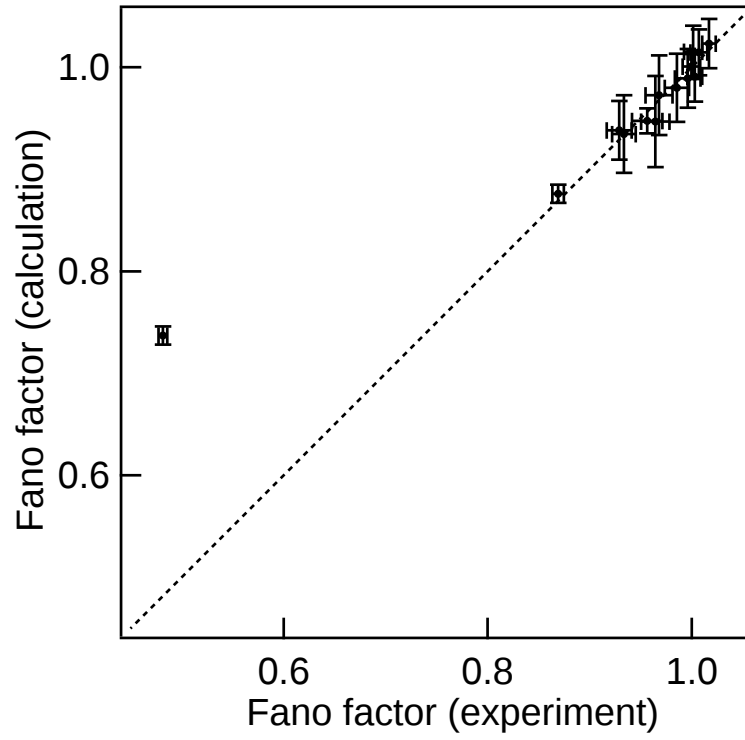
Figure 4.9: Experimental Fano factor ( F_{\text{AP,exp}} ) versus calculated one ( F_{\text{AP,calc}} ). The dashed line represents F_{\text{AP,calc}} = F_{\text{AP,exp}} .
