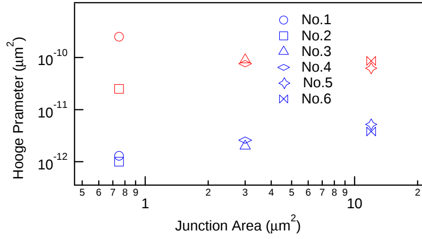
Figure 3.10: Junction area dependence of the Hooe parameter for the P (blue) and AP (red) configuration at 4 K.
