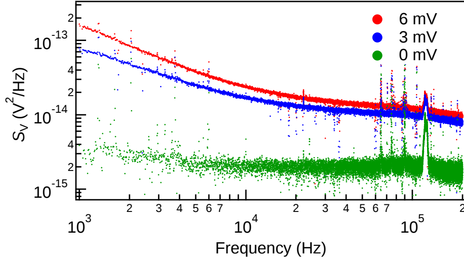
Figure 2.3: Example of the measured voltage noise spectral density in spinel-based MTJs at V_{\text{sd}} = 0, 3, and 6 mV.
