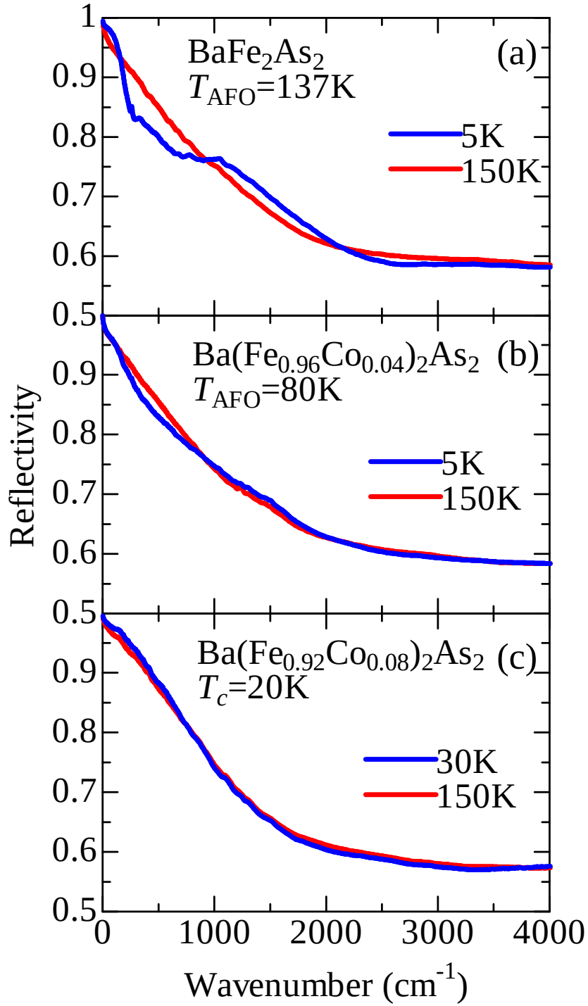
Figure 5.34: (a)-(c) Optical reflectivity of \text{Ba}(\text{Fe}_{1-x}\text{Co}_x)_2\text{As}_2 ( x = 0, 0.04 , and 0.08 ) at 150 K (red) and 5 K (blue).
