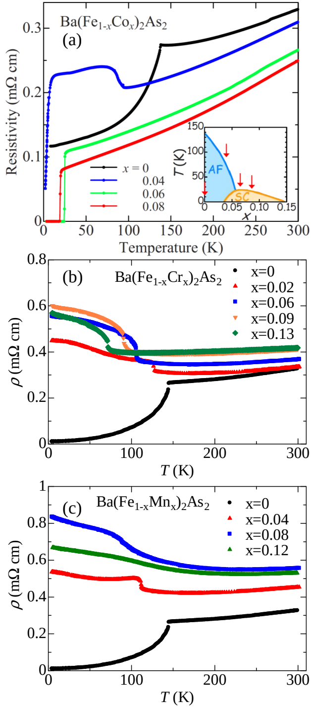
Figure 5.52: Temperature dependence of the in-plane resistivity of \text{Ba(Fe}_{1-x}\text{TM}_x)_2\text{As}_2 (TM=Co, Cr, and Mn) with various x s. (a), (b), and (c) show the results for TM=Co, Cr, and Mn, respectively. The figure of \text{Ba(Fe}_{1-x}\text{Co}_x)_2\text{As}_2 is cited from Ref. [60].
