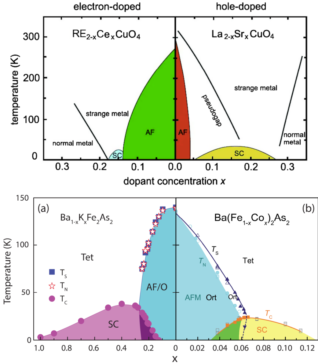
Figure 1.5: The electronic phase diagrams of hole/electron-doped cuprates [20] and those of electron-doped \text{Ba}(\text{Fe}_{1-x}\text{Co}_x)_2\text{As}_2 and hole-doped (\text{Ba}_{1-x}\text{K}_x)\text{Fe}_2\text{As}_2 [8].
