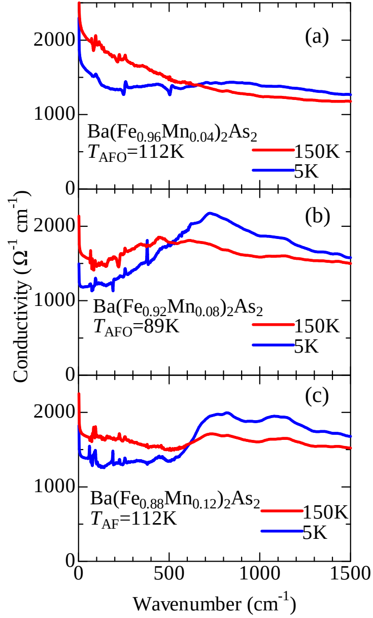
Figure 5.42: (a)-(c) Optical conductivity of \text{Ba}(\text{Fe}_{1-x}\text{Mn}_x)_2\text{As}_2 ( x = 0.04, 0.08 , and 0.12 ) at 150 K and 5 K below 1500 \text{cm}^{-1} .
