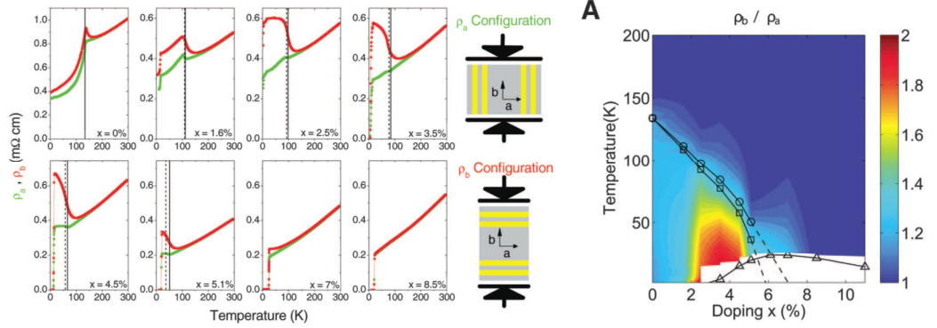
Figure 1.12: (Left panel) Temperature dependence of the in-plane resistivity \rho_a (green) and \rho_b (red) of Ba(Fe 1-x Co x ) 2 As 2 for Co concentrations from x = 0 to 0.085. Solid and dashed vertical lines mark critical temperatures for the structural and magnetic phase transitions T_s and T_{AF} , respectively. (Right panel) Evolution of the in-plane resistivity anisotropy as a function of temperature and doping, expressed in terms of the resistivity ratio \rho_b/\rho_a [45].
