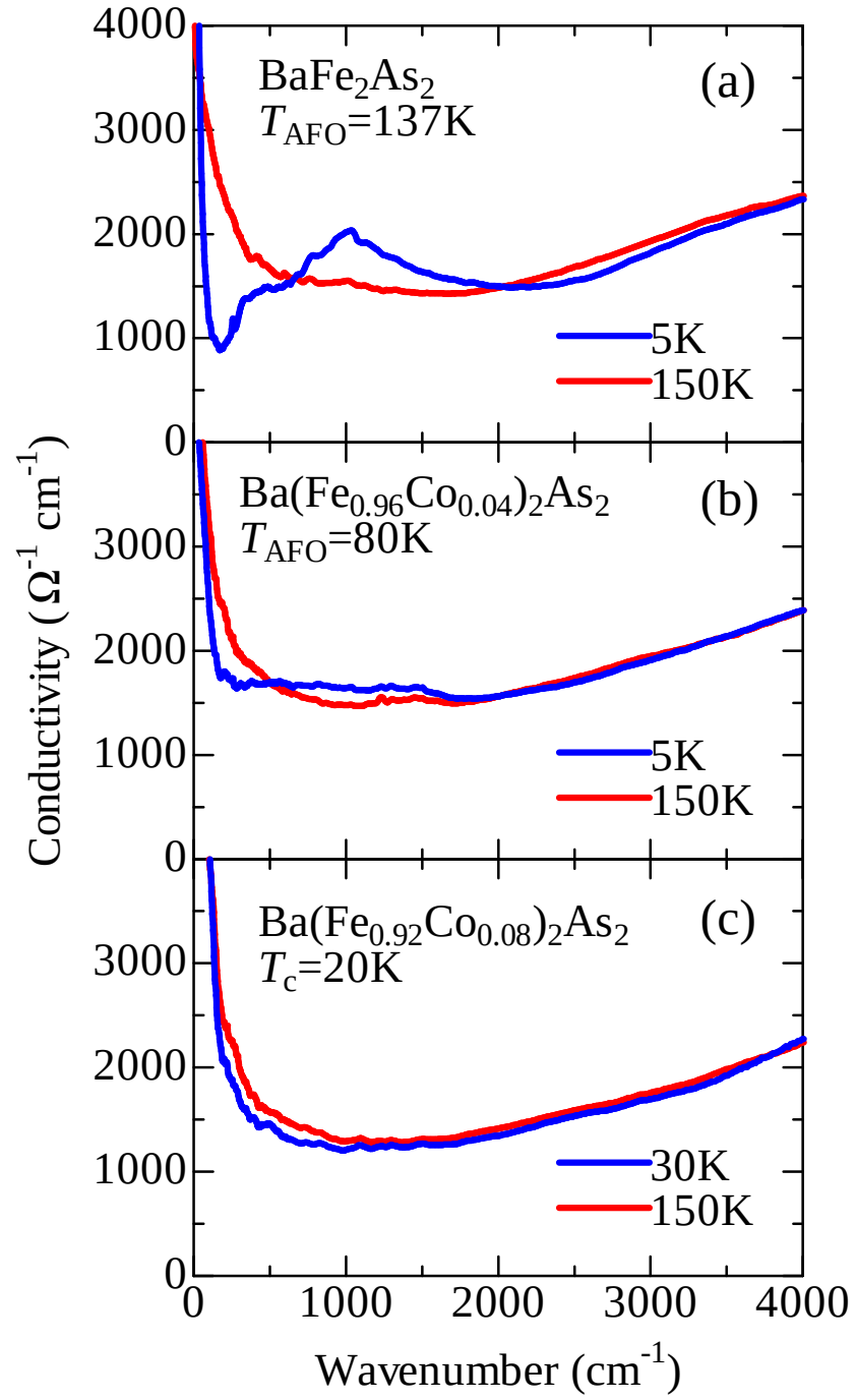
Figure 5.38: (a)-(c) Optical conductivity of \text{Ba}(\text{Fe}_{1-x}\text{Co}_x)_2\text{As}_2 ( x = 0, 0.04 , and 0.08 ) at 150 K (red) and 5 K (blue).
