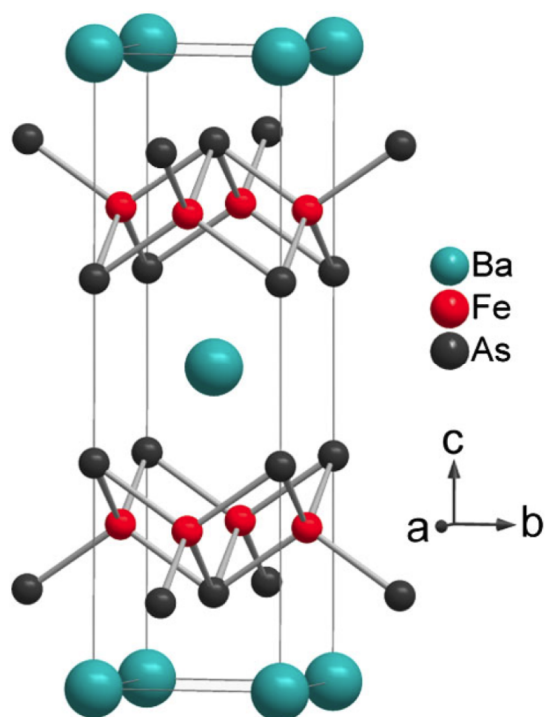
Figure 1.1: The crystal structure of \text{BaFe}_2\text{As}_2 [10].
