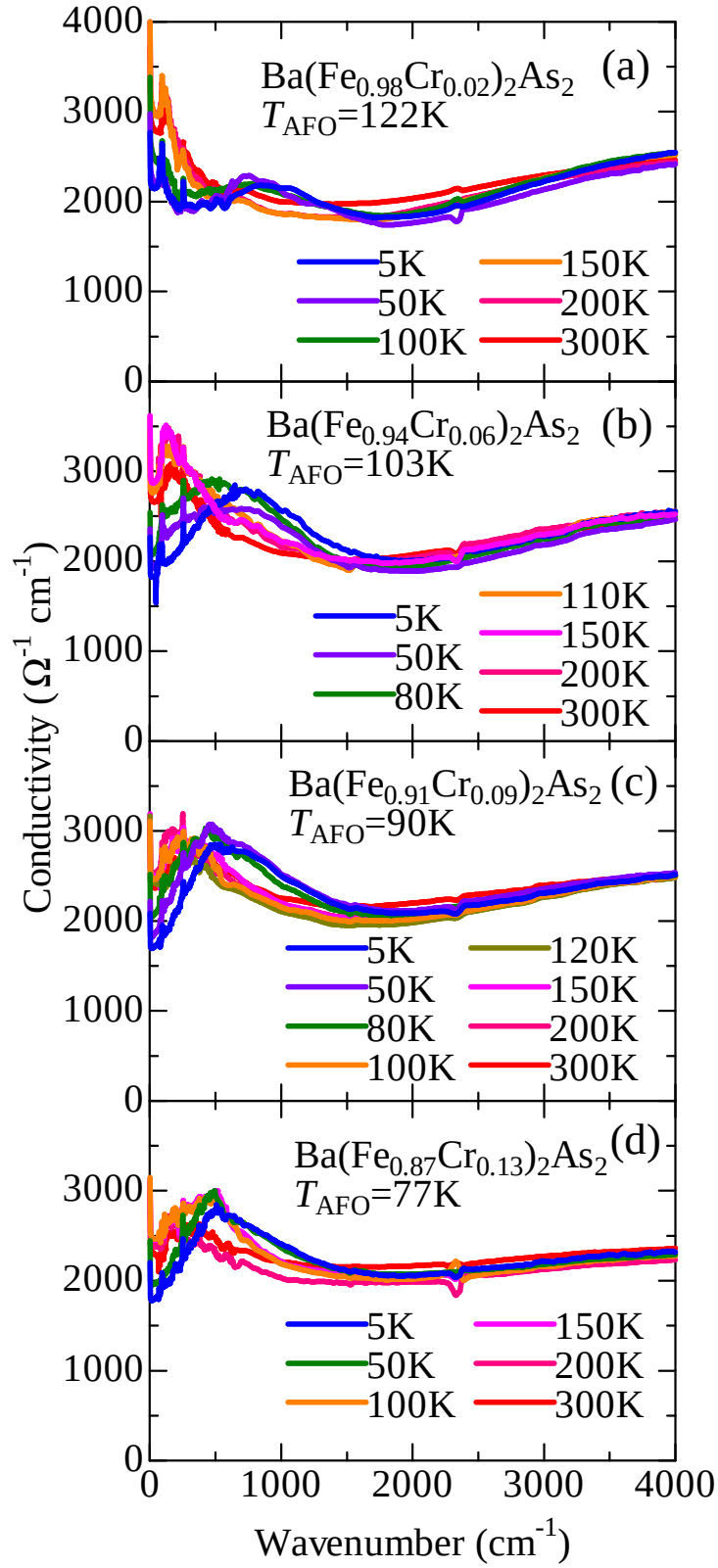
Figure 5.39: (a)-(d) Optical conductivity of \text{Ba}(\text{Fe}_{1-x}\text{Cr}_x)_2\text{As}_2 ( x = 0.02, 0.06, 0.09 , and 0.13 ) at various temperatures.
