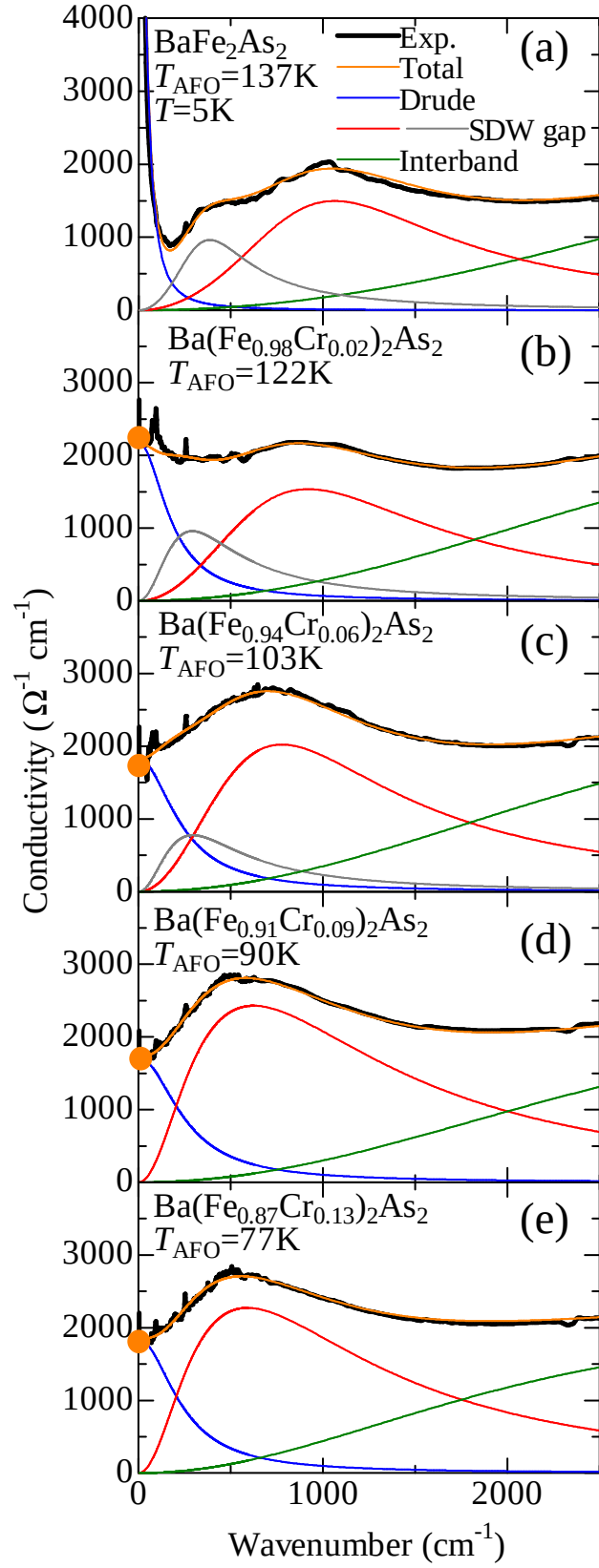
Figure 5.49: The fitting results of \text{Ba}(\text{Fe}_{1-x}\text{Cr}_x)_2\text{As}_2 ( x = 0.02, 0.06, 0.09, \text{ and } 0.13 ) at 5 K. Solid circles indicate the values of the dc ( \omega = 0 ) conductivity for each composition.
