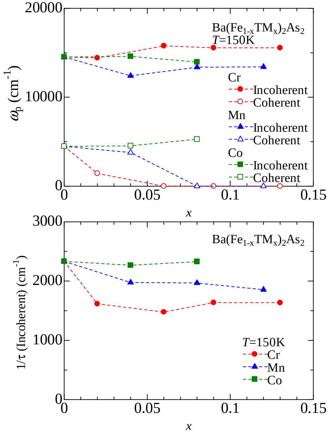
Figure 5.53: (a) Doping dependence of the plasma frequency of coherent (open) and incoherent (closed) component for \text{Ba}(\text{Fe}_{1-x}\text{TM}_x)_2\text{As}_2 [TM=Cr (red circles) and (Mn) (blue triangles), and Co (green squares)] at 150 K, respectively. (b) Doping dependence of scattering rate of incoherent component for \text{Ba}(\text{Fe}_{1-x}\text{TM}_x)_2\text{As}_2 [TM=Cr (red circles) and Mn (blue triangles), and Co (green squares), respectively. These are the fitting results of “one Drude” fitting method.
