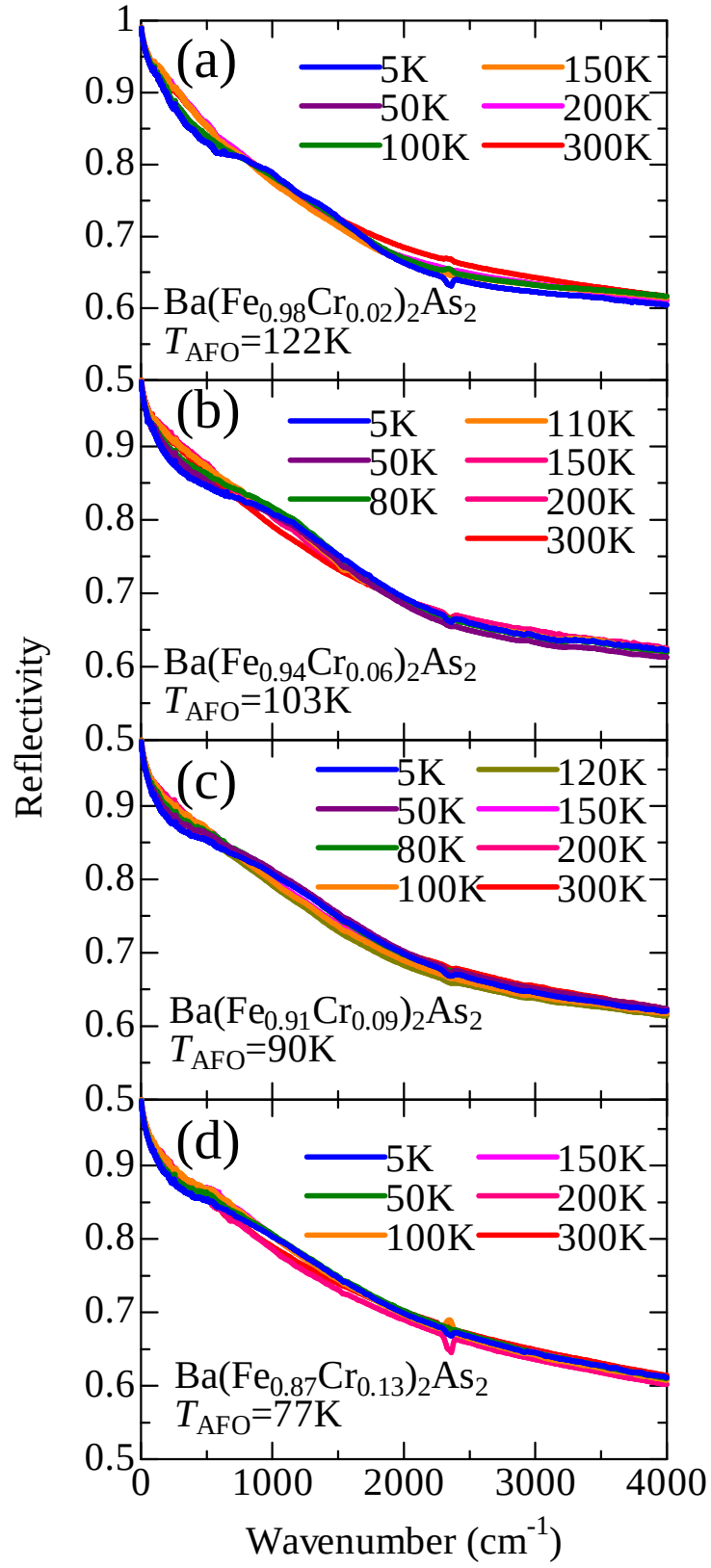
Figure 5.35: (a)-(d) Optical reflectivity of \text{Ba}(\text{Fe}_{1-x}\text{Cr}_x)_2\text{As}_2 ( x = 0.02, 0.06, 0.09, \text{ and } 0.13 ) at various temperatures.
