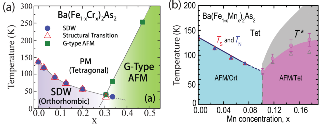
Figure 1.7: The structural and magnetic phase diagrams of Cr and Mn-substituted \text{BaFe}_2\text{As}_2 [24, 25].
