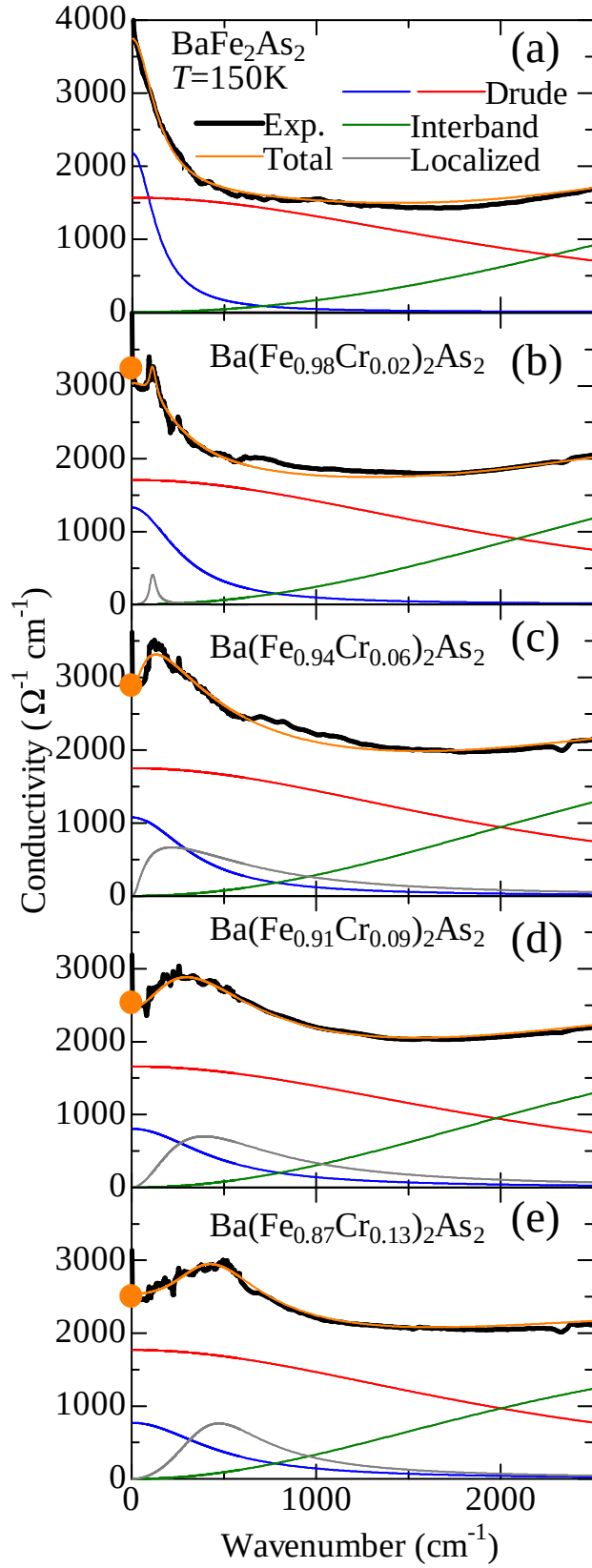
Figure 5.46: The fitting results of \text{Ba}(\text{Fe}_{1-x}\text{Cr}_x)_2\text{As}_2 at 150 K. Solid circles indicate the values of the dc ( \omega = 0 ) conductivity for each composition. For the incoherent component of Cr-doped systems, the similar fitting parameters to that of the parent compound are used.
