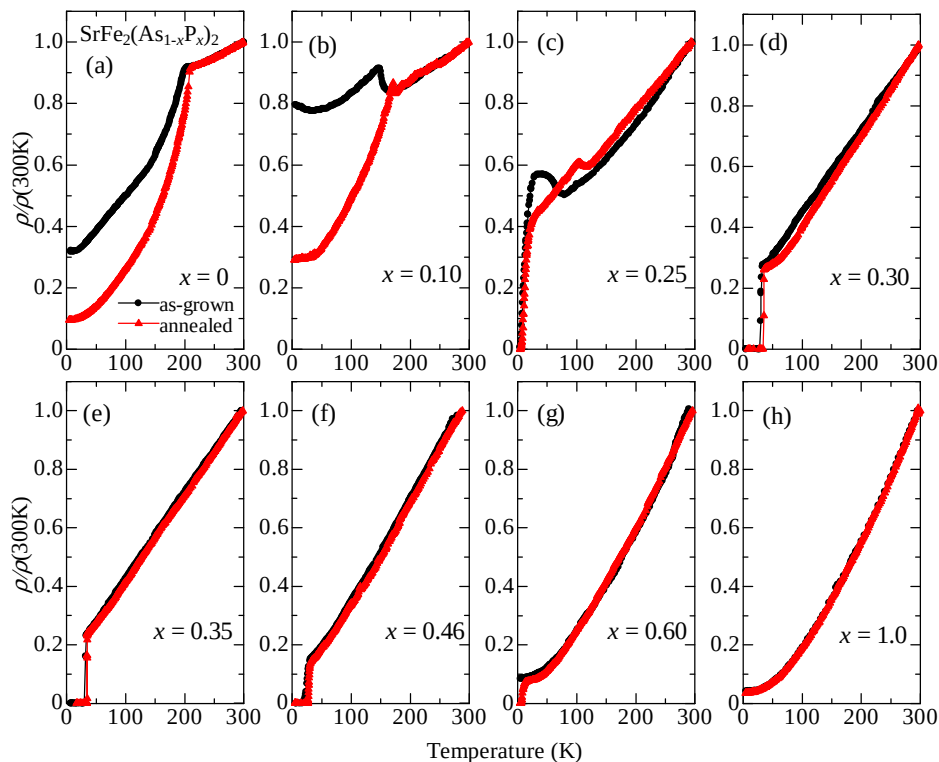
Figure 3.17: (a)-(h) Temperature dependence of the resistivity before and after annealing for 0 \leq x \leq 1 . The absolute value of \rho(300\text{ K}) decreases from 0.29\text{ m}\Omega\cdot\text{cm} for x = 0 to 0.22 for x = 0.35 and 0.030 for x = 1 . The solid lines are visual guides.
