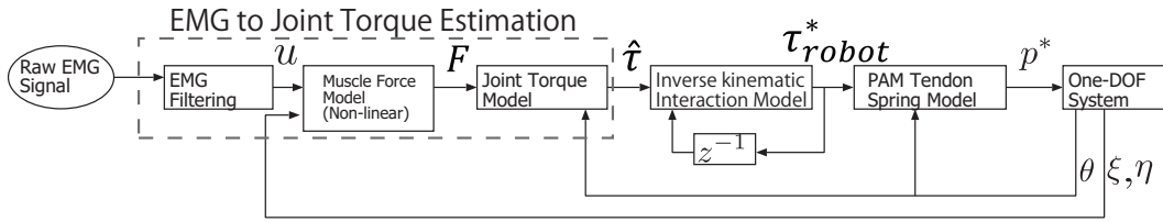
Figure 5.19: Feedback process considering Human-robot interaction
