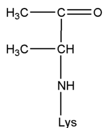
Carboxyethyllysine (CEL)
