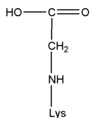
Carboxymethyllysine (CML)
