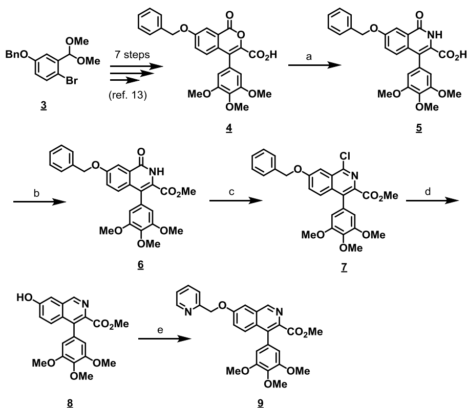
Scheme 1-1. Reagents and conditions: (a) \text{NH}_3\text{-MeOH} , r.t.; (b) \text{SOCl}_2 , MeOH, reflux (84% from 4 ); (c) \text{POCl}_3 , reflux (quant.); (d) \text{Pd-C} , \text{H}_2 , \text{Et}_3\text{N} , EtOH, r.t.; (e) 2-chloromethylpyridine, \text{K}_2\text{CO}_3 , DMF, 50^\circ\text{C} (53% from 7 ).
