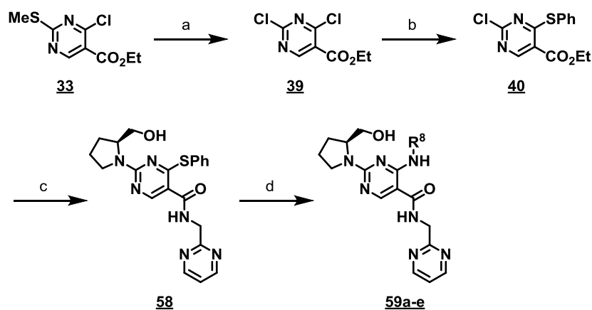
Scheme 2-8. Reagents and conditions: (a) \text{SO}_2\text{Cl}_2 , 50 °C (quant.); (b) Ph-SH, \text{K}_2\text{CO}_3 , toluene, r.t. (80%); (c) (i) ( S )-prolinol, \text{Et}_3\text{N} , THF, r.t., (ii) NaOH aq., EtOH, r.t., (iii) 2-aminomethylpyrimidine, EDC, HOBT, DMF, r.t. (55%), (d) (i) m CPBA, \text{CHCl}_3 , 0 °C, (ii) amine ( \text{R}^8\text{-NH}_2 ), \text{Et}_3\text{N} , \text{CHCl}_3 , reflux ( 59a 75% or r.t. ( 59b 20%, 59c 83%, 59d 63%, 59e 89%, ).
