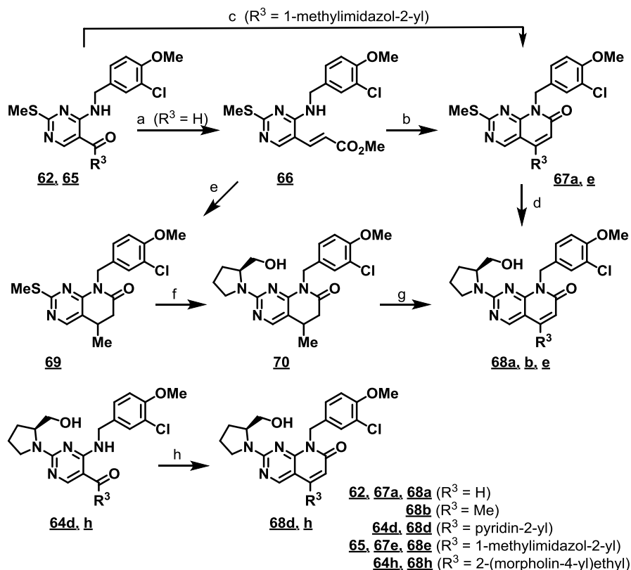
Scheme 3-4. Reagents and conditions: (a) (\text{MeO})_2\text{P}(\text{O})\text{CH}_2\text{CO}_2\text{Me} , NaH, THF, r.t. (59%); (b) NaH, MeOH, r.t. ( 65a 96%); (c) (\text{MeO})_2\text{P}(\text{O})\text{CH}_2\text{CO}_2\text{Me} , NaH, toluene 100 °C ( 65e 13%); (d) (i) m CPBA, \text{CHCl}_3 , 0 °C, (ii) ( S )-prolinol, \text{Et}_3\text{N} , \text{CHCl}_3 , 0 °C ( 66a 77%, 66e 96%); (e) MeLi, CuCN, \text{EtO}_2 , THF, 0 °C, (67%); (f) (i) m CPBA, \text{CHCl}_3 , 0 °C, (ii) ( S )-prolinol, \text{Et}_3\text{N} , \text{CHCl}_3 , 60 °C (75%); (g) DDQ, dioxane, 60 °C ( 66b 30%); (h) (\text{MeO})_2\text{P}(\text{O})\text{CH}_2\text{CO}_2\text{Me} , NaH, toluene, 100 °C ( 66d 17%) or \text{TMSCH}_2\text{CO}_2\text{Me} , dicyclohexylamine, n -BuLi, THF, r.t. ( 66h 8%).
