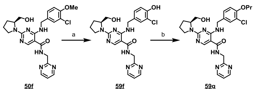
Scheme 2-9. Reagents and conditions: (a) \text{BBr}_3 , \text{CH}_2\text{Cl}_2 , 0 °C (43%); (b) Pr-I, \text{K}_2\text{CO}_3 , DMF, r.t. (94%).
