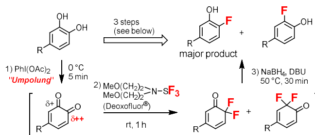
Scheme 1. Deoxyfluorination of catechol derivatives
