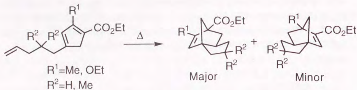
Scheme 1.7
