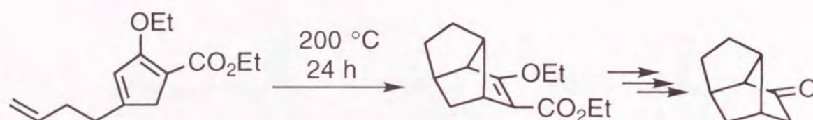
Scheme 1.8
