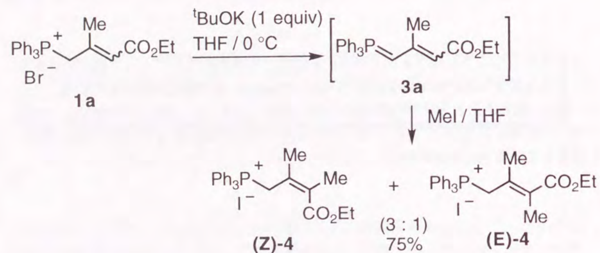
Scheme 2.2
