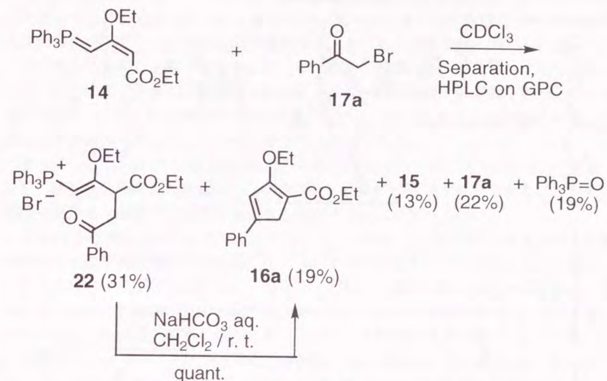
Scheme 3.4
