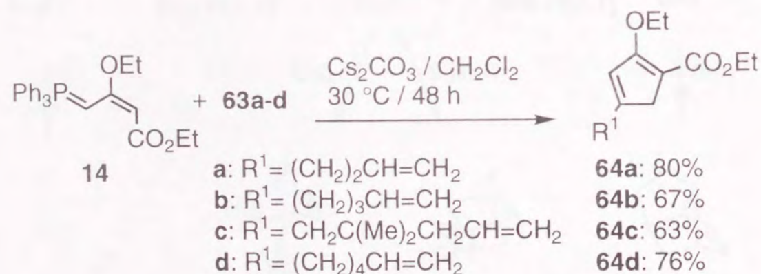
Scheme 5.2
