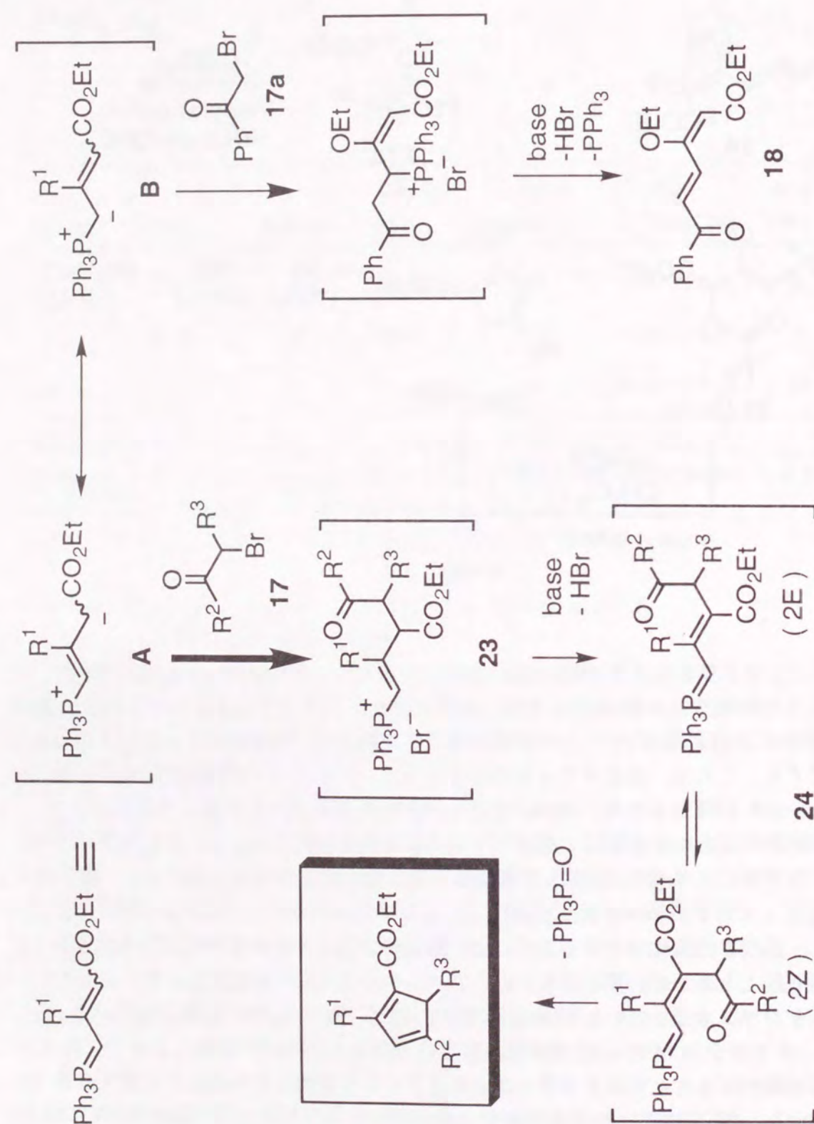
Scheme 3.5
