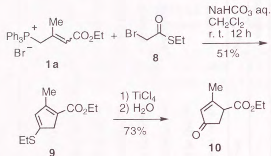
Scheme 2.4
