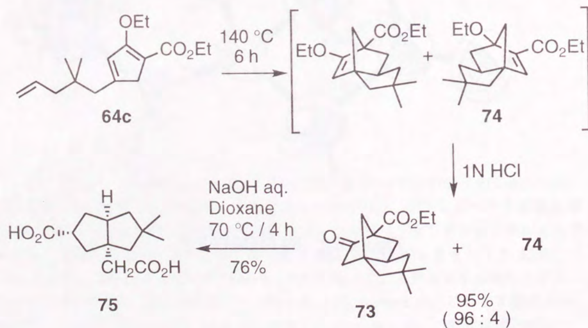
Scheme 5.7
