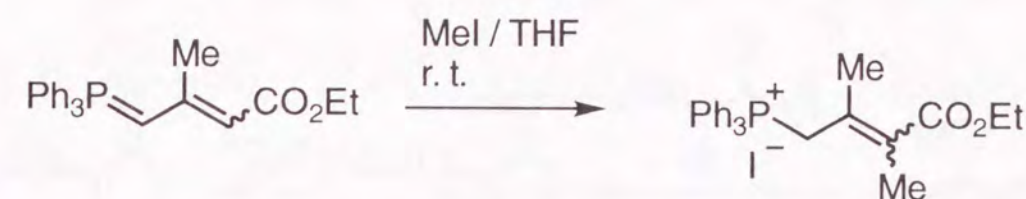
Scheme 1.1
