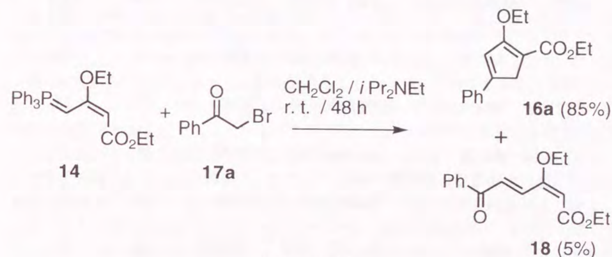
Scheme 3.2
