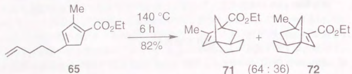
Scheme 5.6
