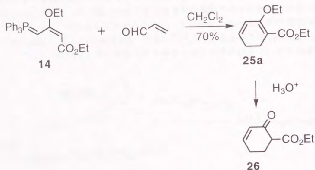
Scheme 4.1
