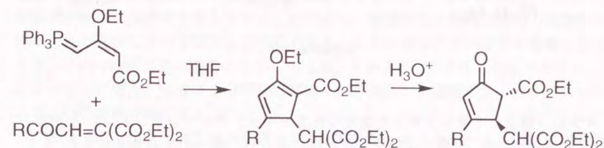
Scheme 1.5
